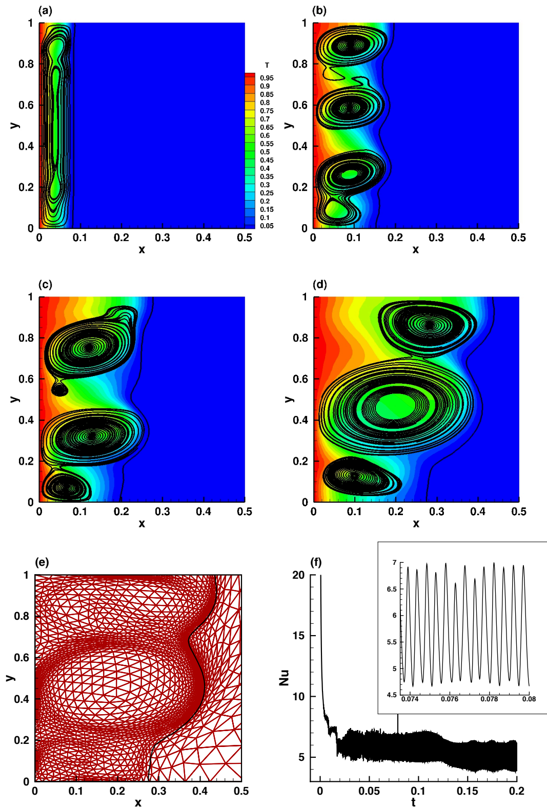
Figure 5.9: Melting of Gallium: temperature field, streamlines, and melting front for dimensionless time instants (panels a to d): t = 0.0015 , 0.006 , 0.01 , and 0.019 . Adapted mesh corresponding to t = 0.019 (e). Time evolution of the Nusselt number (f). For a better view of the convection cells, a ratio 2 : 1 was used for the axes.
