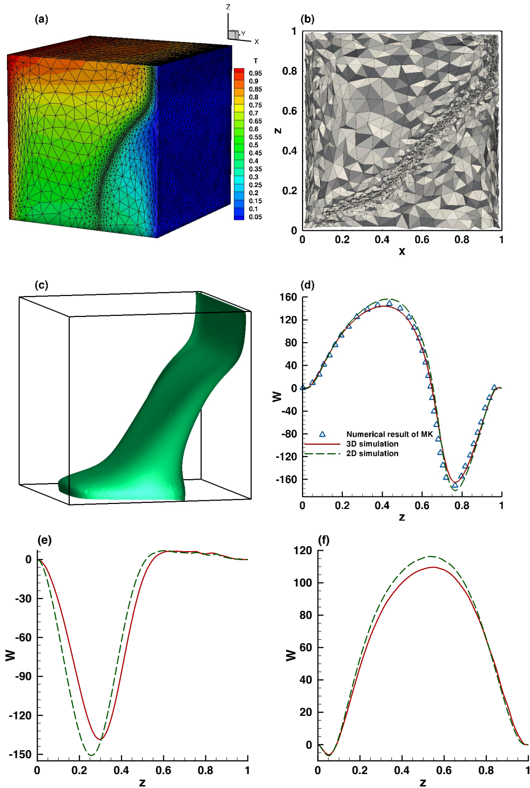
Figure 8.2: Natural convection of water in a cube-shaped cavity. (a) Temperature distribution and adapted mesh. (b) Zoom of the 3D adapted mesh at mid-plane. (c) Iso-surface \theta = \theta_m . Comparison of the profile of the vertical velocity along the z -direction with the numerical benchmark by Kowalewski and Rebow (1999) at the mid-plane ( y = 0.5 ) and x = 0.93 (d); x = 0.1 (e); x = 0.5 (f).
