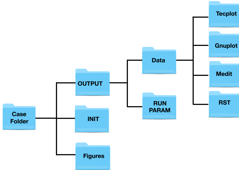
Figure 3.2: Structure of each Test-case folder.
