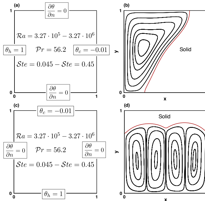
Figure 6.1: Comparison between lateral (LM) and basal melting (BM). Sketch of the computational domain and boundary conditions for LM (top) and BM (bottom) cases. Streamlines (panels b and d) and solid-liquid interfaces (solid red lines).
