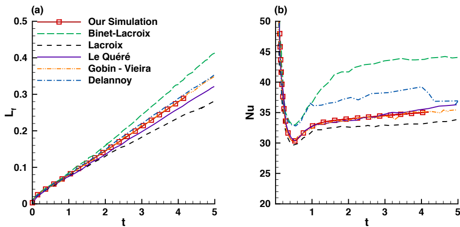
Figure 5.8: Benchmark #3 : \mathcal{Ra} = 2 \cdot 10^8 , \mathcal{Pr} = 50 and Ste = 0.1 . Time evolution of the liquid fraction (a) and the Nusselt number (b). Comparison with five simulations presented by Bertrand et al. (1999).
