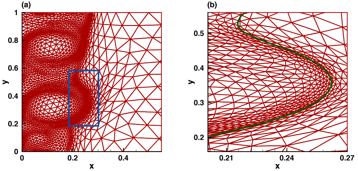
Figure 5.3: Adapted mesh during simulation of PCM melting. (a) 4, 211 triangles: the mesh is refined around the melting front \theta = 0 and in the fluid where velocity gradients exist. (b) zoom showing the variation of the mesh size around the temperature isoline \theta = 0 .
