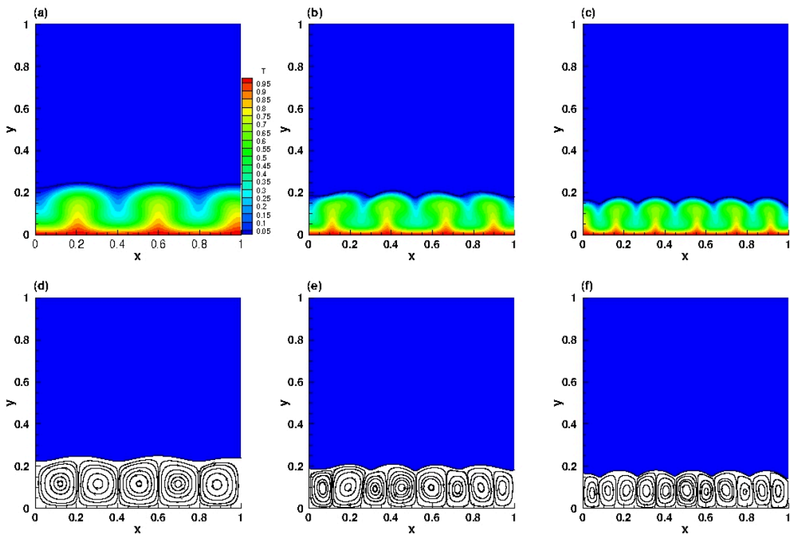
Figure 6.9: Melting of PCM heated from below. Temperature field and solid-liquid interface (top) and streamlines (bottom) in the liquid phase for different Rayleigh numbers (a) \mathcal{Ra} = 3.27 \cdot 10^5 and t = 30 , (b) \mathcal{Ra} = 1.635 \cdot 10^6 and t = 15 , (c) \mathcal{Ra} = 3.27 \cdot 10^6 and t = 10 .
