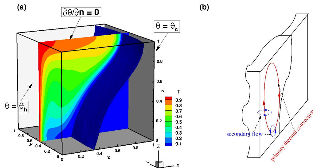
Figure 8.3: Melting of a phase-change material. Problem definition, shape of the solid-liquid interface at t = 78.8 , and temperature distribution in the symmetry plane (a). Scheme of 3D convection flow near the side wall by Nikrityuk (2012) (b).
