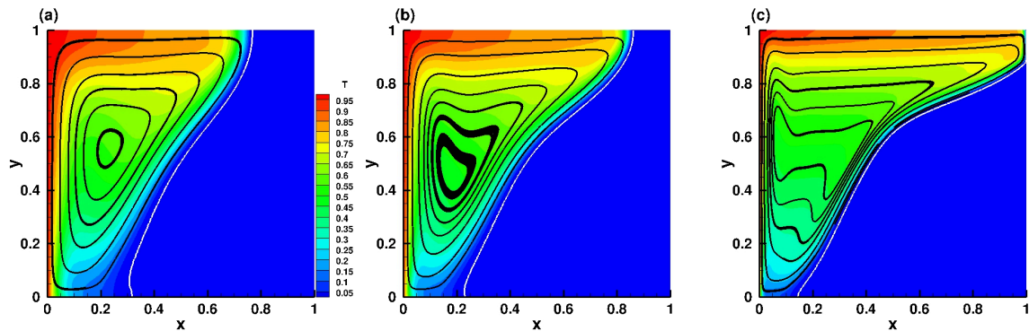
Figure 6.6: PCM melting at L_f = 0.5 . Illustration of the temperature field, streamlines, and melting front for three \mathcal{R}a numbers: (a) \mathcal{R}a = 3.27 \cdot 10^5 , (b) \mathcal{R}a = 1.62 \cdot 10^6 , and (c) \mathcal{R}a = 3.27 \cdot 10^6 . The Pr and Ste numbers are kept constant: Pr = 56.2 and Ste = 0.045 .
