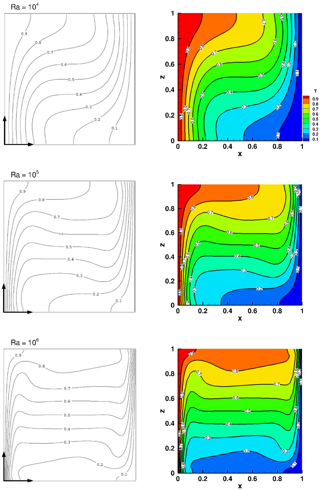
Figure 8.1: Natural convection of air in a 3D differentially heated cavity. Temperature contours at the mid-plane of ( y = 0.5 ). Comparison with the results of Wakashima and Saitoh (2004) (left images).
