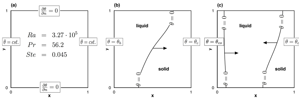
Figure 7.1: Sketch of the computational domain and boundary conditions. General configuration (panel a) with isothermal ( \theta = cst. ) vertical ( x = 0 and x = 1 ) walls and adiabatic ( \partial\theta/\partial n = 0 ) top and bottom walls. Configuration for the melting phase (panel b) with a hot left wall ( \theta = \theta_h > 0 ) and a cold right wall ( \theta = \theta_c < 0 ), followed by a solidification phase (panel c), when the temperature of the left wall is cooled to \theta = \theta_{co} < 0 .
