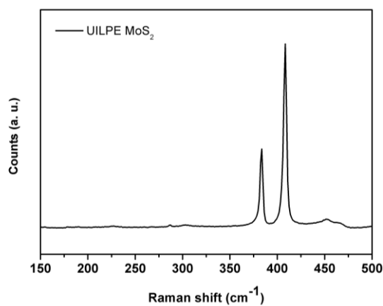
Figure 5. 9. Characteristic Raman spectrum of MoS 2 exfoliated by ultrasounds.
