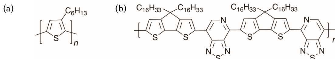
Figure 6. 2. Chemical structure of the two chosen p -type polymeric semiconductors: (a) P3HT and (b) PCDTPT.
