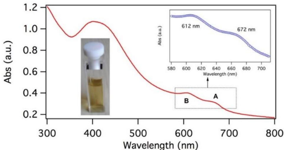
Figure 4. 23. UV-Vis absorption spectrum of MoS 2 nanosheets dispersed in a mixture of H 2 O (70%) and ethanol (30%). The inset shows a magnified view of the spectrum in the region of the A and B exciton peaks.
