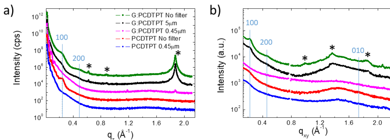
Figure 6. 10. (a) Specular scans and (b) in-plane integrated intensities of GIWAXS images (Figure A I 7) of the PCDTPT and graphene:PCDTPT spin-coated films, shifted for clarity. Bragg peaks coming from graphene solution are labelled by stars.
