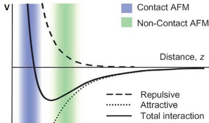
Figure 3. 2. Lennard-Jones potential model (solid line) is the sum of the attractive and repulsive potential (indicated with dotted and dashed lines, respectively). The regions for the different type of AFM measurements are indicated by different colors.
