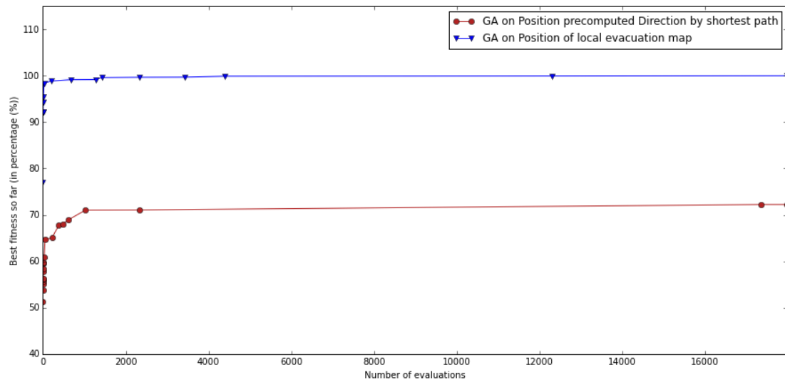
FIGURE 8.5: Comparison between guiding sign optimization and local evacuation map optimization
