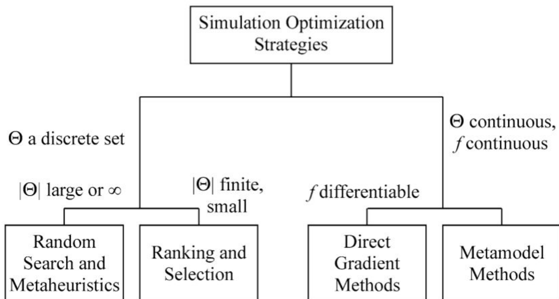
FIGURE 3.2: Simulation optimization strategy depends on the nature of \Theta and f (figure from BARTON and MECKESHEIMER [2006])
