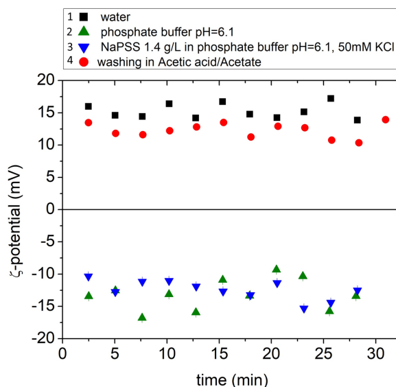
Figure 4.9: \zeta -potential as function of time for nPAAM measured in the following solutions in sequence: water+50mM KCl(black squares), phosphate buffer+50mM KCl (pH=6.1) (green,verse triangles), NaPSS 1.4 g/L in phosphate buffer (pH=6.1)+50mM KCl(blue inverse triangles), Acetic acid/Acetate buffer (pH=4) (red circles).
