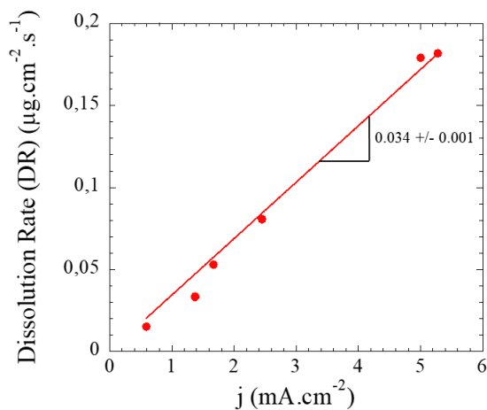
Figure 1.15: Al dissolution rate in electrolyte as a function of current density j . This plot gathers data from different electrolytes (selenic, sulfuric and oxalic in \text{H}_2\text{O} ). The slope is in line with previous works [71].
