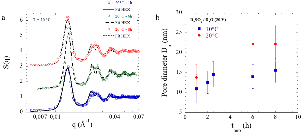
Figure 1.18: (a) Structure factor S(q) derived from the SEM images analysis of nPAAMs prepared in \text{D}_2\text{SO}_4/\text{D}_2\text{O} at 20^\circ\text{C} during different times (1 h, 6 h and 8 h). (b) Evolution with anodization time of pore diameters of nPAAMs prepared in \text{D}_2\text{SO}_4/\text{D}_2\text{O} at 10^\circ\text{C} (blue squares) and 20^\circ\text{C} (red circles).
