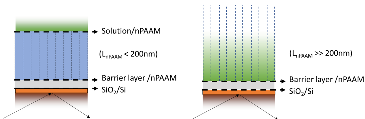
Figure 1.31: Scheme of the probed interfaces by NR depending on the thickness of nPAAM on a Silicon wafer, measured in a mixture of \text{H}_2\text{O}/\text{D}_2\text{O} .
