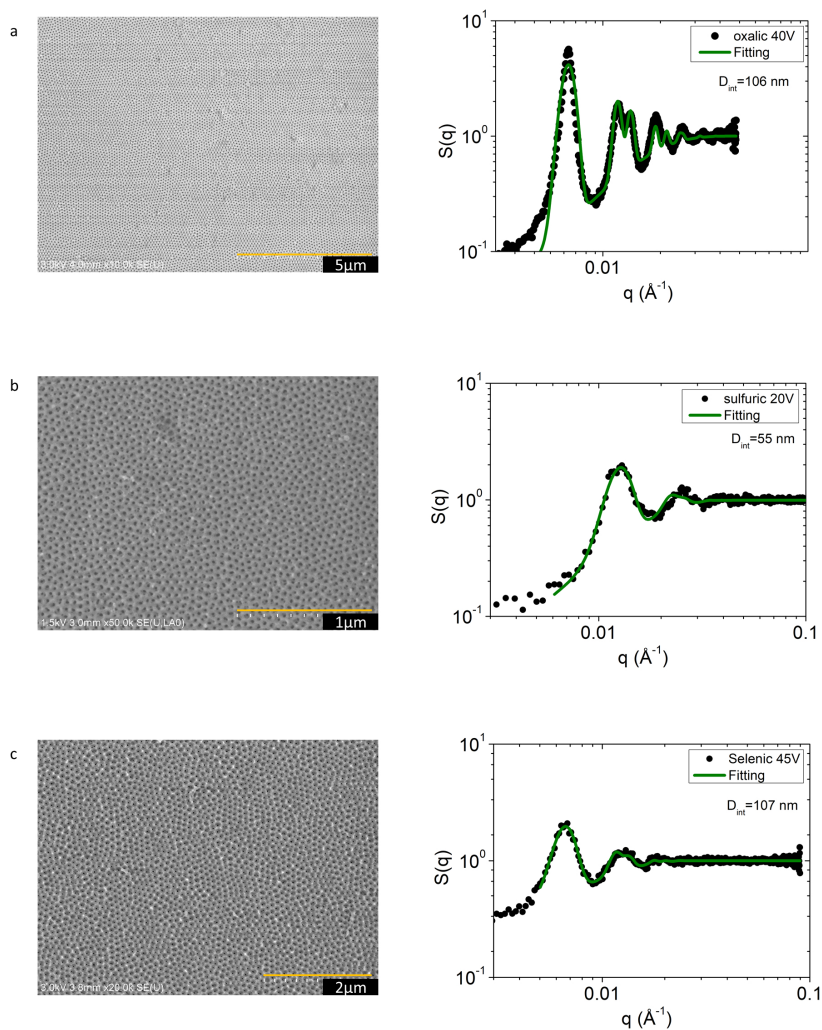
Figure 1.8: SEM images of top surface of nPAAMs prepared by two-step anodization under different conditions. a) Oxalic acid 0.3 M, 40 V, T=18 °C, t=4 hours. b) Sulfuric acid 0.3 M, 20 V, T=10 °C t=8 hours. c) Selenic acid 0.3 M, 45 V, T=0 °C, t=6.5 hours.
