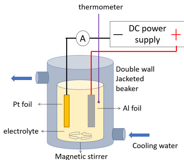
Figure 1.4: Schematic representation of the anodization set-up
