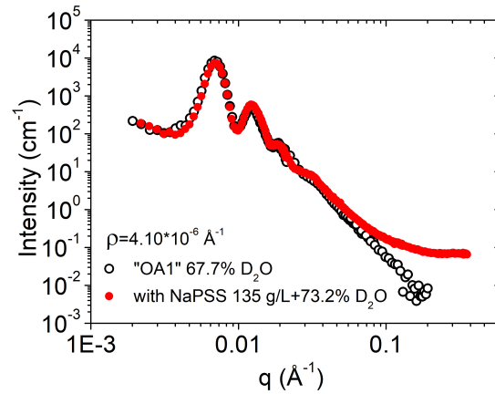
Figure 4.28: Comparison between a SANS spectrum measured in 67.7% D_2O ( \rho_{67.7\% - D_2O} = 4.10 \times 10^{-6} \text{ \AA}^{-1} ) for a bare membrane and the spectrum obtained for a membrane filled with NaPSS at 135 g/L in 73.2% D_2O .
