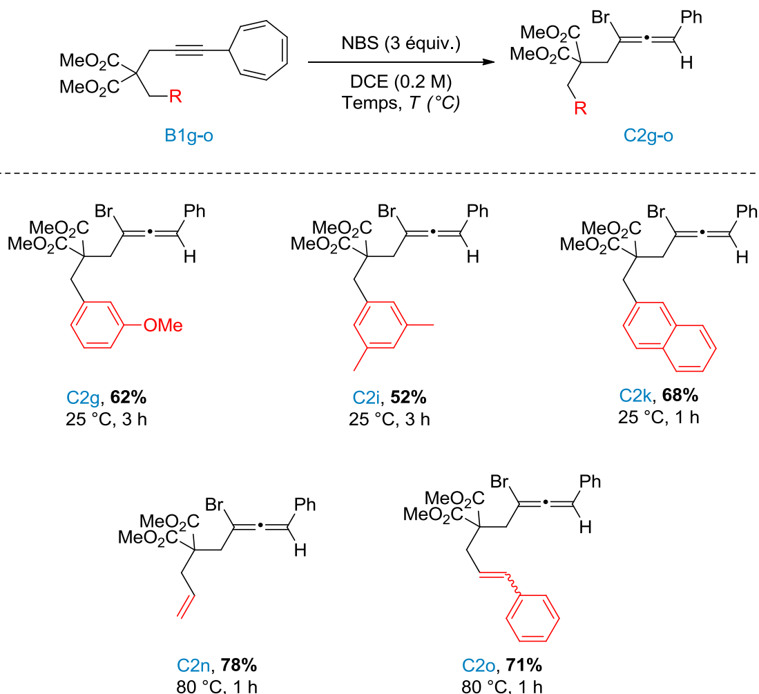
Sch\u00e9ma 144. Bromoall\u00e8nes poss\u00e9dant un lien dim\u00e9thyle malonate
