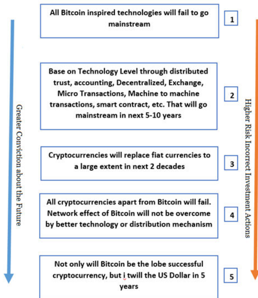
Figure 4.27: Tokenize Everything
