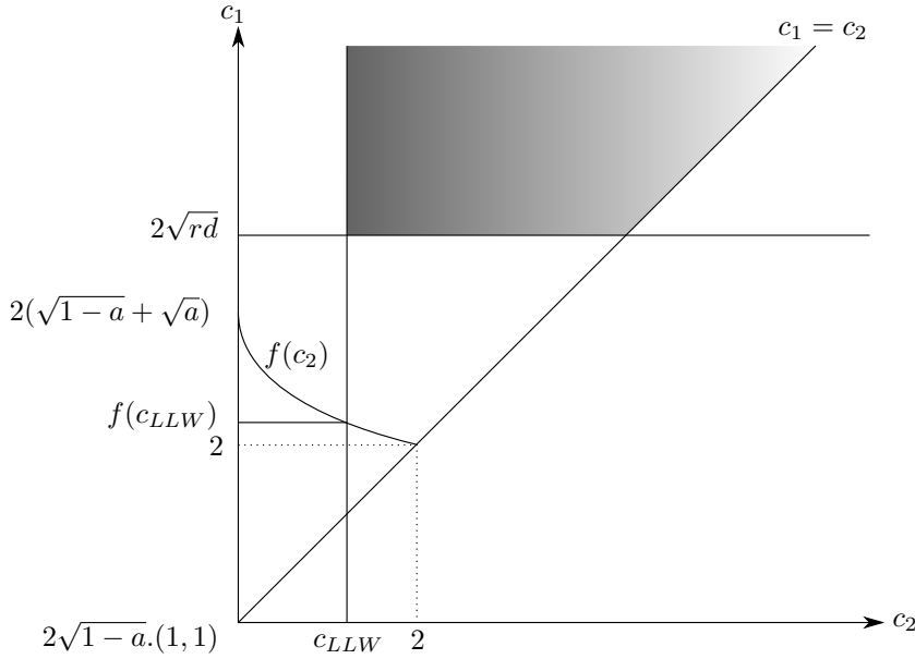
Figure 7.1.2 – Example of set of admissible pairs of speeds (c_1, c_2) : c_{LLW} > 2\sqrt{1-a} , 2\sqrt{rd} > f(c_{LLW}) . In this case Theorem 7.1(3) applies with (c_1, c_2) = (2\sqrt{rd}, c_{LLW}) .
