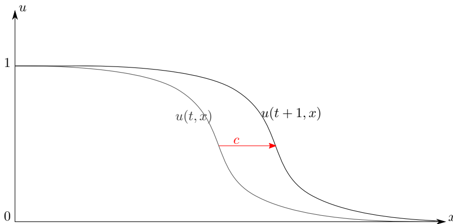
Figure 0.0.2 – A traveling wave for the Fisher–KPP equation
