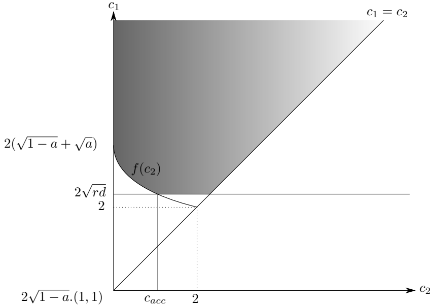
Figure 7.1.1 – Example of set of admissible pairs of speeds (c_1, c_2) : c_{LLW} = 2\sqrt{1-a} , 2\sqrt{rd} < f(c_{LLW}) .
