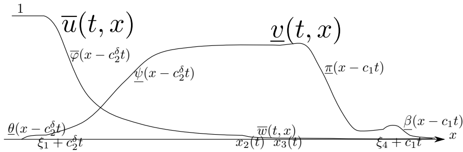
Figure 7.4.2 – Super-solution (\overline{u}_\delta, \overline{v}_\delta) for Theorem 7.3
