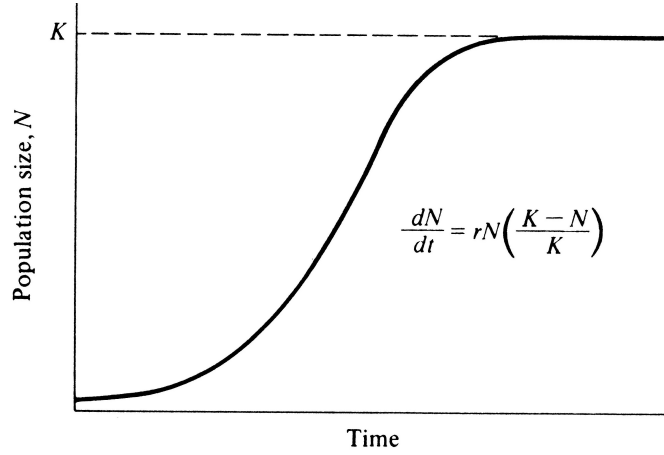
Figure 0.0.1 – Logistic growth curve
