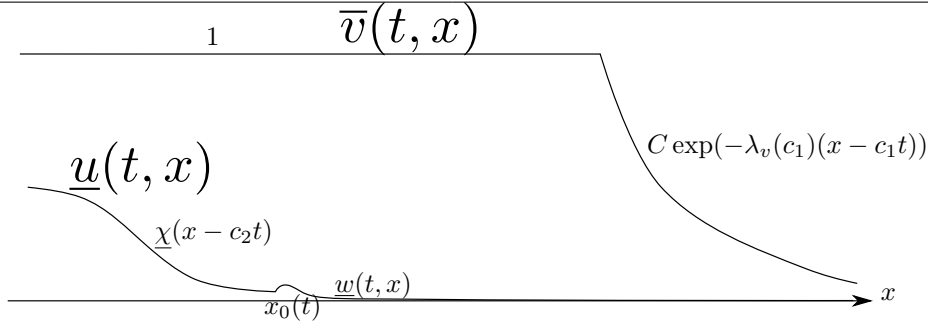
Figure 7.4.1 – Sub-solution (\underline{u}_\delta, \underline{v}_\delta) for Theorem 7.3
