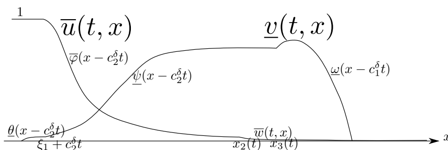
Figure 7.4.3 – Super-solution (\overline{u}_\delta, \underline{v}_\delta) for Theorem 7.1
