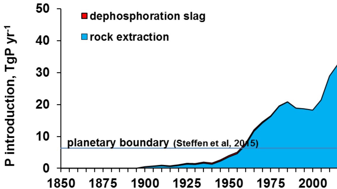
Figure 0.3 Global introduction of phosphorus resulting from fossil P extraction from 1850 to 2015, based on a data compilation from several sources (Jasinski, 2008; IFA, https://www.ifastat.org/databases/plant-nutrition )
