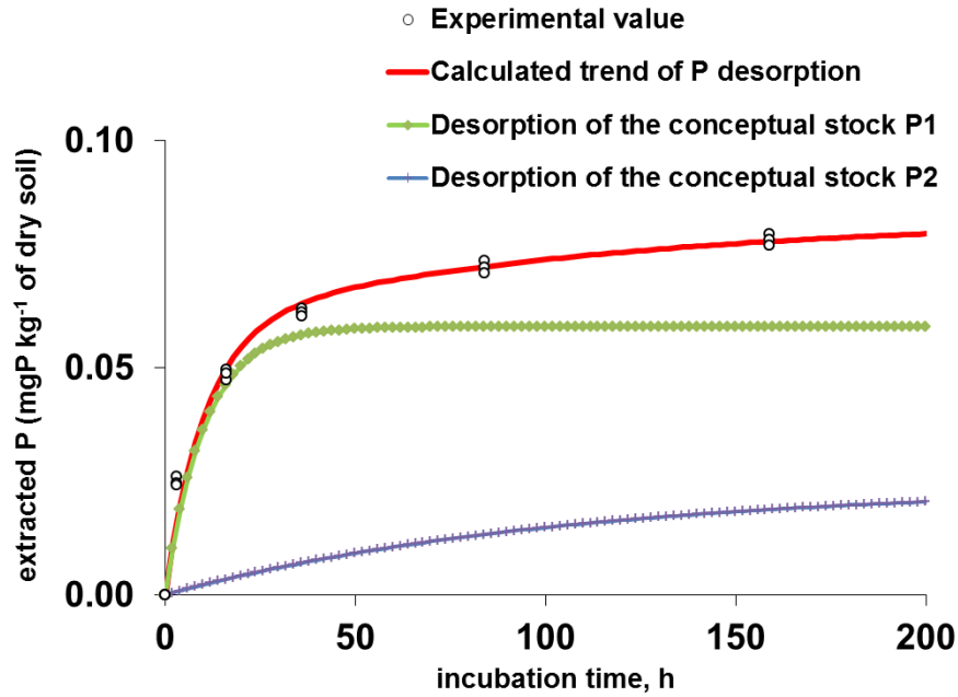
Figure 3.3 Kinetics of phosphate desorption from the soil by anion exchange against hydrogen carbonate. The equation for the desorption curve is: P_1 \times (1 - \exp^{-t/10.4}) + P_2 \times (1 - \exp^{-t/104.2}) , with P_1 the stock of P available within 24 h and P_2 the stock of P available within 240 h. The results from a surface soil from an organic cropping system in Seine-et-Marne are provided as an example.
