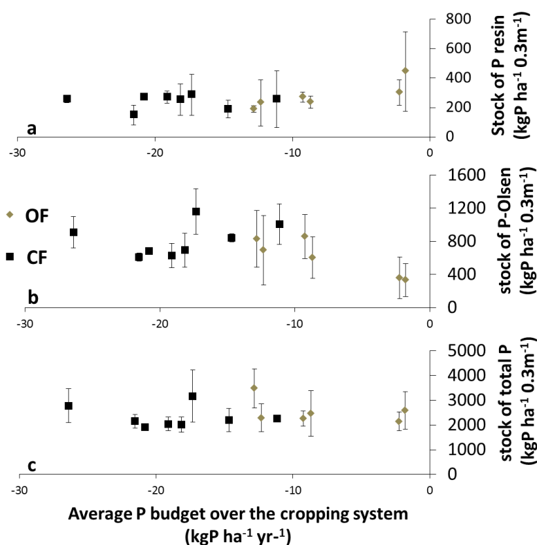
Figure 3.5 Mean P budgets (kgP ha -1 yr -1 ) over the 14 cropping systems on the basis of the studied plots a. stocks of available P within 10 days (kgP ha -1 in the top 30 cm of the soil profile) measured using resin anion exchange; b. stocks of available P (kgP ha -1 in the top 30 cm) measured using the Olsen method; c. stocks of total P (kgP.ha -1 in the top 30 cm) measured using ignition and extraction with HCl 1 M.
