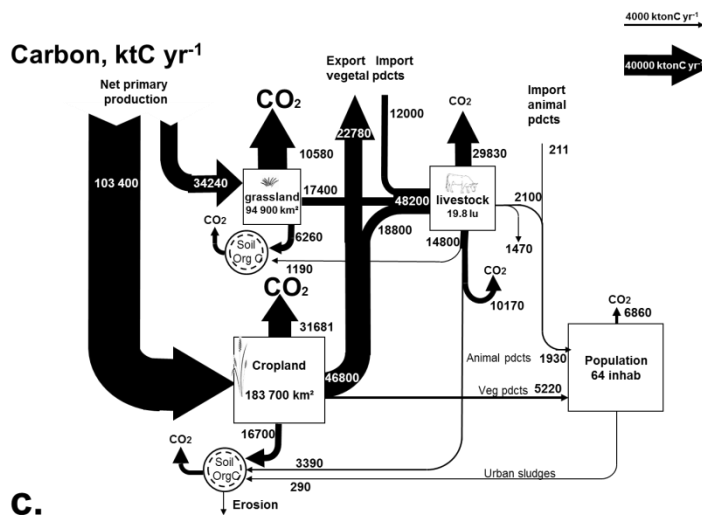
Figure 2.3 Representation of: a. nitrogen; b. phosphorus and; c. carbon fluxes, expressed in kt\ yr^{-1} at the national scale for France in 2006. Squares represent transformation processes occurring in the corresponding environmental compartments. The width of black arrows are proportional to the intensity of the fluxes involved in these processes. Circles represent storage pools of N, P or C in the soil compartments; the dotted circle figures the initial state, the solid circle the final stage.
