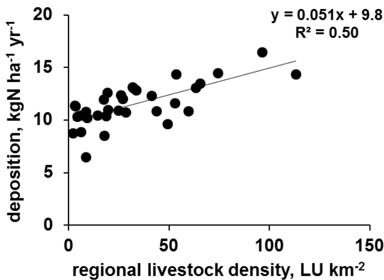
Figure 1.11 Relationship between atmospheric N deposition and livestock density for agricultural regions in France in 2006.
