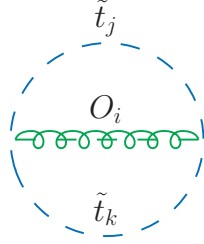
Figure 3.1 – Novel two-loop contribution to the effective potential involving stops and octet scalars.
