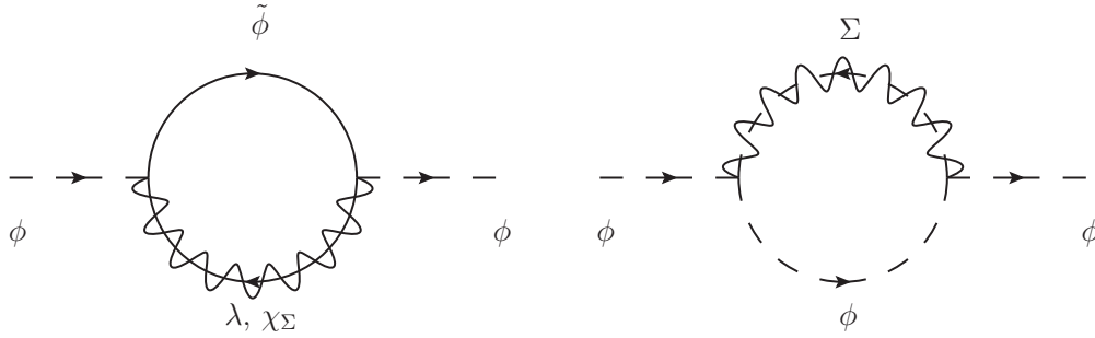
Figure 1.5 – Diagrams contributing to the mass of a scalar \phi : on the left hand side with \tilde{\phi} , i.e. the fermionic superpartner of \phi , and a Dirac gaugino ( \lambda and \chi_\Sigma in terms of Weyl spinors); and on the right hand side with the scalar \phi and the adjoint scalar \Sigma . The logarithmic divergences from both diagrams cancel out when the gauginos only have Dirac masses.
