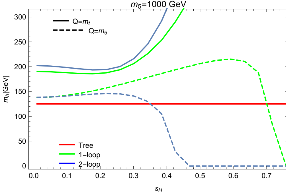
Figure 5.10 – The SM-like Higgs mass at tree-, one- and two-loop level for m_5 = 1 \text{ TeV} and as a function of s_H . The results are shown for two different choices for the renormalisation Q scale, namely Q = m_t and Q = m_5 .
