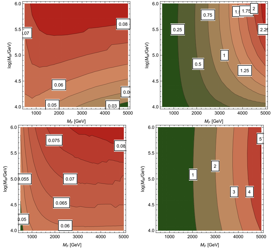
Figure 5.4 – The change in the Higgs mass in GeV due to the two-loop corrections involving the new Yukawa-like interactions \tilde{g}_{(1,2)(u,d)} . On the top, we used \tan\beta = 1 at M_M and on the bottom \tan\beta = 10 . The left plots are with the consistent tadpole solutions, the right ones without.
