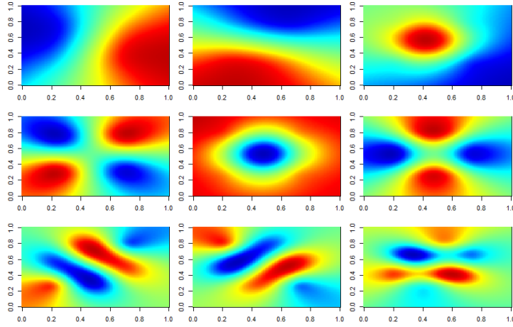
Figure 6.9: Example 6.1, circle with d = 3 parameters, 9 first eigenvectors (left to right and top to bottom) when \phi = \text{signed distance} .
