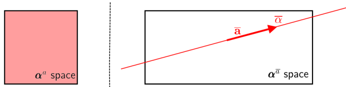
Figure 6.34: EI maximization in \alpha^a complemented by the maximization along \bar{\mathbf{a}} , a random line in the \alpha^{\bar{a}} space.
