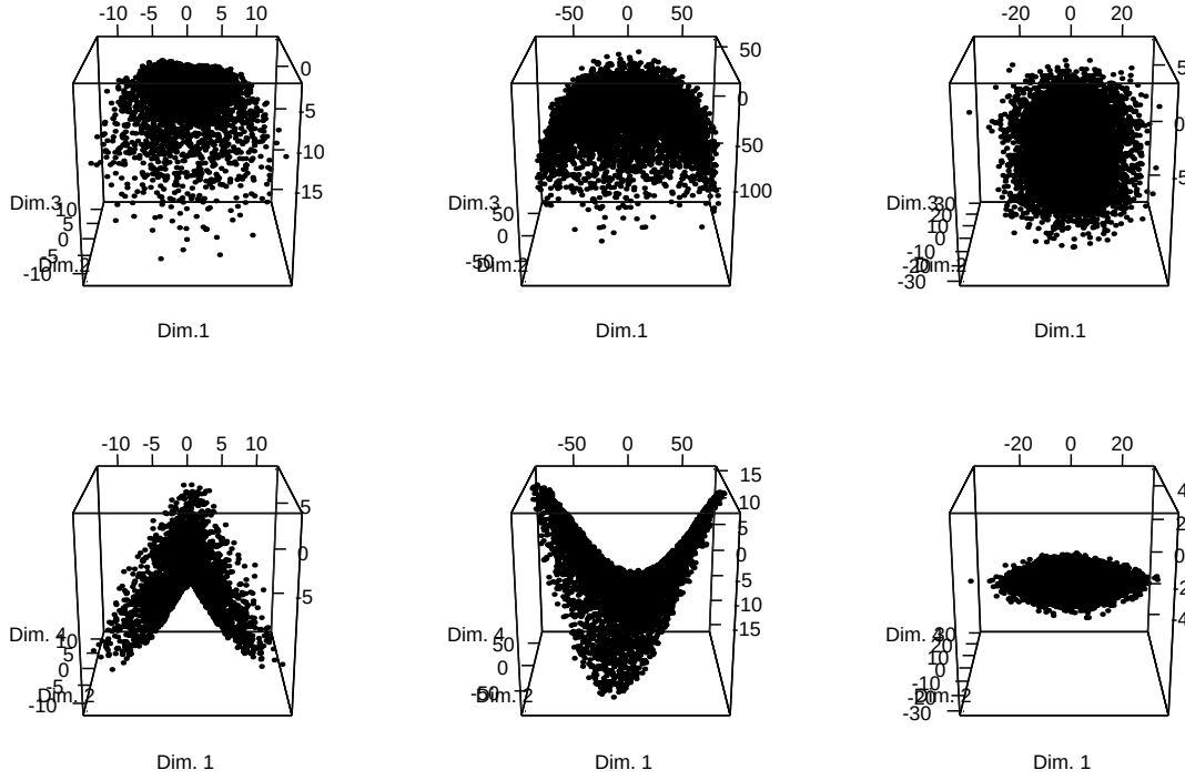
Figure 6.12: Four first eigenvectors of the \alpha^{(i)} 's in the Example 6.2, for the three different shape representations \phi . Left: characteristic function, middle: signed distance to the contour, right: discretization of the contour. The manifolds are shown in the \{\mathbf{v}^1, \mathbf{v}^2, \mathbf{v}^3\} (top), and \{\mathbf{v}^1, \mathbf{v}^2, \mathbf{v}^4\} bases (bottom). As can be seen from the two-dimensional surface in the \{\mathbf{v}^1, \mathbf{v}^2, \mathbf{v}^4\} space when \phi = \mathcal{D} (bottom right), the true dimension (3) is retrieved with the contour discretization. Note also that the associated manifold is convex.
