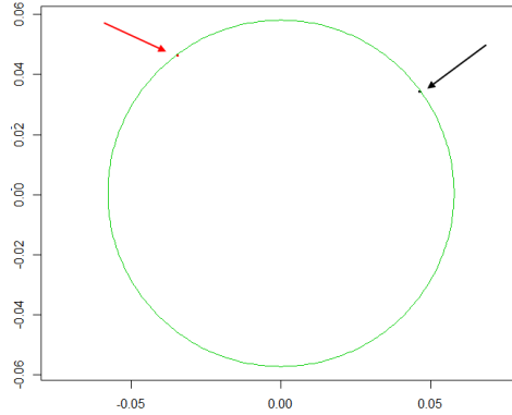
Figure 6.10: Example 6.1, circle with d = 3 parameters, 3 first eigenvectors (black, red, green) when \phi = \text{contour discretization} .
