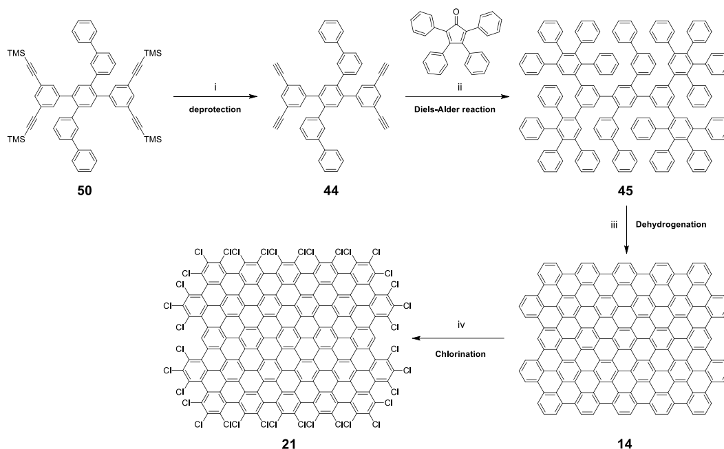
Scheme 3.11: i) TBAF, THF, 0°C, 1h, 94%, ii) o -xylene, 180°C, overnight, 39%; iii) FeCl 3 , MeNO 2 , DCM, R.T., overnight, 73%; iv) AlCl 3 , ICl, CCl 4 , 80°C, 72h, 49%
