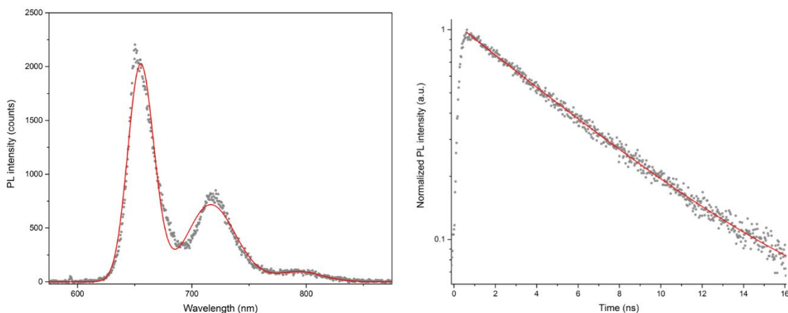
Figure 2.21: PL spectrum and time-resolved PL of a single C96C12 GQD 3
