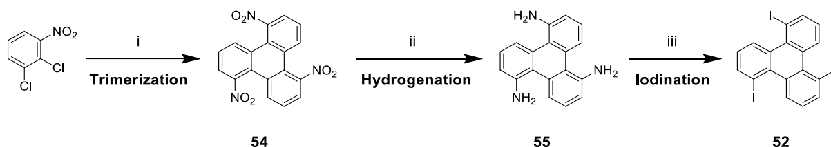
Scheme 4.1: i) Cu, DMF, 160°C, overnight, 34%; ii) Pd/C, EtOAc/EtOH, R.T., overnight, 73%; iii) KI, HCl, NaNO 2 , water, 0°C to R.T., 1h, 26%.
