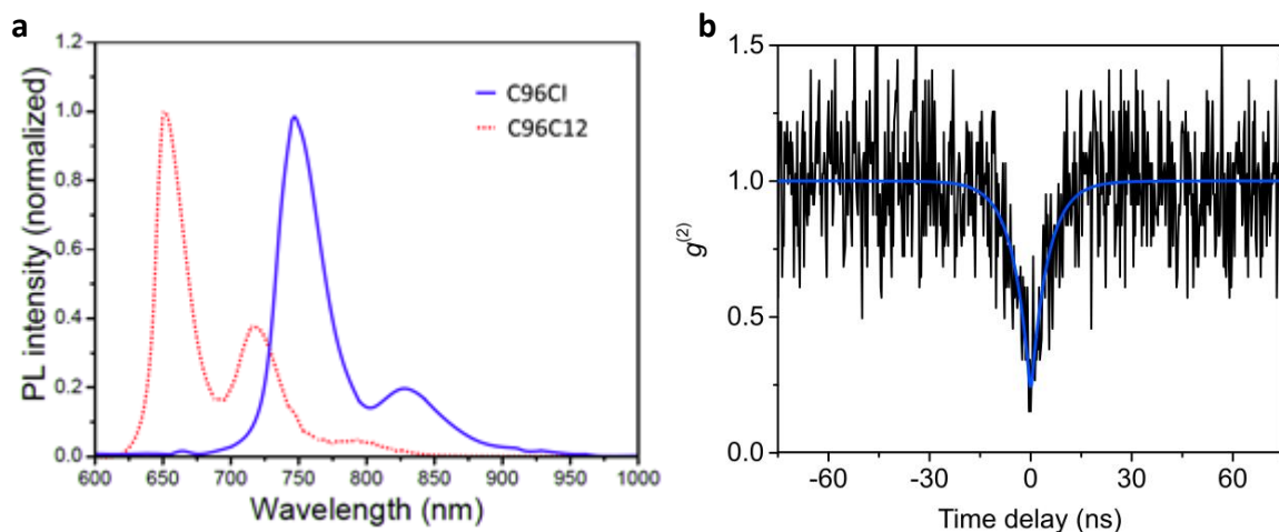
Figure 2.24: a) PL spectra of C96Cl 2 (blue line) and C96C12 3 (red dot line) and b) g^{(2)} function for C96Cl 2 .
