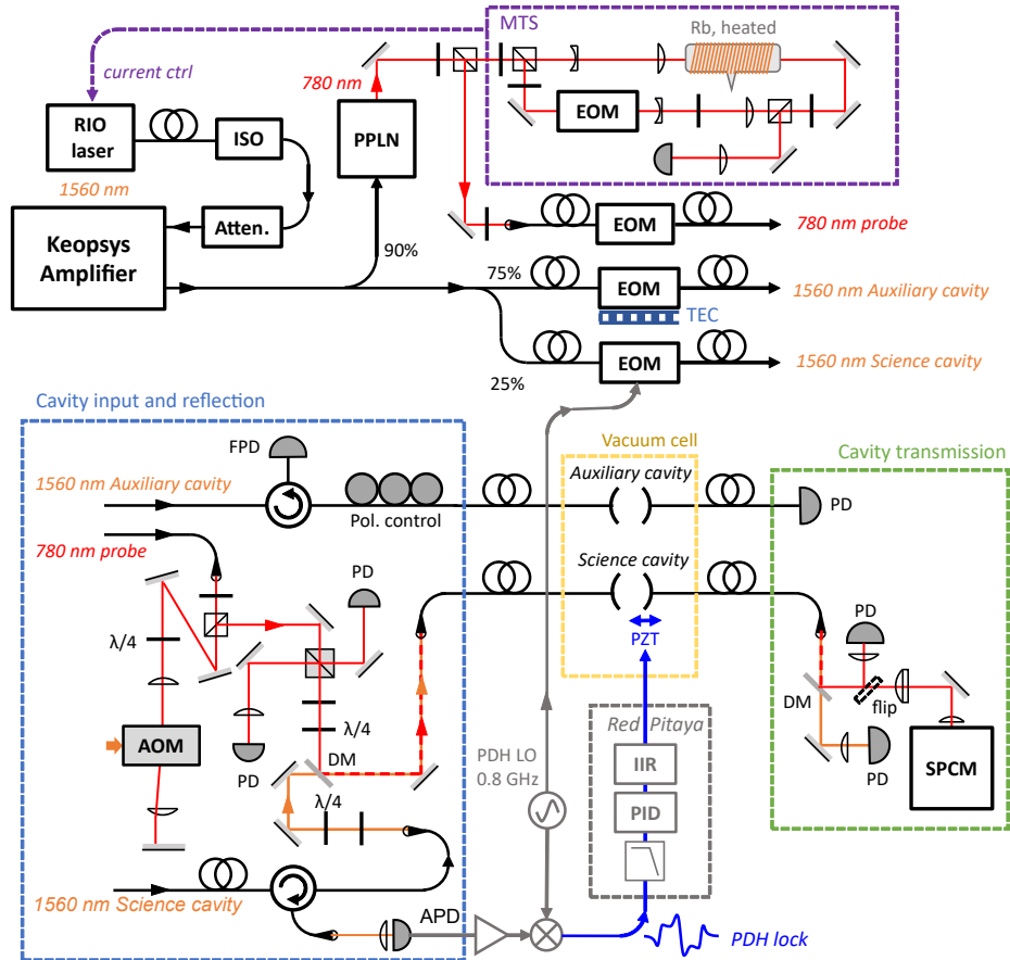
Figure 2.22 Schematics of the complete laser setup for cavity probing and stabilisation. Here we show direct PDH locking of the science cavity. Electronics are shown in grey. APD: avalanche photodiode; DM: dichroic mirror; FPD: fast photodiode; PZT: piezoelectric stack; SPCM: single photon counting module; TEC: thermoelectric cooler.
