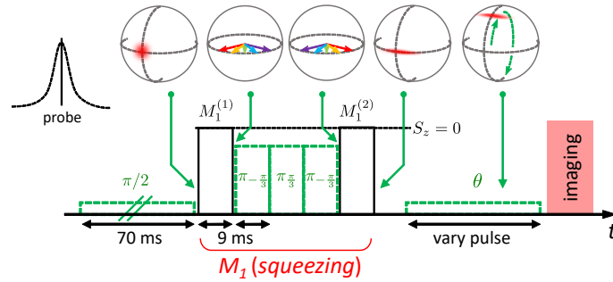
Figure 4.5 Sequence of coherence measurements using Rabi oscillations. The colour arrows on the Bloch sphere after the first probe M_1^{(1)} represent the strong dephasing induced by the probe photons, which is subsequently rephased by the second probe M_1^{(2)} . Here the probe is on resonance so M_1^{(2)} - M_1^{(1)} \approx 0 , not correlated with S_z . The decoherence is in principle only due to the transmitted probe photons, regardless of the probe detuning. Measurements with probe detuned at \kappa/2 are also compared in Fig. 4.6. After the composite measurement, we apply a MW pulse (same Rabi frequency as the first \pi/2 pulse) with variable lengths, along an axis perpendicular to the spin vector. The contrast of the Rabi oscillation measures the coherence.
