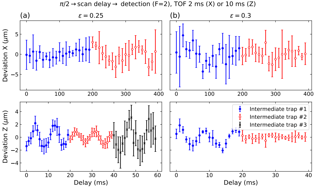
Figure 2.12 Residual oscillations in the clock trap. A \pi/2 pulse is applied once the decompression is finished to mimic a typical experimental cycle, but only |F=2\rangle is detected after a variable trap time (to avoid using ARP (Sec. 2.2.7.1)). Oscillations in \vec{x} (first row) and \vec{z} (second row) are measured in different timescales and with different TOFs (2 ms and 10 ms, respectively). We compare mainly two intermediate traps: the one used in TACC-1 (#1, trap frequencies \{50 \text{ Hz}, 550 \text{ Hz}, 550 \text{ Hz}\} ) and a tighter one (#2, \{55 \text{ Hz}, 1040 \text{ Hz}, 1040 \text{ Hz}\} ) that has a large displacement in the second step. The tightest trap (#3) aligned with the clock trap ( \{38 \text{ Hz}, 200 \text{ Hz}, 200 \text{ Hz}\} ) seems not tight enough, causing larger oscillations. We also vary the ramp of the second step by changing \epsilon , clearly for \epsilon = 0.25 (a) the ramp is too fast at the beginning, causing a larger oscillation compared to \epsilon = 0.3 (b). Oscillations in \vec{x} is not so strong. Data are shifted in the horizontal axis intentionally for visual clarity.
