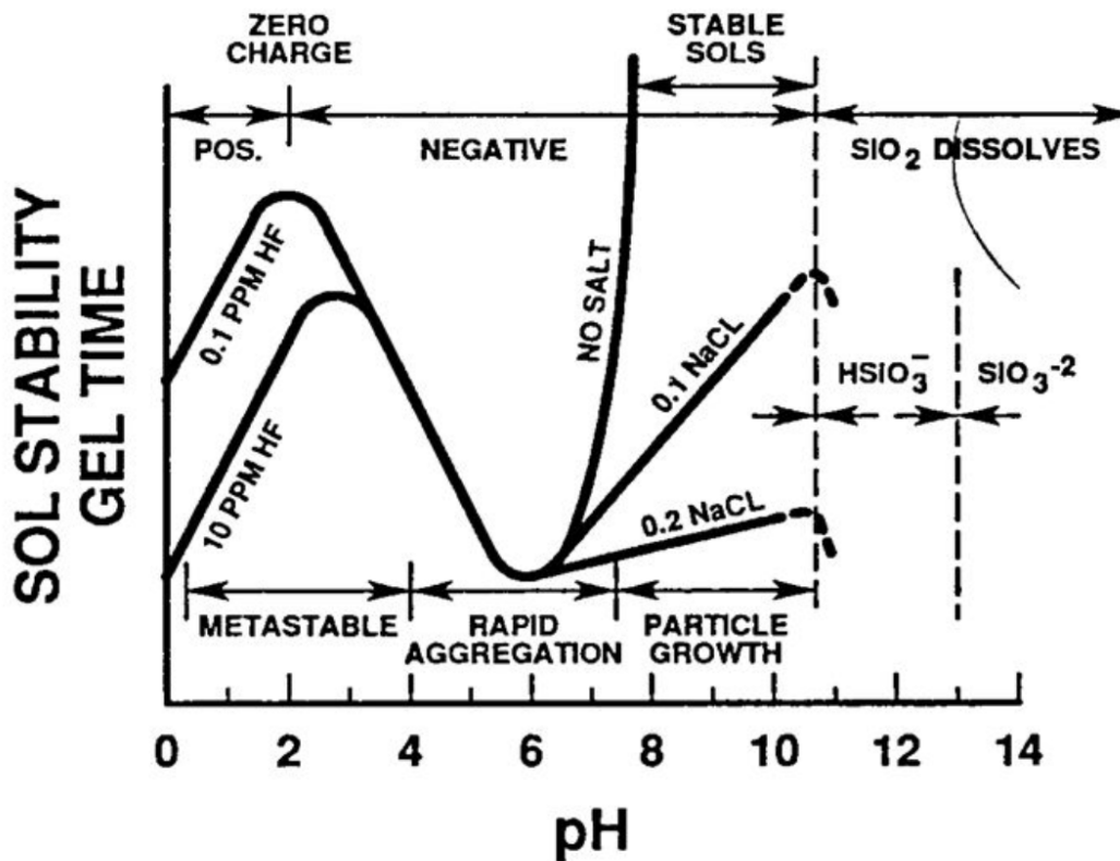
Figure 1.10 – Stability of colloidal silica and coagulation time, depending on pH and on NaCl concentration. Picture from reference [52].
