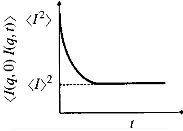
Figure 7.4 – Time autocorrelation function of I(q, t) as a function of time. Picture from reference [191].
