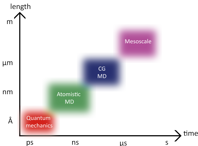
Figure 2.3 – Representation of different length and time scale in molecular simulations and the related methods.
