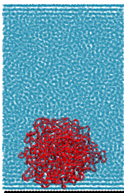
(a) Snapshot of the first situation (1S): PDMA (in red) placed on a flat silica surface (in black), surrounded by explicit solvent (in blue).
