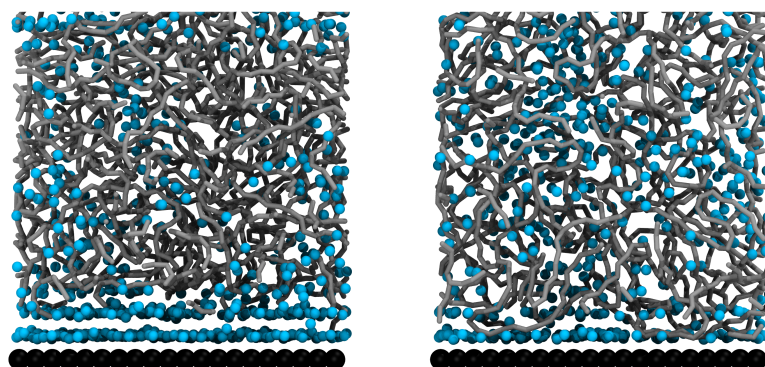
Figure 4.6 – Snapshot of half a simulation cell. Surface is in black, solvent in blue and polymer chains are in gray. PAAm is on the left side and PDMA on the right.
