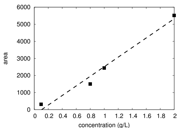
Figure 7.5 – TOC calibration curve of PDMA-155k.
