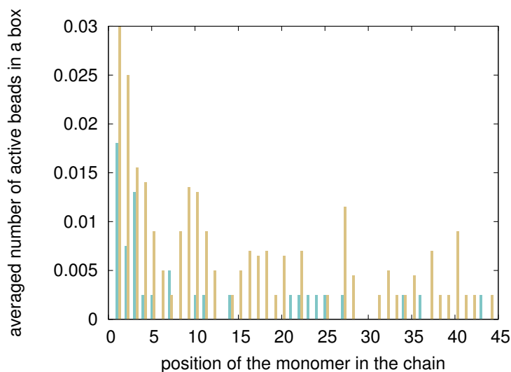
Figure 4.5 – Distribution of active beads in PAAm (blue) and PDMA (orange). Position 1 is the extremity of the chain; position 45 is the middle of the chain.
