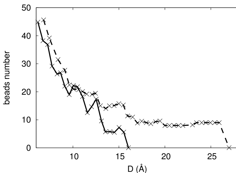
Figure 5.12 – Number of adsorbed beads close to the surface for PAAm (solid line) and PDMA (dashed line).
