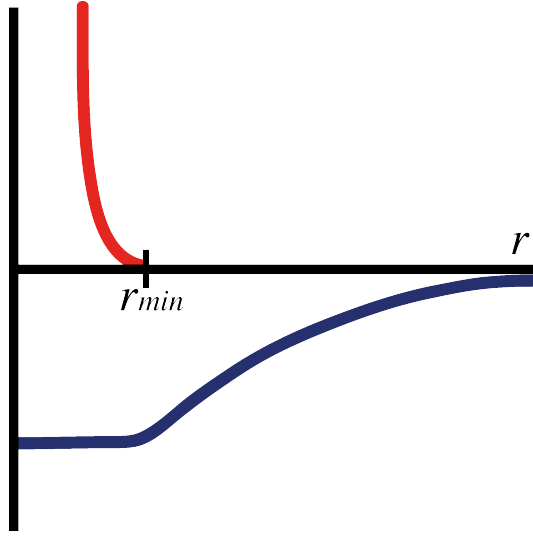
Figure 2.2 – Repulsive part of the LJ potential (red) and attractive part (blue).
