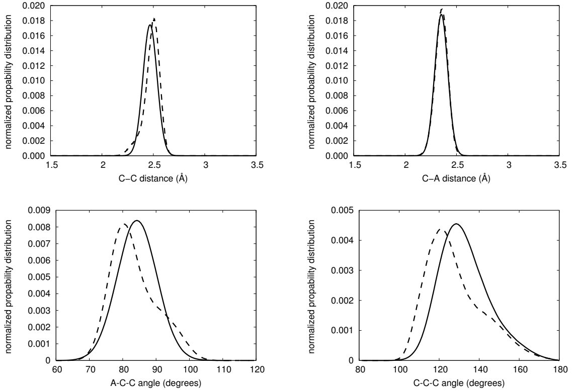
Figure 3.12 – Comparison between all atoms (dashed line) and coarse-grained (solid line) bonds and angles distribution.
