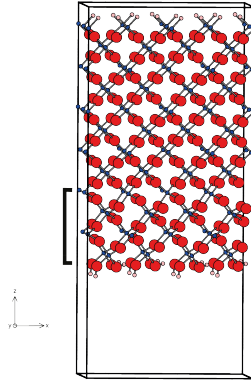
(a) 100 surface relaxed with 10 Å vacuum. The eight first atomic planes represent one layer (black square bracket). The surface is 216.6 \text{ Å}^2 is the x, y plane and the cell length is 36.2 Å in z direction.
