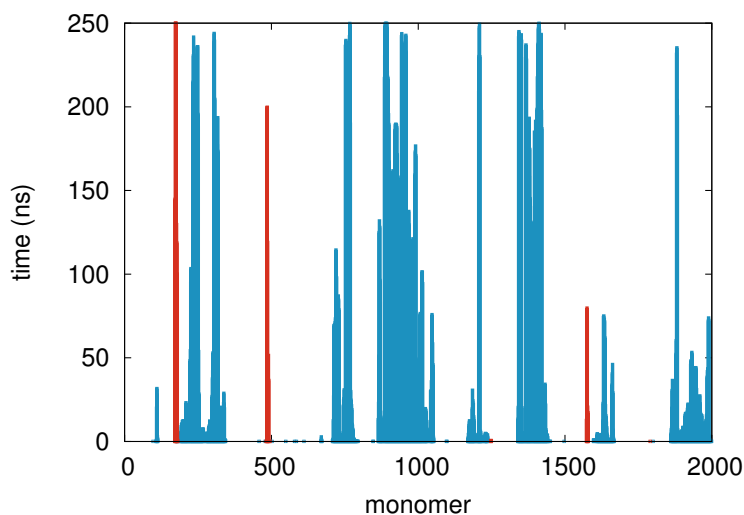
Figure 6.9 – Residence time in region I for each PDMA C bead, in situation (1S) (red) and in situation (2S) (blue).
