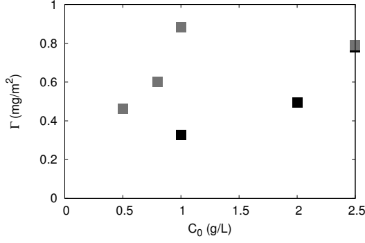
(a) Adsorption isotherm of PDMA with molecular weight of 45 000 g/mol (black squares) and 155 000 g/mol (gray squares). Corresponds to the adsorbed quantity of PDMA per surface unit as a function of the initial PDMA concentration.
