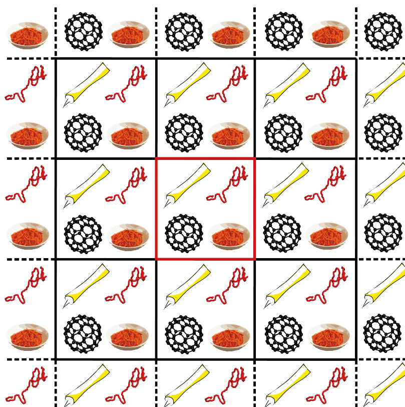
Figure 2.1 – Representation of PBC in two dimensions. The simulation cell, in red, is infinitely reproduced in the two directions.
