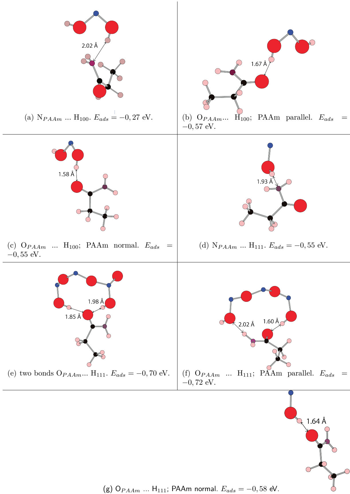
Figure 3.7 – PAAm adsorption on 100 and 111 surfaces and related adsorption energies E_{ads} . H_{100} is an hydrogen from the 100 surface and H_{111} is an hydrogen from the 111 surface.
