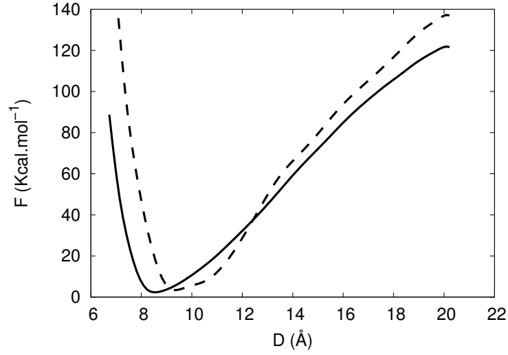
Figure 5.3 – Free energy profile for PAAm (solid line) and PDMA (dashed line) in an implicit solvent at 300 K.
