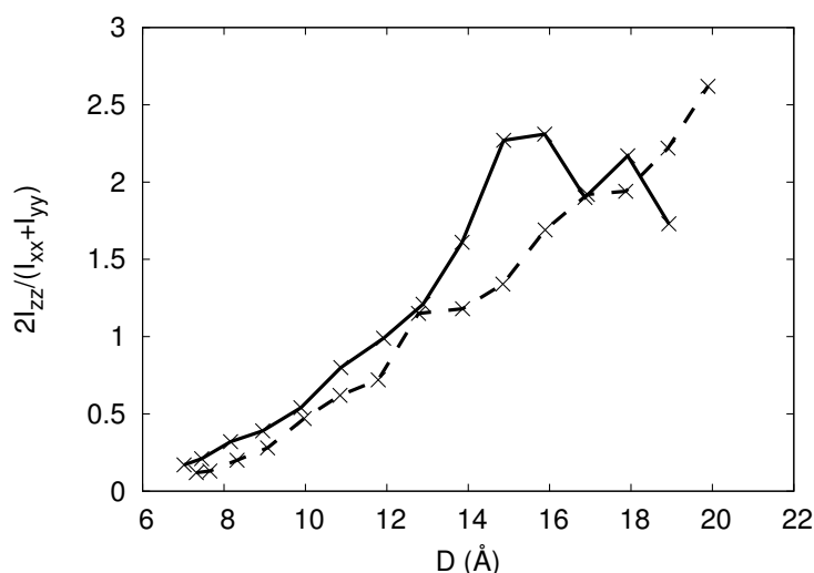
Figure 5.5 – Evolution of the shape of PAAm (solid line) and PDMA (dashed line) along the direction normal to the surface. Implicit solvent at 300 K.
