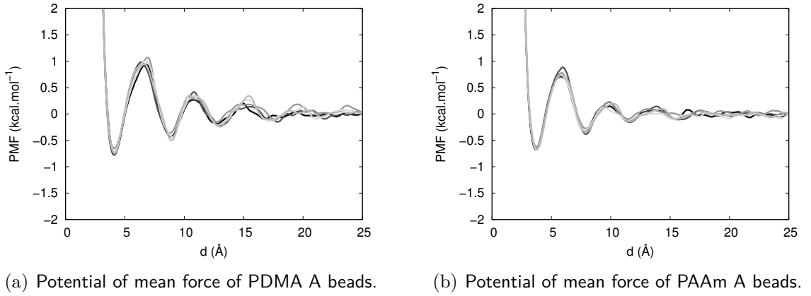
Figure 4.10 – Potential of mean force of PDMA A beads and PAAm A beads interacting through an implicit solvent collected in five independent simulations. .
