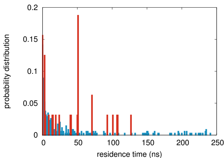
Figure 6.8 – Histogram of residence times of PDMA active C beads for situation (1S) (red) and situation (2S) (blue).
