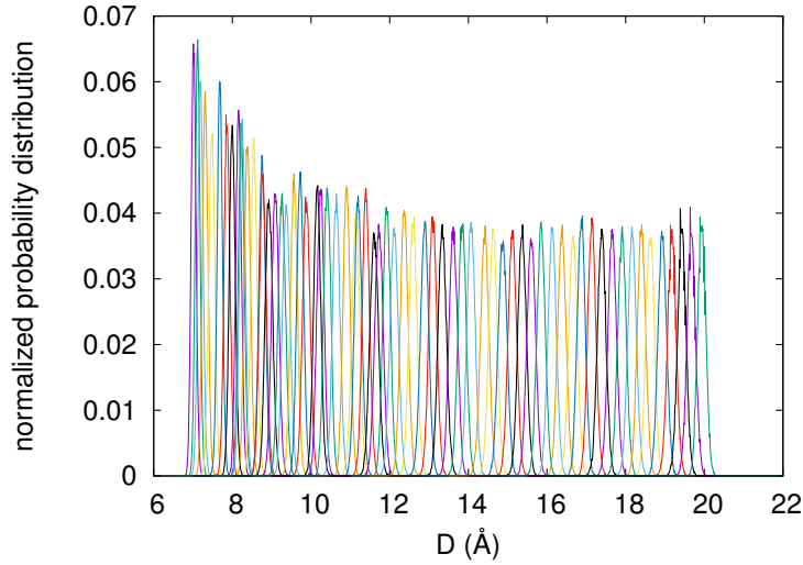
Figure 5.2 – Histogram distributions as a function of distances D .
