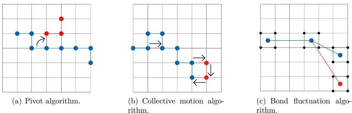
Figure 2.4 – Representation of three lattice methods. The lattice is in black, initial configuration of the chain is in blue (beads are depicted as plain circles and bonds as solid lines), final configuration is in red and arrows indicate the direction of the move.
