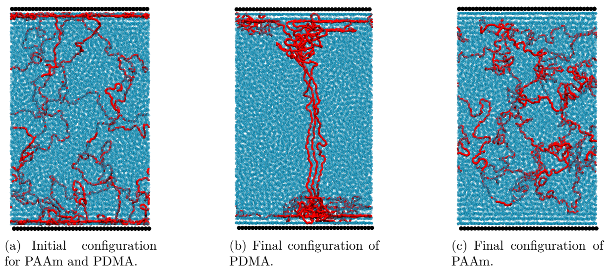
Figure 6.1 – Snapshots of the initial and final configurations of PDMA and PAAm between two flat silica surfaces. The silica surface is in black, solvent beads are in blue and the polymer chain is in red.
