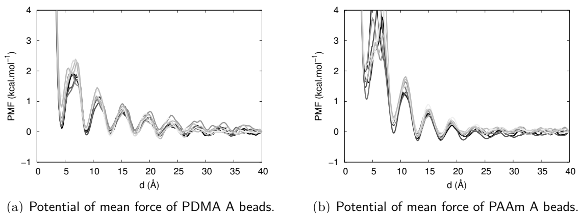
Figure 4.3 – Potential of mean force of PDMA A beads and PAAm A beads collected in nine independent simulations. .
