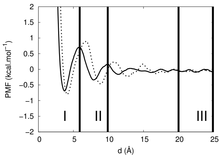
Figure 4.8 – Potential of mean force of PAAm (solid line) and of PDMA (dashed line). Implicit solvent.
