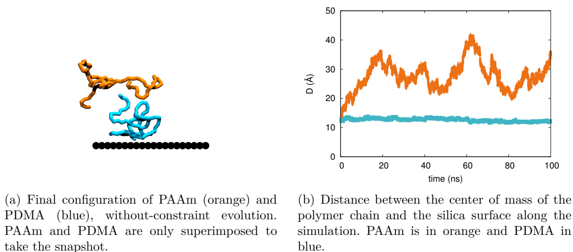
Figure 5.10 – Without-constraint evolution of PDMA and PAAm.
