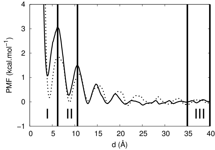
Figure 4.2 – Potential of mean force of PAAm (solid line) and of PDMA (dashed line) both in explicit solvent.
