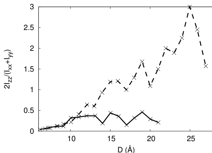
Figure 5.11 – Evolution of the shape of PAAm (solid line) and PDMA (dashed line) along the direction normal to the surface. Explicit solvent at 500K.
