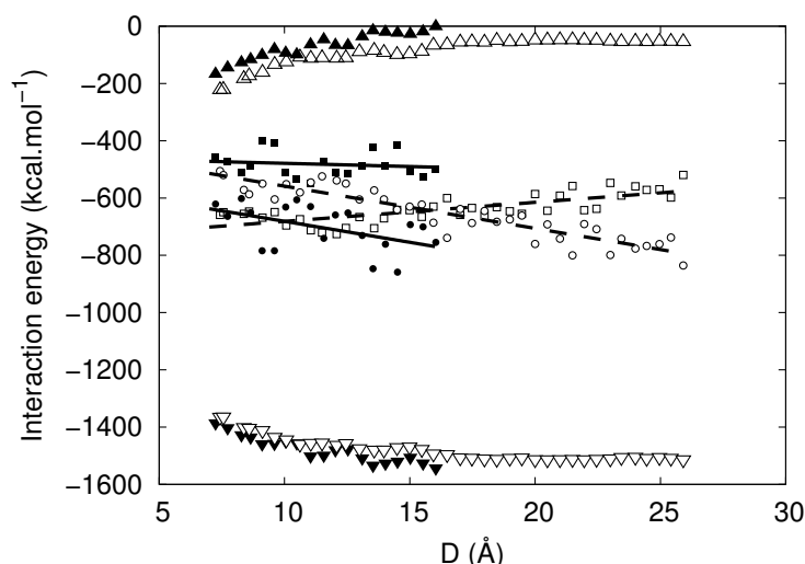
Figure 5.15 – Interaction energies for PAAm (solid line and black symbols) and PDMA (dashed line and open symbols). Polymer/surface (▲ for PAAm and △ for PDMA), polymer/polymer (■ for PAAm and □ for PDMA), polymer/solvent (● for PAAm and ○ for PDMA) and surface/solvent (▼ for PAAm and ▽ for PDMA) interaction energies are represented.
