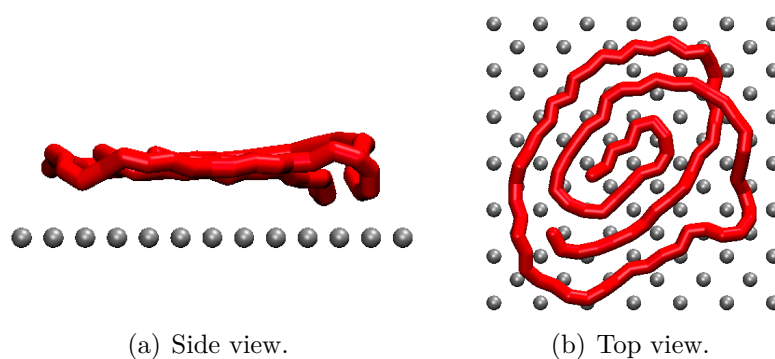
Figure 5.8 – Side and top view of the PDMA chain on silica surface at D equals 7.2 Å. Only the backbone chain (C beads) is represented. Implicit solvent at 500 K.
