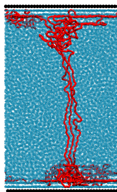
(b) Snapshot of the second situation (2S): PDMA (in red) shared between two flat silica surfaces (in black), surrounded by explicit solvent (in blue).
