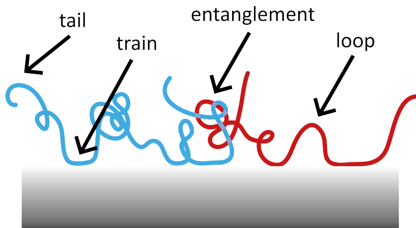
Figure 1.8 – Entangled adsorbed layer of polymer chains with trains, tails and loops.
