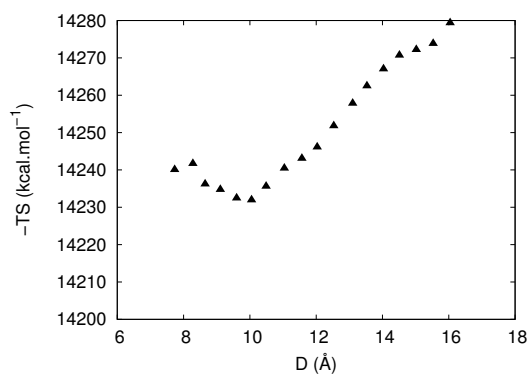
(c) Entropy (-TS) of PAAm.
