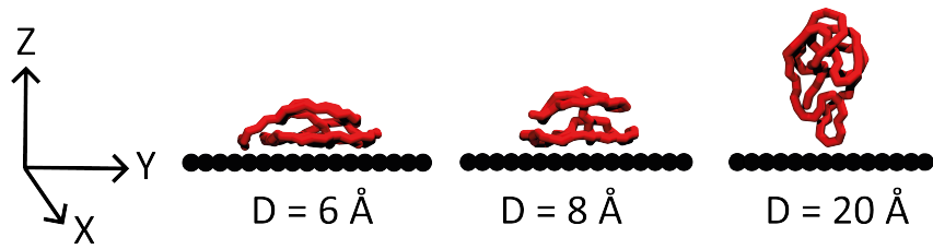
Figure 5.4 – Evolution of the polymer shape as D increases.
