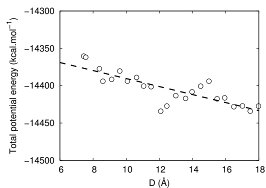
(b) Total potential energy of PDMA.
