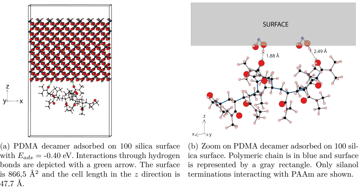
Figure 3.10 – Decamer of PDMA on the 100 surface.
