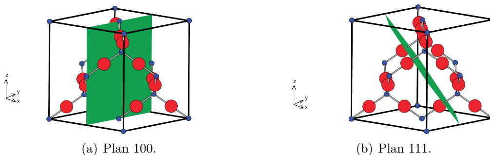
Figure 3.5 – Planes in \beta cristobalite. Oxygen atoms are in red and silicon atoms are in blue.
