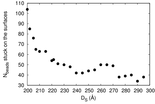
(a) Number of beads that remain in region I for 250 ns at least.
