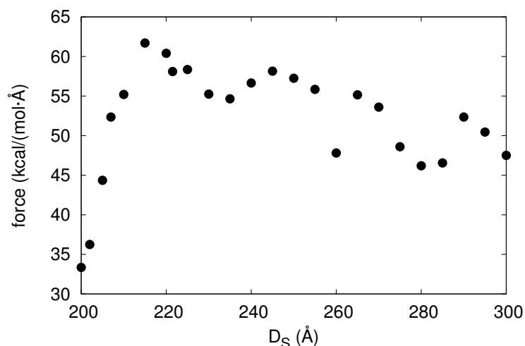
Figure 6.14 – Force strength between PDMA and surfaces.
