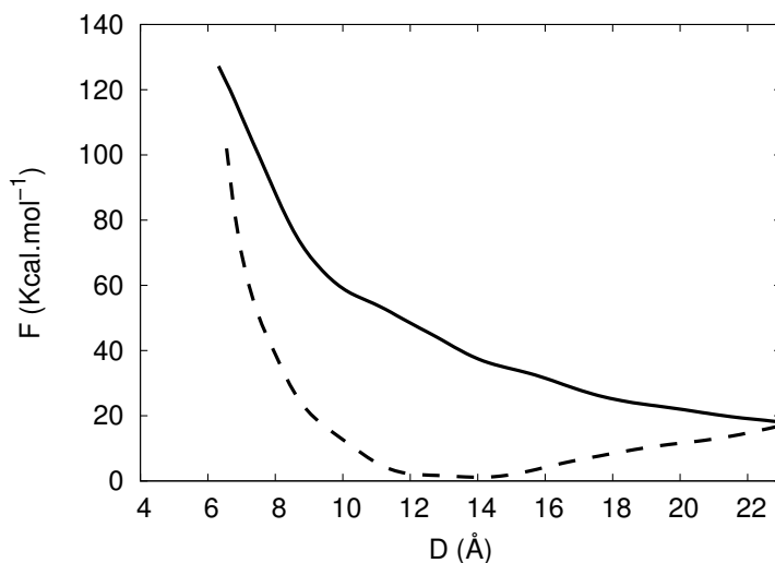
Figure 5.9 – Free energy profile for PAAm (solid line) and PDMA (dashed line) in an explicit solvent at 500 K.
