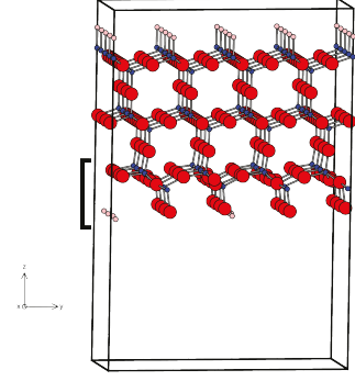
(b) 111 surface relaxed with 10 Å vacuum. The four first atomic planes represent one layer (black square bracket). The surface is 375.1 \text{ Å}^2 is the x, y plane and the cell length is 26.2 Å in z direction.
