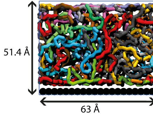
Figure 4.7 – Snapshot of a simulation cell containing 24 chains of 90 monomers of PAAm (one color corresponds to one chain) and 200 silica beads (black).
