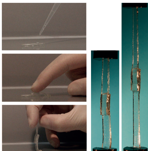
Figure 1.7 – Gluing two PDMA strips by spreading a droplet of silica nanoparticles solution in between them and simply bringing them into contact (left picture). The resulting junction is able to undergo large deformations (right picture). Pictures from reference [1].
