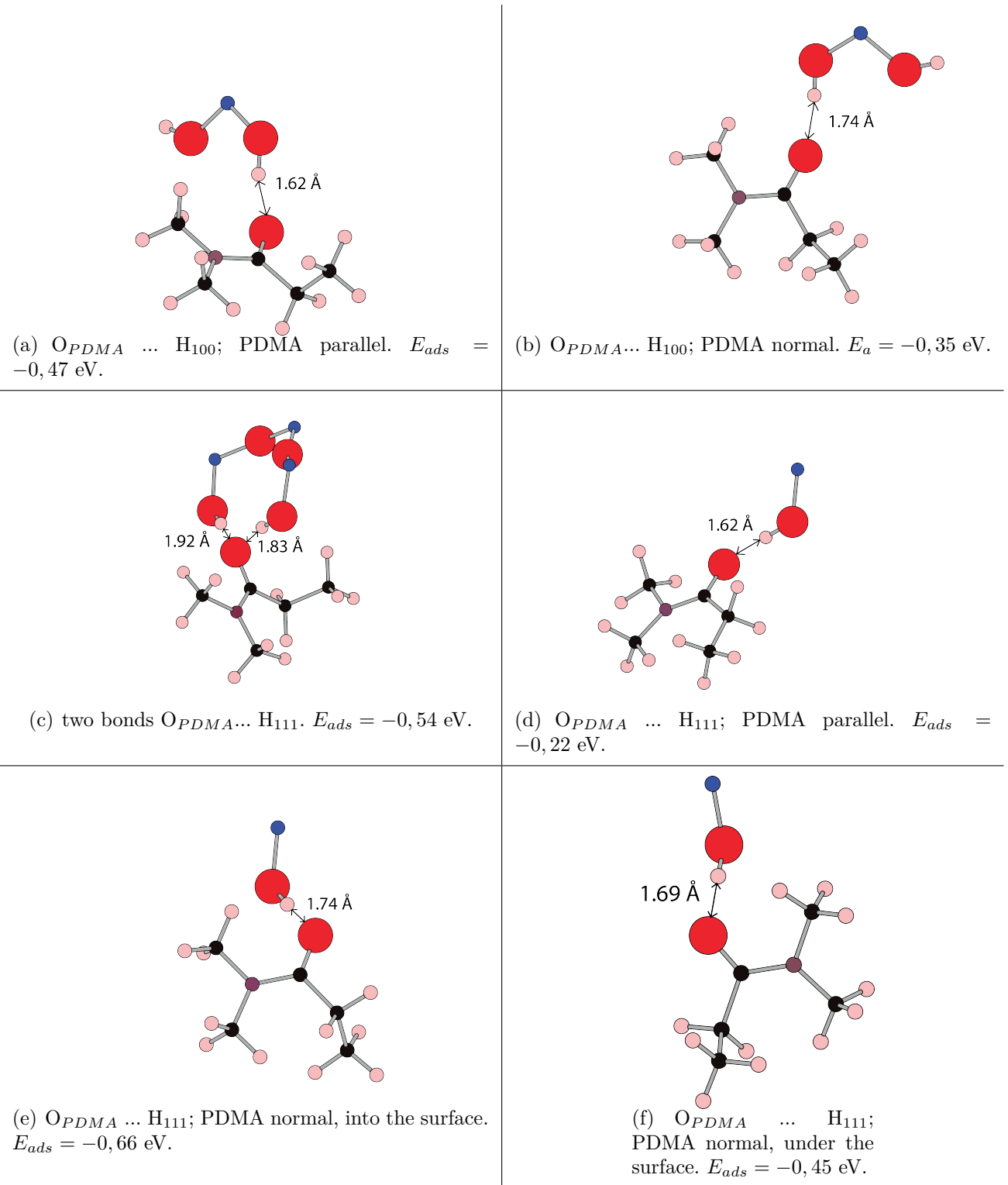
Figure 3.8 – PDMA adsorption on 100 and 111 surfaces and related adsorption energies E_{ads} . H_{100} is an hydrogen from the 100 surface and H_{111} is an hydrogen from the 111 surface.
