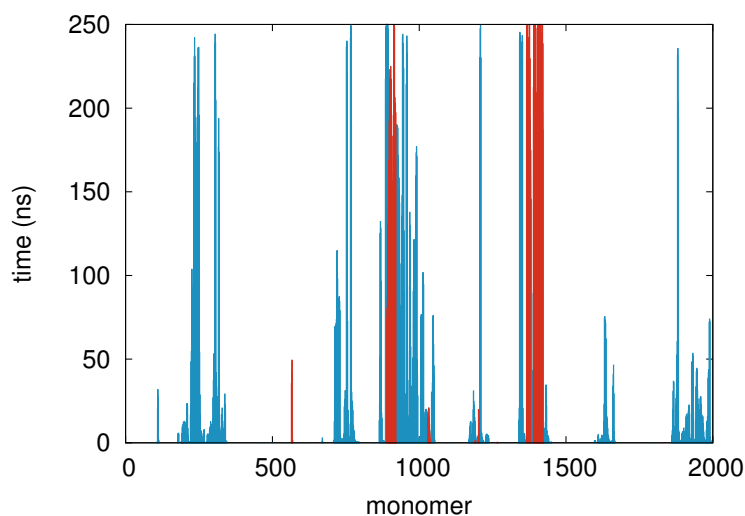
Figure 6.10 – Residence time, per PDMA C bead, close to the surface (nanoseconds). In blue: initial configuration, distance between the two surfaces = 200 Å. In red: distance between the two surfaces = 285 Å.
