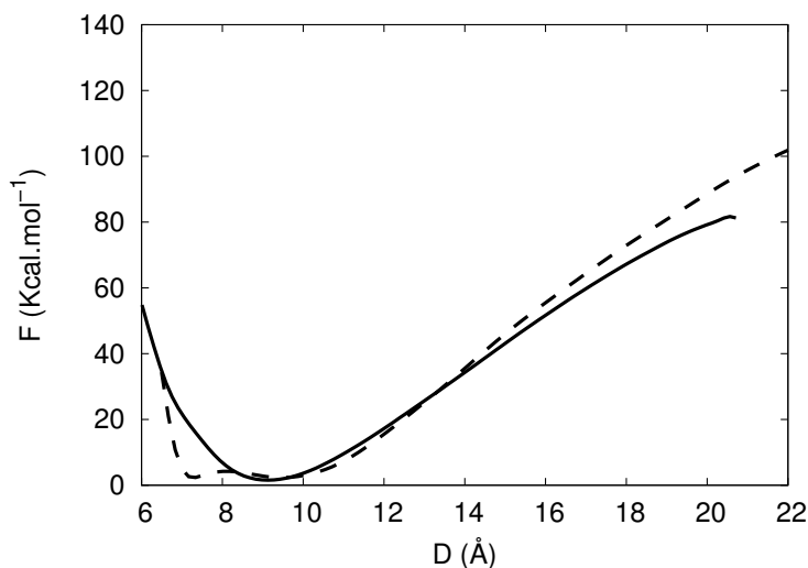
Figure 5.6 – Free energy profile for PAAm (solid line) and PDMA (dashed line) in an implicit solvent at 500 K.
