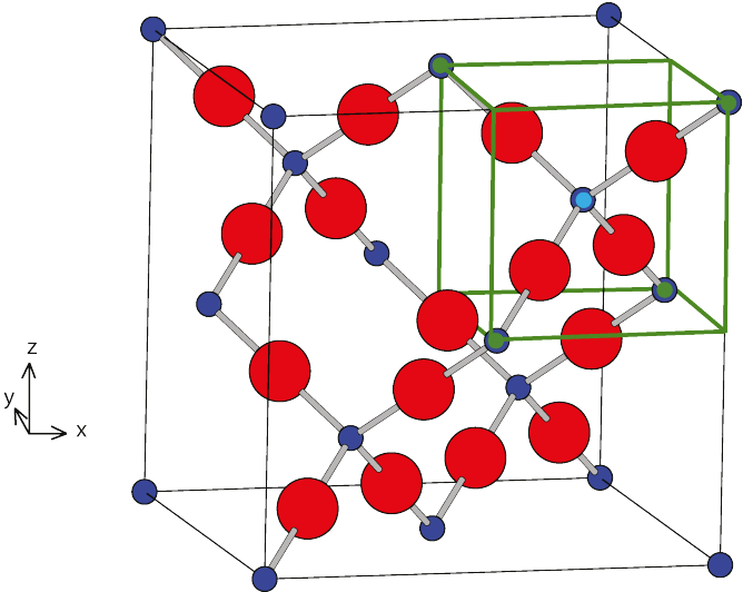
Figure 3.3 – \beta cristobalite primitive cell (black solid lines). Oxygen atoms are in red and silicon atoms are in blue.
