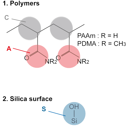
Figure 3.11 – Coarse-grained mapping of the polymer and the silica surface.
