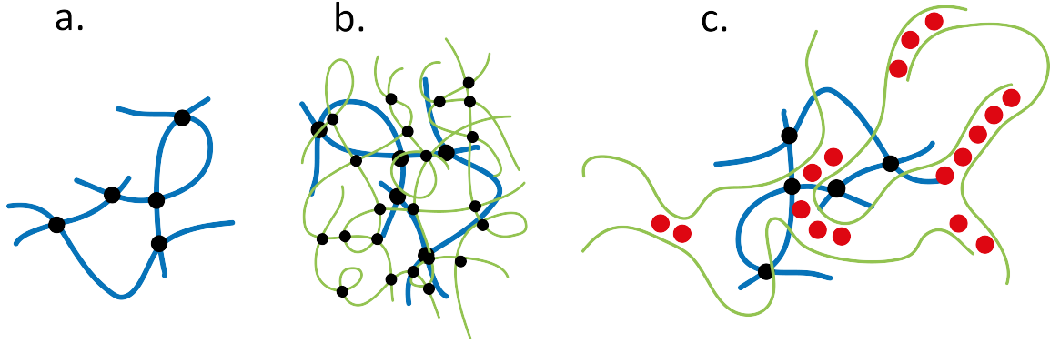
Figure 1.5 – a. Normal hydrogel: polymer chains are in blue and cross-links are black circles. b. Double-network hydrogel: the first polymer network is in green and the second in blue. c. Hydrogel with hybrid chemical and physical cross-linkers: blue chains are chemically cross-linked while green chains form ionic cross-links through \text{Ca}^{2+} ions (red circles). Inspired by figure 1 of reference [18].
