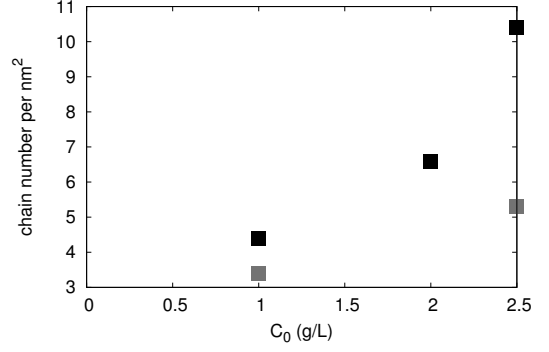
(b) Number of adsorbed PDMA chains per \text{nm}^2 as a function of the initial PDMA concentration. PDMA with molecular weight of 45 000 g/mol is in black and 155 000 g/mol in gray.
