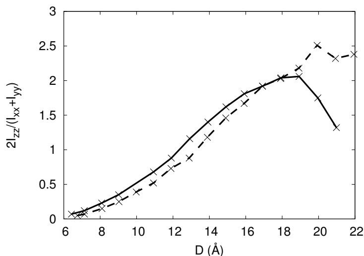
Figure 5.7 – Evolution of the shape of PAAm (solid line) and PDMA (dashed line) along the direction normal to the surface. Implicit solvent at 500 K.
