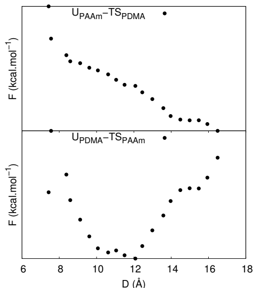
Figure 5.14 – Free energy from mixed potential energy and entropy between PAAm and PDMA.
