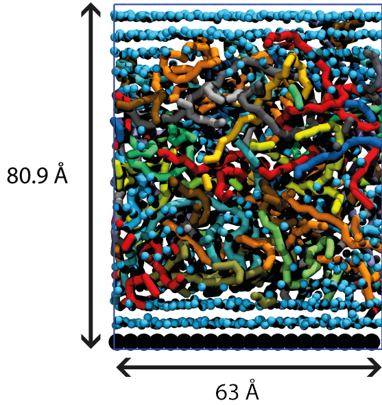
Figure 4.1 – Snapshot of a simulation cell containing 24 PAAm chains of 90 monomers each (one color corresponds to one chain), 200 silica beads (black) and 960 solvent beads (light blue).
