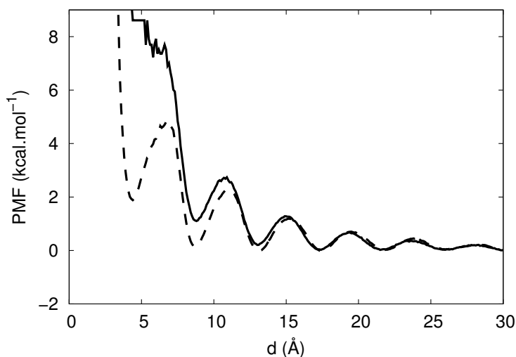
Figure 6.2 – Potential of mean force of A beads of PAAm (solid line) and PDMA (dashed line).
