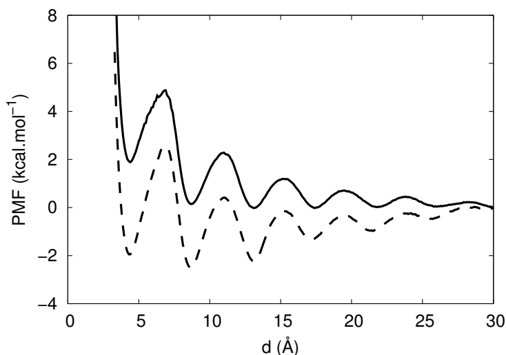
Figure 6.7 – Potential of mean force of PDMA A beads in situation (1S) (dashed line) and situation (2S) (solid line).
