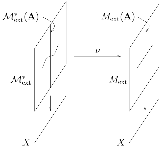
FIGURE 1. Isomonodromic Deformations
