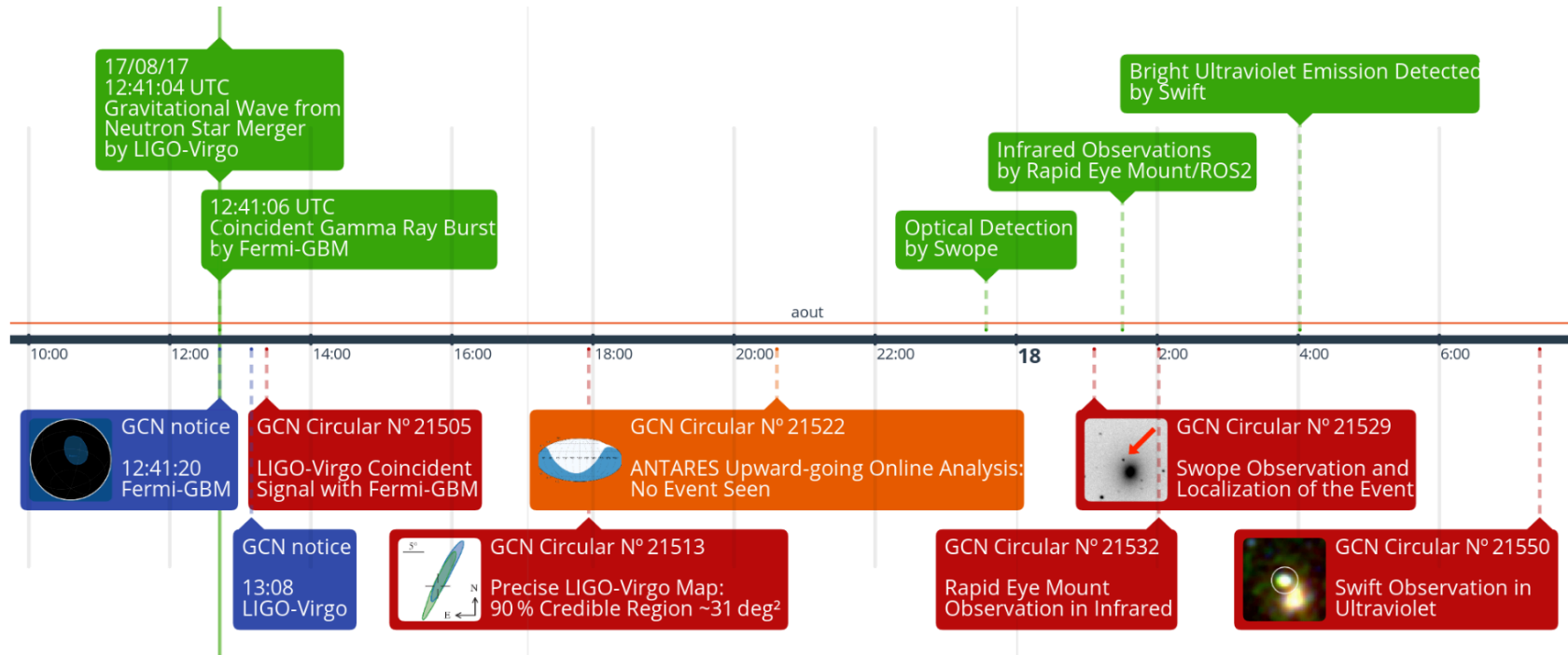
Figure 9.7 – Timeline of the multi-messenger observations of the GW170817 event (green) as well as the Gamma-ray Coordinates Network (GCN) notices (blue) and circulars (red) sent subsequently in the 18 hr following the event. The ANTARES GCN circular is represented in orange.
