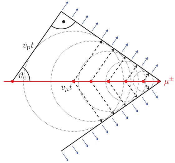
Figure 2.3 – Illustration of the cone shape of the Cherenkov effect. The atoms (red dots) along the path of the charged particle (red line) travelling faster than the light phase velocity in the medium emit Cherenkov light (dotted circles) which forms a wave front with a characteristic angle \theta_c . Figure taken from [13].
