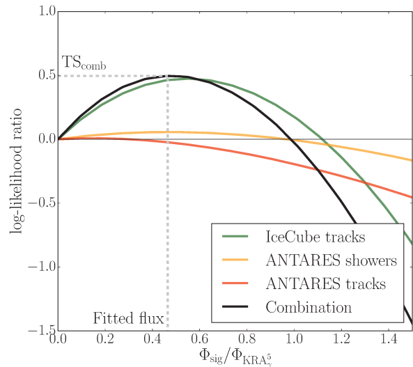
Figure 6.5 – Log-likelihood ratio curves and fitting of the flux for the combined analysis. The black curve is the sum of the three other ones. These curves correspond to unblinded data using the likelihood for the model with the 5 PeV cutoff.
