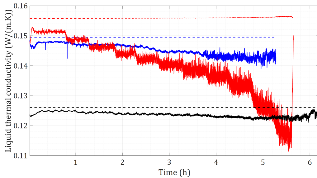
Figure F.6: Evolution of the liquid thermal conductivity during progressive heat load tests of the three working fluids: nitrogen at saturation temperature (—), nitrogen at condenser's temperature (---), neon at saturation conditions (—), neon at condenser's temperature (---), argon at saturation conditions (—) and argon at condenser's temperature (---).
