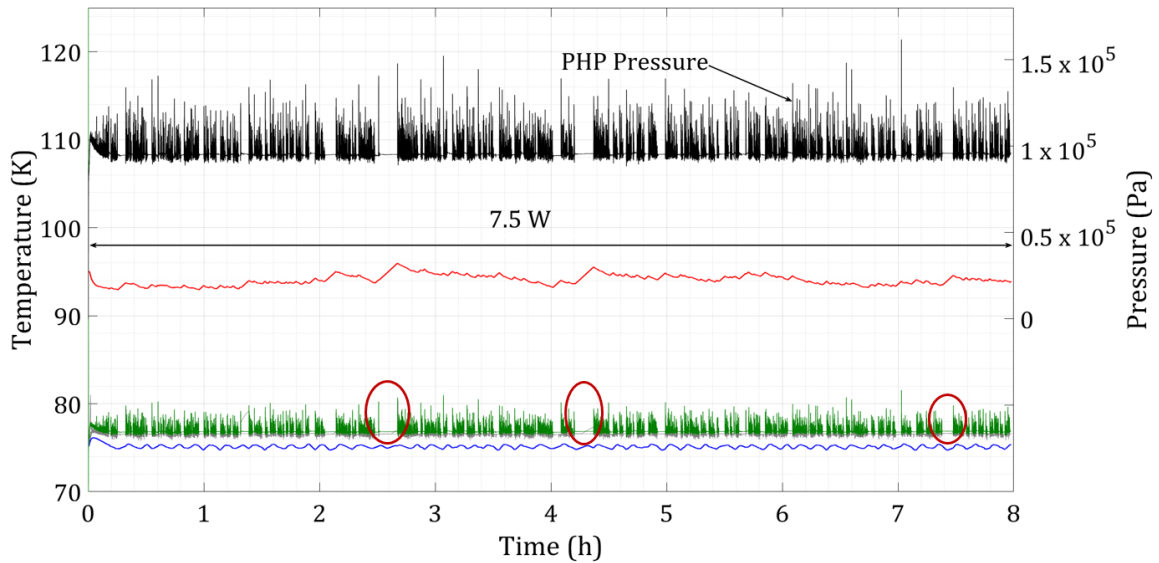
Figure 5.4: Evolution of the PHP pressure ( \blackrightarrow ), the saturation temperature ( \text{---} ), the average temperature of the evaporator ( \text{---} ) and the condenser ( \text{---} ) and the temperatures of the adiabatic part ( \text{---} ) of a fixed heat load experiment in open configuration using nitrogen as working fluid in the PHP with 24 turns.
