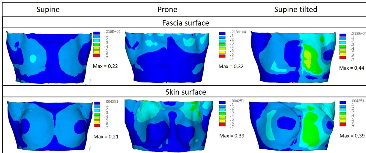
Figure 5.6: Strain distribution when using a Gent material model.
