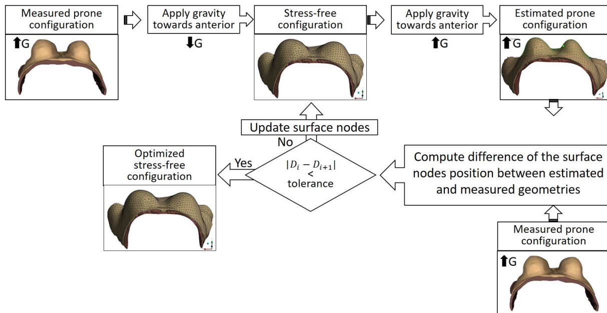
Figure 2.15: Prediction-correction algorithm
