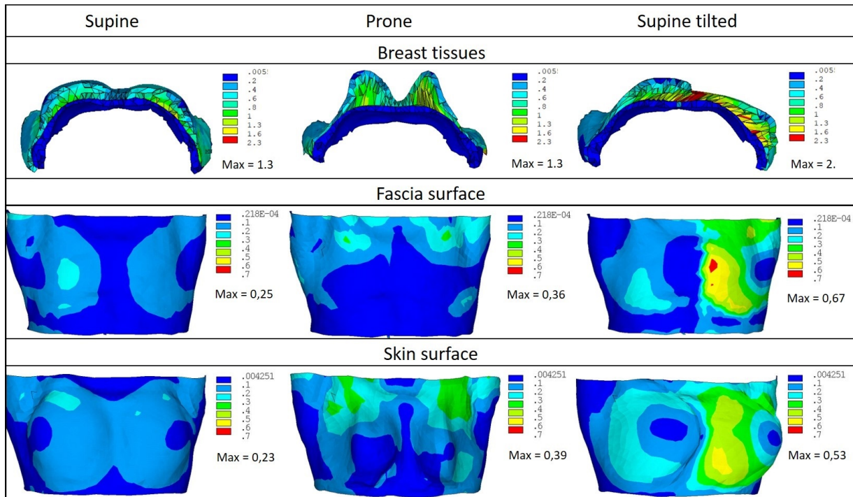
Figure 5.5: Strain distribution when using a Neo-Hookean material model.
