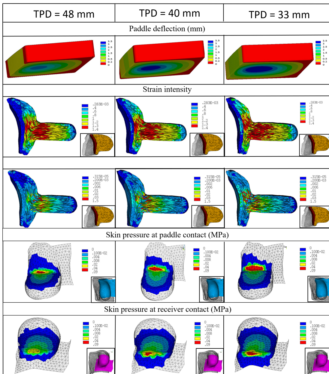
Figure 5.15: Stress, strain and contact pressure distributions for a variable thoracic cage to paddle distance (TPD).
