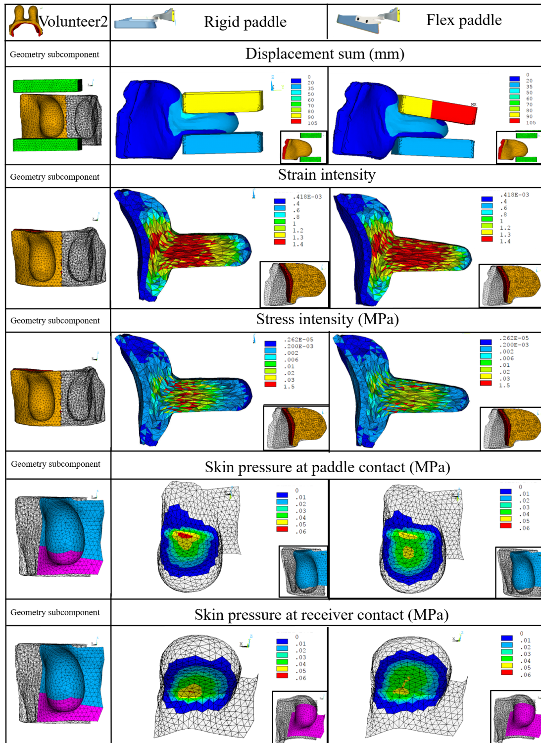
Figure 5.13: Stress, strain and contact pressure distributions for the second volunteer
