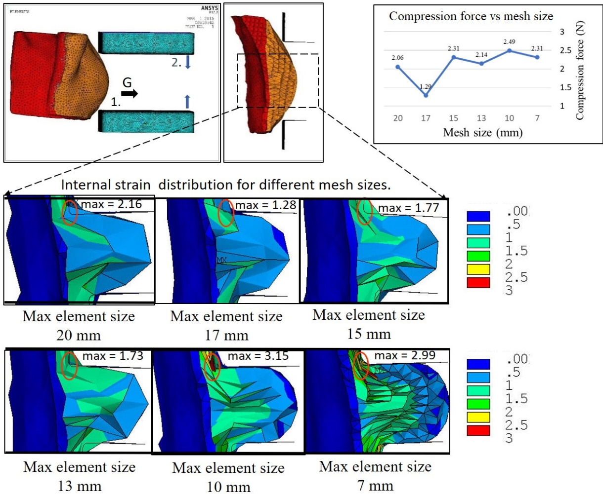
Figure B.1: Internal strain distribution as a function of the elements size.
