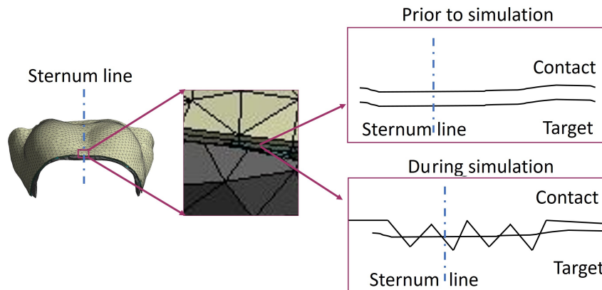
Figure 3.12: Tissues accumulation on the sternum line with excessive sliding
