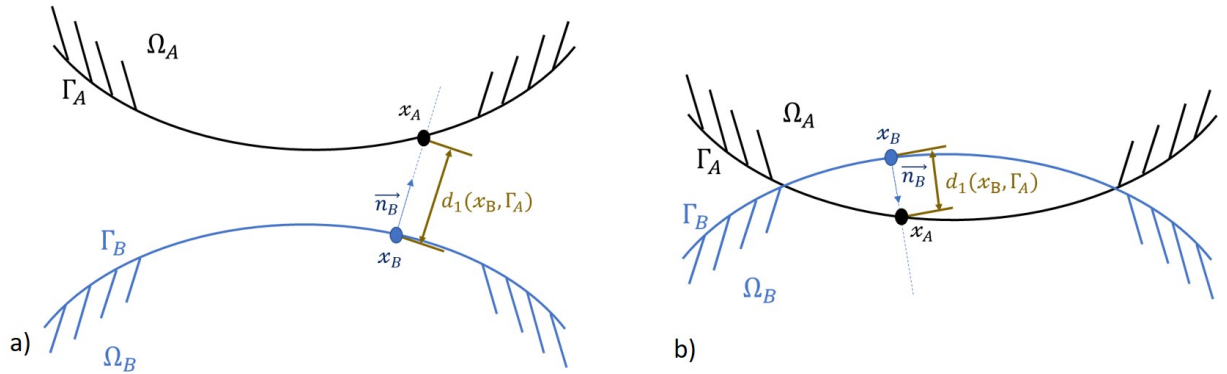
Figure 2.13: a) Body \mathcal{A} and body \mathcal{B} are close but not in contact. The d_1(x_B, \mathcal{A}) measure define the gap between the bodies at point x_B . b) Body \mathcal{B} have penetrated the body \mathcal{A} . The d_1(x_B, \mathcal{A}) measure gives the penetration at point x_B .
