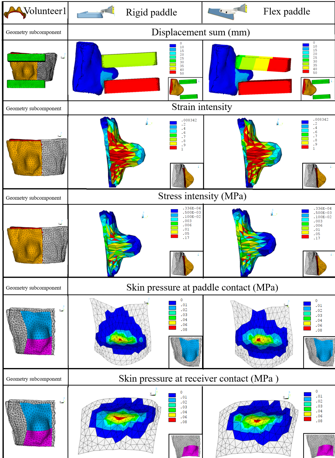
Figure 5.12: Stress, strain and contact pressure distributions for the first volunteer
