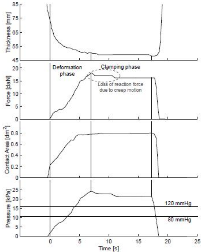
Figure 4.4: A typical breast compression cycle. Reproduced from Groot et al. [62]
