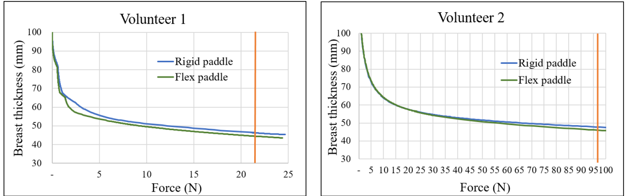
Figure 5.4: Resulting breast flattening curve as function of the compression force with Gent constitutive model. The orange line shows the breast thickness corresponding to the target compression force measured during mammography.
