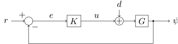
Figure 5.5: Regulation scheme for Ciscrea yaw angle control.
