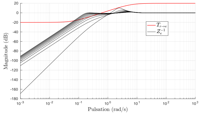
Figure 5.8: Diagram of T_{r \to e} and Z_e^{-1} .
