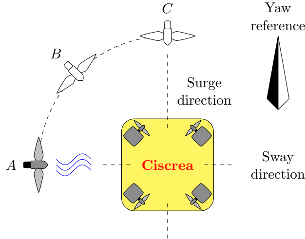
Figure 5.13: Top view of experiment setup
