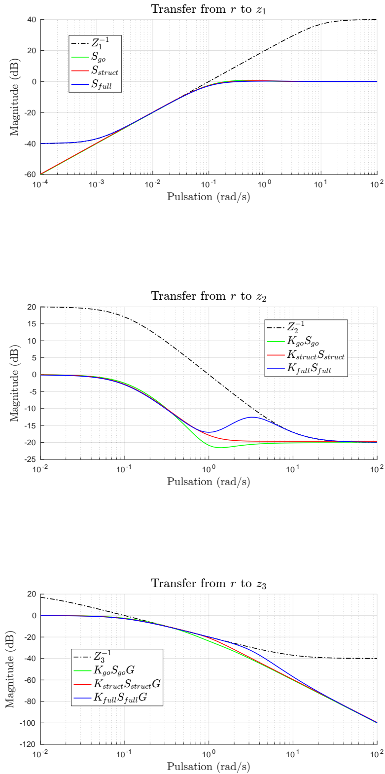
Figure 4.3: Frequency specifications, displayed in dotted, and closed loop objective transfers for the three controllers.
