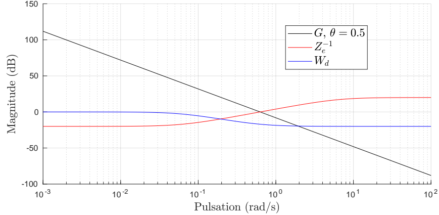
Figure 5.7: Gain of the frequency templates Z_e^{-1} in red, disturbance weighting function W_d in blue, and G in black at \theta = 0.5 .
