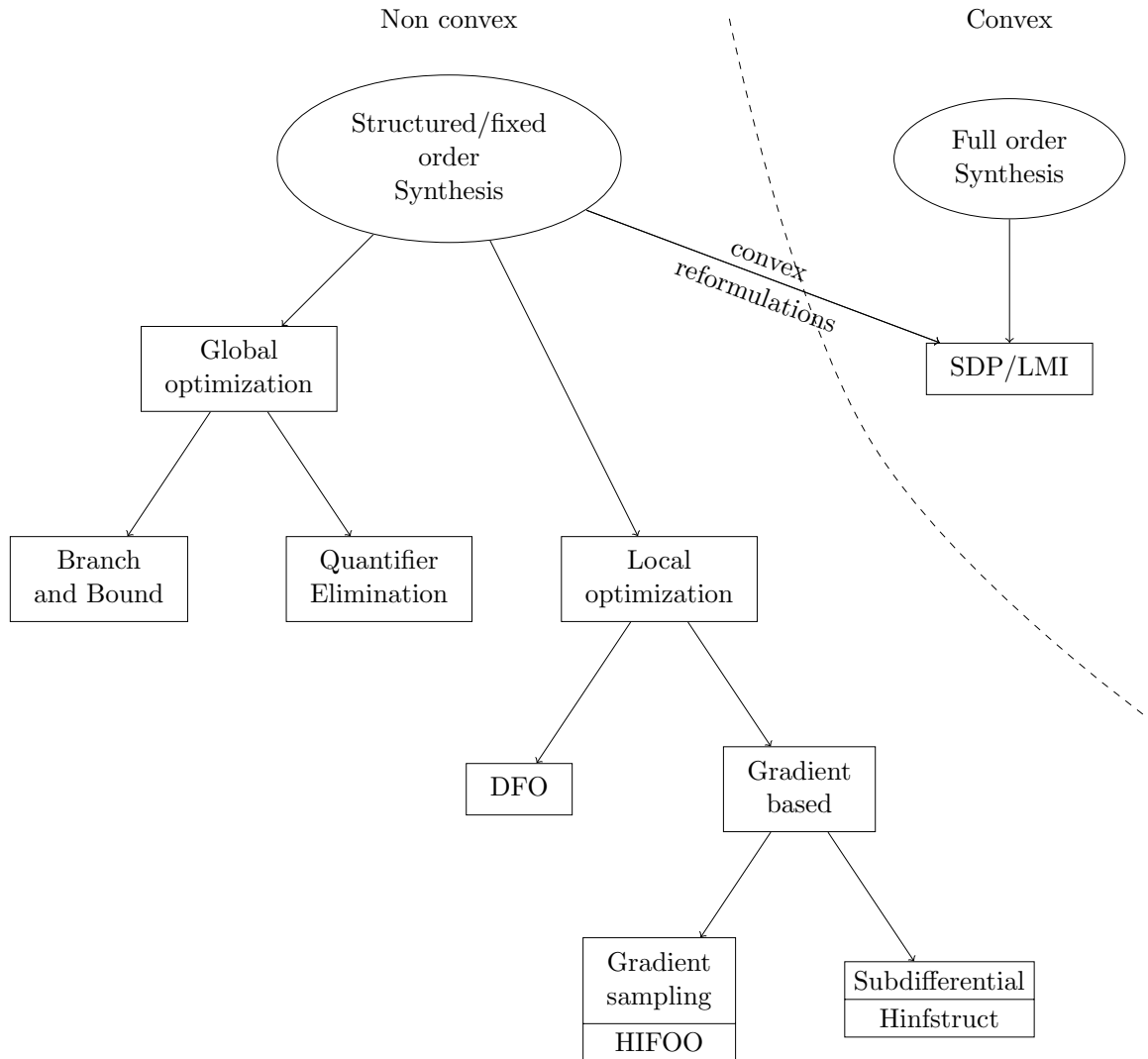
Figure 1.8: Chart of optimization approaches to the H_\infty synthesis problem.
