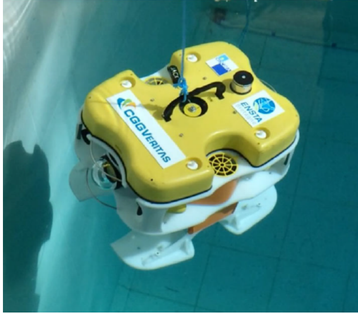
Figure 5.1: Ciscrea AUV.
