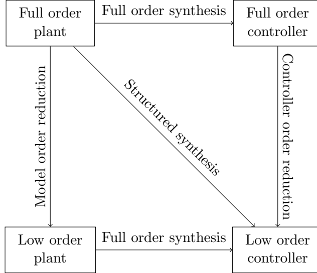
Figure 1.7: Low order controller synthesis process.
