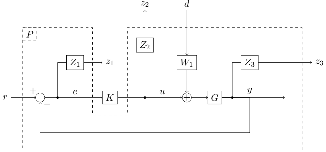
Figure 1.5: H_\infty sensitivity approach.
