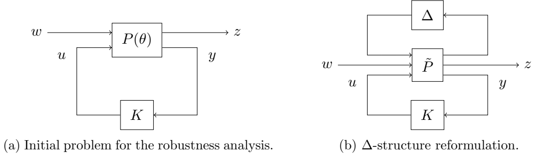
Figure 1.9: \Delta -structure representation of uncertainty.
