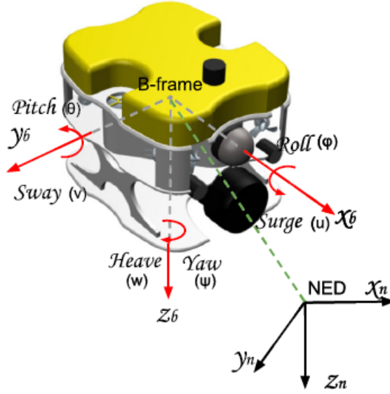
Figure 5.2: NED-frame and B-frame.
