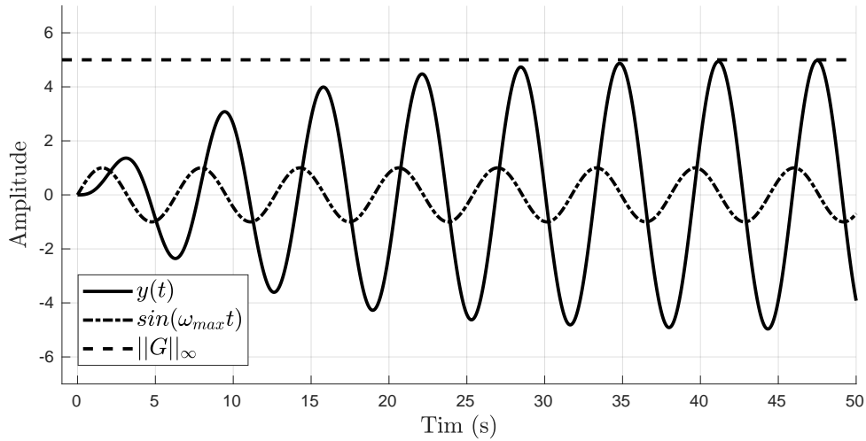
(b) Time response of G to a sine wave input.
