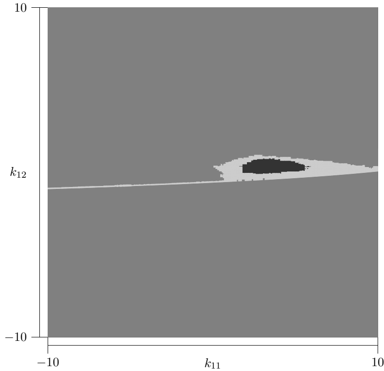
Figure 4.4: Characterization of feasible tunable parameters for the AC7 problem.
