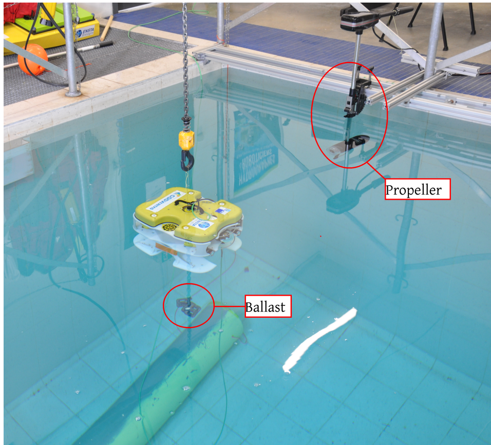
Figure 5.12: Experimental setup at ENSTA Bretagne pool.
