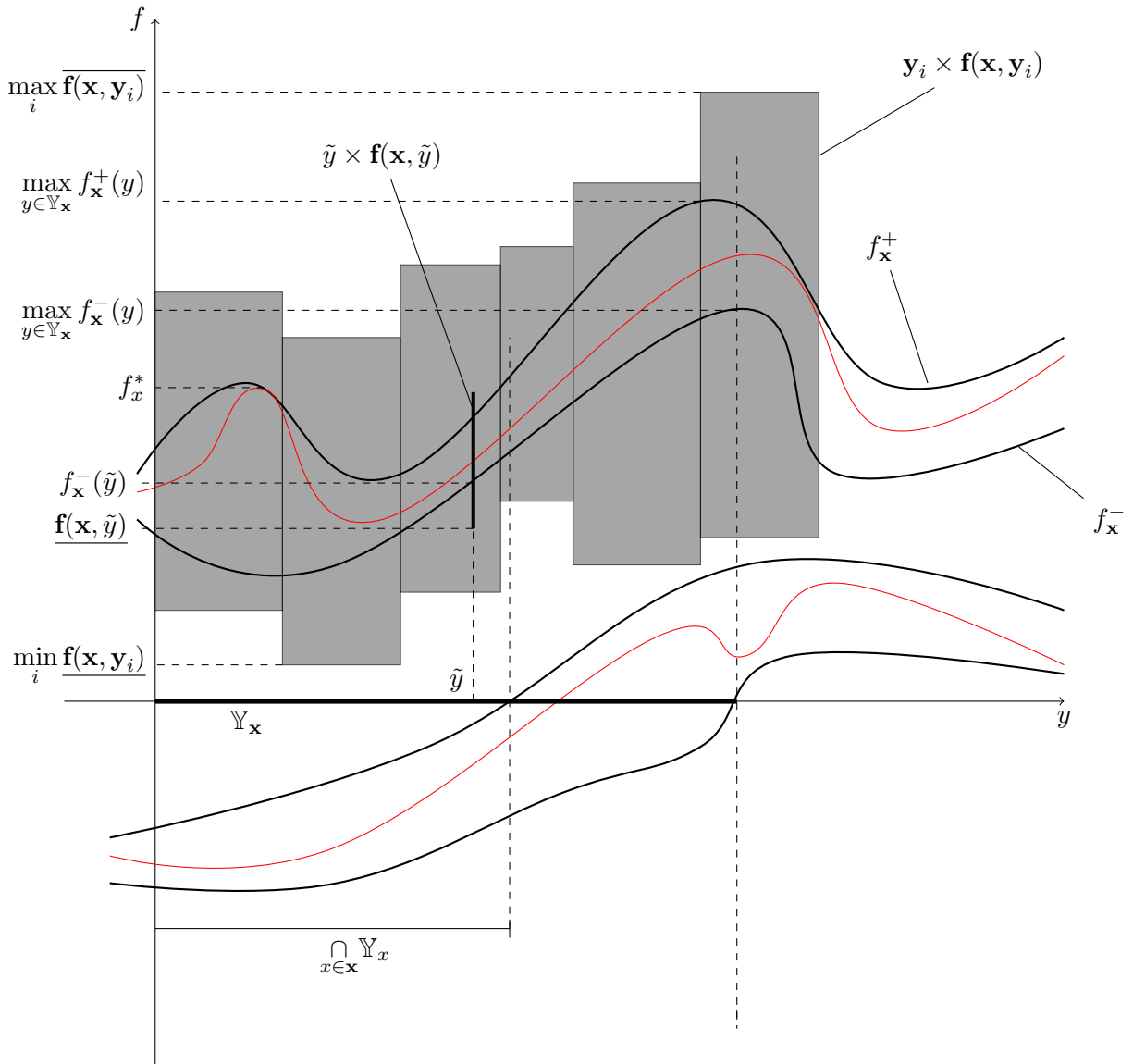
Figure 3.2: Optimization of a family of function with IBBA
