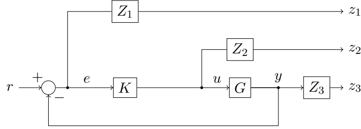
Figure 4.2: Mixed sensitivity problem.
