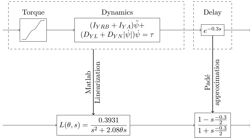
Figure 5.4: Linearization process of the Ciscrea, represented as three non linear blocks.
