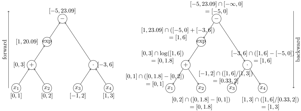
Figure 2.4: Constraint propagation procedure.
