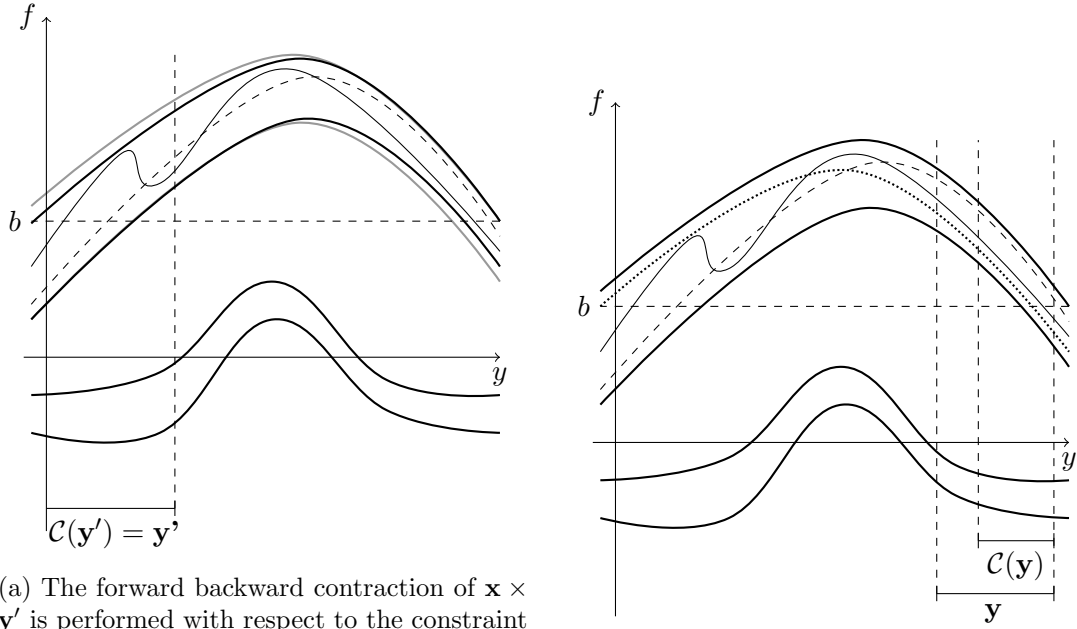
(b) \mathbf{y} is contracted by \mathcal{C} , proving that x^* \notin x . As a consequence, \mathcal{C}_l contracts \mathbf{x} to \emptyset .
