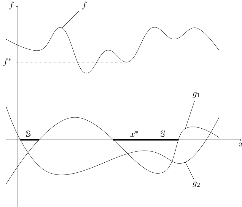
Figure 2.8: Minimization of f subject to the constraints g_1(x) \leq 0 and g_2(x) \leq 0 .
