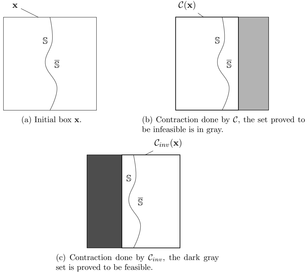
Figure 2.7: Contractions performed by \mathcal{C} and \mathcal{C}_{inv} .
