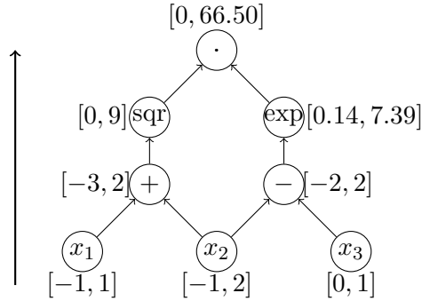
Figure 2.3: Interval computation done by the natural inclusion function of f .
