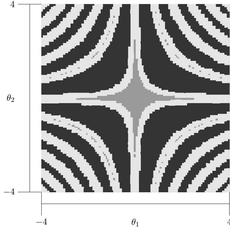
Figure 4.7: Set of parameters for which \|T_{w \rightarrow z_1}\|_\infty is lower than 1, in dark gray, and strictly greater than 1, in gray. Nothing is proved for the light gray set.
