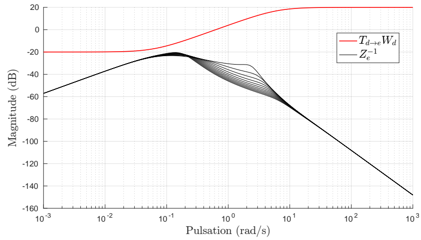
Figure 5.9: Diagram of T_{d \to e} and Z_e^{-1} .
