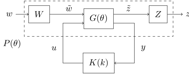
Figure 4.9: General regulation scheme for robust H_\infty synthesis.
