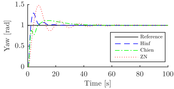
(a) Step response simulation
