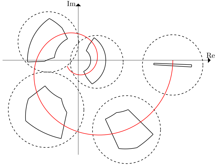
Figure 1.10: The exact regions of the uncertainty are delimited by hard line, and the convex approximations are represented by dashed circle, plotted at 5 pulsations in the Nyquist plan. The red curve represent the nominal system \tilde{P} .
