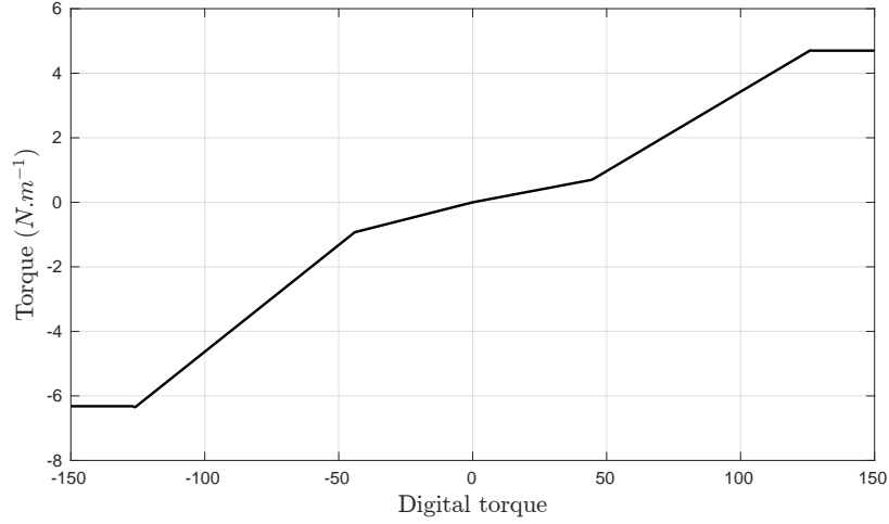
Figure 5.3: Generated torque in Newtons per meters versus digital control.
