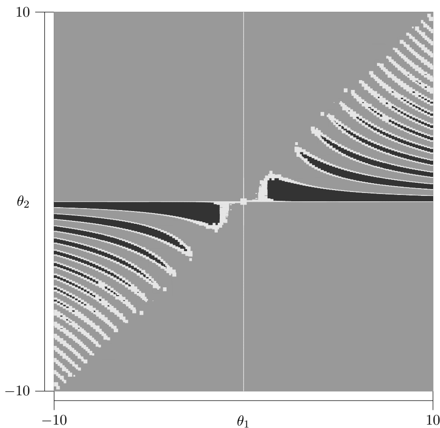
Figure 4.6: Characterization of the stable set of the uncertain parameters.
