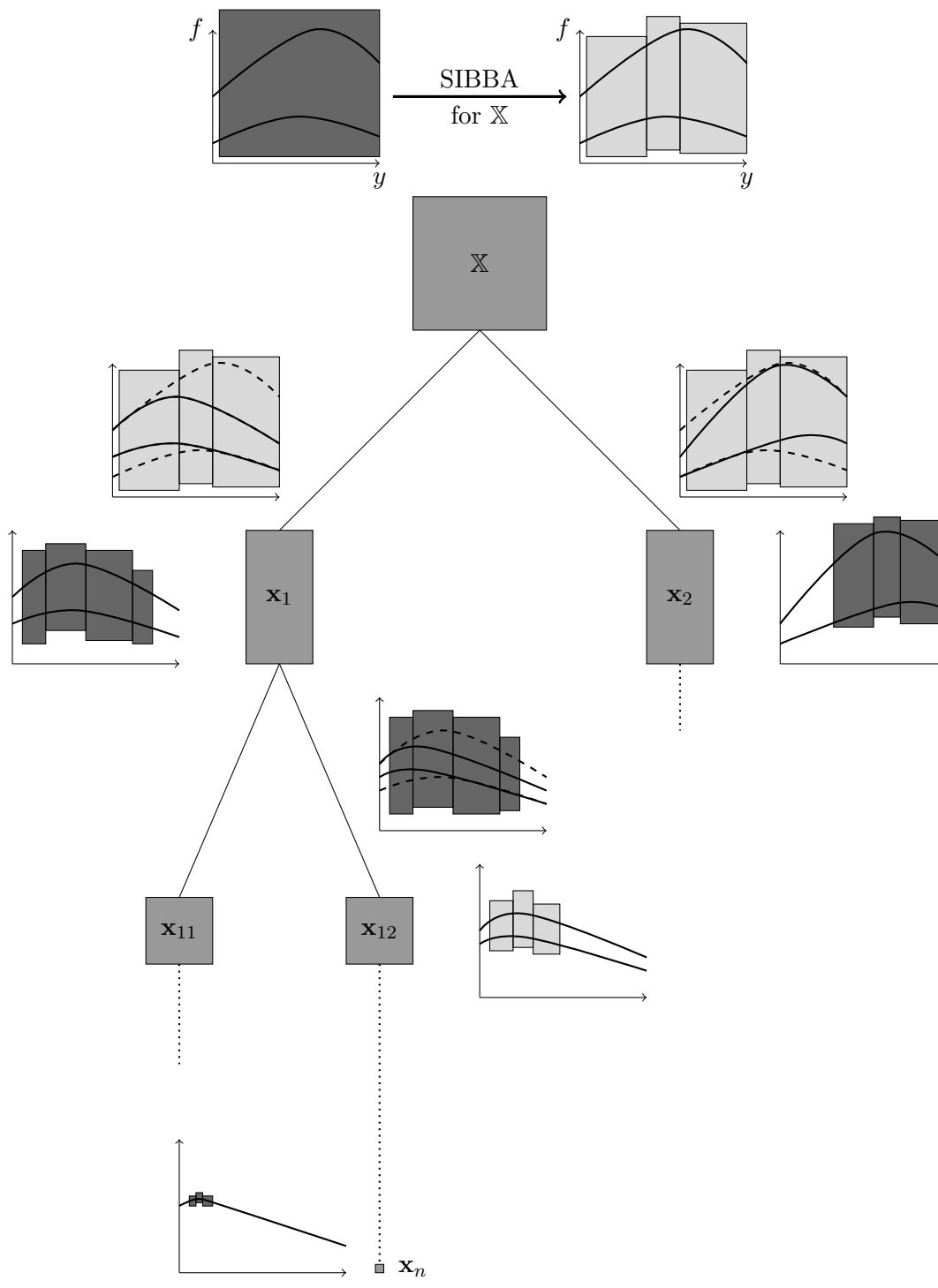
Figure 3.6: Illustration of inheritance strategy in MMIBBA.
