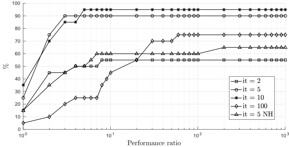
Figure 3.7: Performance profiles of MMIBBA on the minmax problems.
