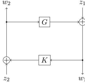
Figure 1.3: Generic regulation scheme for ensuring internal stability.
