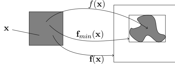
Figure 2.2: Inclusion function \mathbf{f} and minimal inclusion function f_{min}
