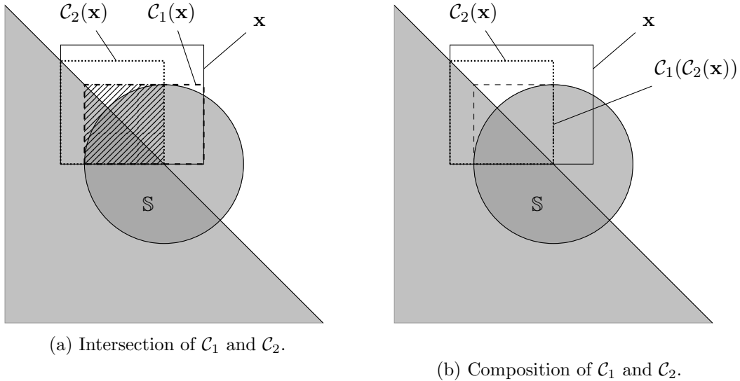
Figure 2.6: Combination of two contractors.
