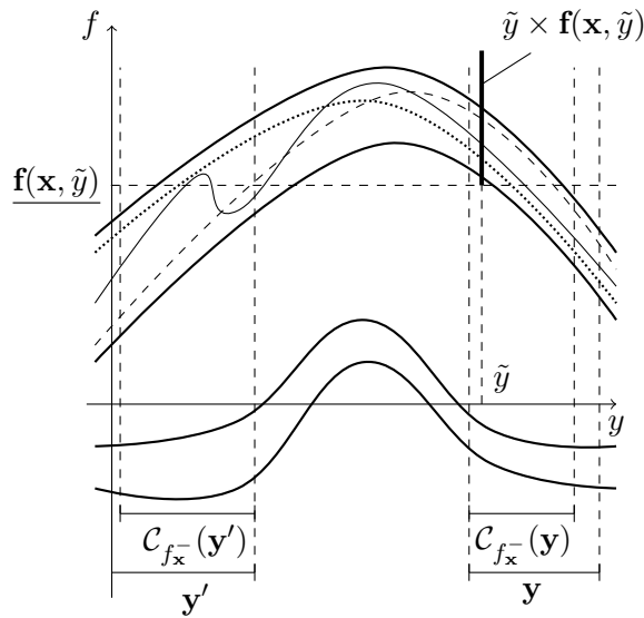
(c) Contraction done by C_{f_{\mathbf{x}}^-} . Subsets of y and y' are discarded for they do not maximize f for any x \in \mathbf{x} .
