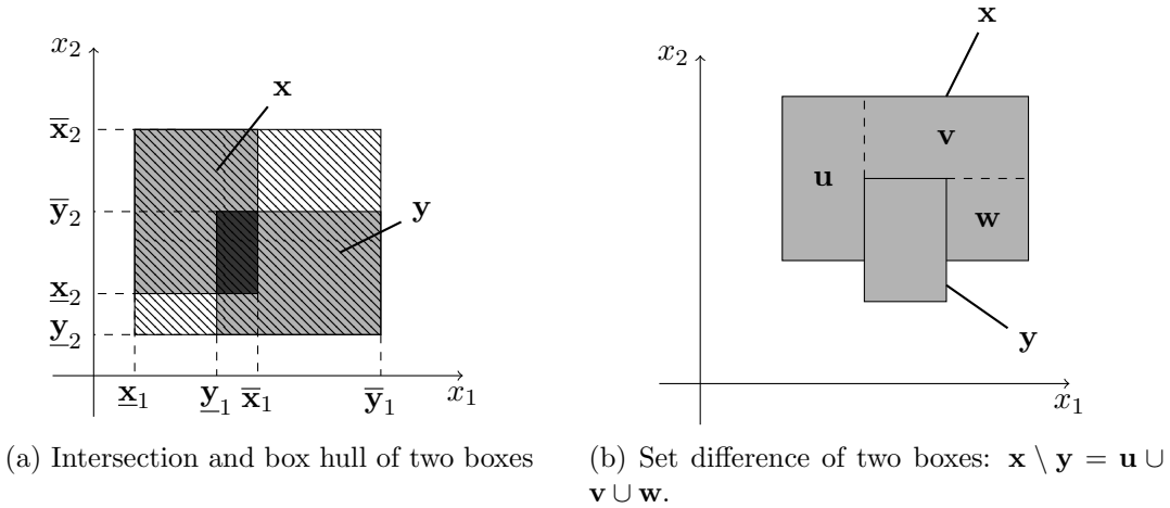
Figure 2.1: Set operations on boxes.
