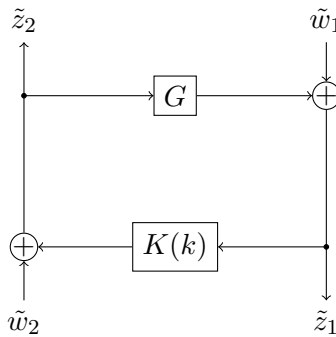
Figure 4.1: Internal stability generic scheme.
