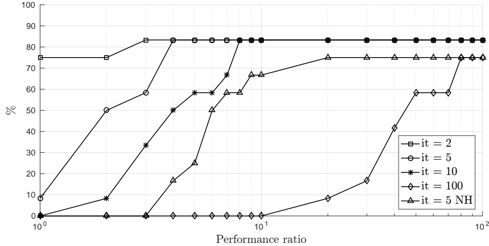
Figure 3.8: Performance profiles of MMIBBA on the SIP problems.
