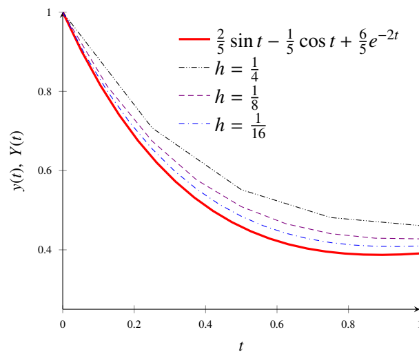
Figure F.4 – Backward Euler’s method approximate solutions of Y'(t) = -2Y(t) + \sin t , Y(0) = 1 for different h values
