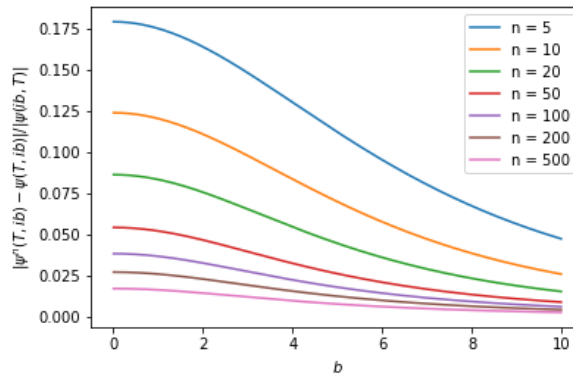
Figure VIII.1 - The relative error \left| \frac{\psi^n(T, ib) - \psi(T, ib)}{\psi(T, ib)} \right| as a function of b under (27) and for different numbers of factors n with T = 1 .
