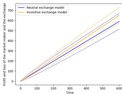
Figure IX.8 - Average total P&L of the exchange and the market maker on [0, T] with 95% confidence interval, with/without incentive policy from the exchange.
