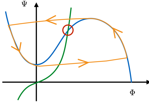
Fig. 2.3 Large-B surge cycle.
