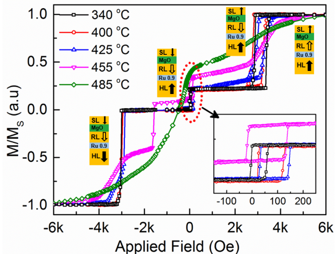
Figure 2.10: Normalized descending branch of out-of-plane M(H) loops of pMTJ stacks at different annealing temperature. The inset shows minor loops of free layer.
