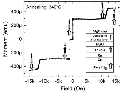
Figure 3.7: Descending branch of M(H) loop of thin-pMTJ stack (Si/Ta 3/Pt 5/[Co 0.5/Pt 0.25] 3 /Co 0.5 /Ru 0.45/FeCoB 1.0/MgO /FeCoB 1.2/W 0.2/FeCoB 0.8/MgO cap/cap layers (thicknesses are in nm)) after annealing at 340°C. The arrows indicate the reversals of different magnetic components of the stack when the field is swept from +16 kOe to -16 kOe..
