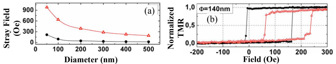
Figure 3.1: (a) Dipolar field as a function of device diameter for a single ferromagnetic hard layer (Ta3/Pt30/(Co0.5/Pt0.4) 5 /Co0.5/ CoFeB1 nm) in red line and perpendicular synthetic antiferromagnetic hard layer (Ta3/Pt30/(Co0.5/Pt0.4) 5 /Co0.5/Ru0.85/(Co0.5/Pt0.4) 3 /Co0.5/CoFeB1 nm) in black. (b) Storage layer hysteresis for two patterned devices showing smaller loop shift in case of SAF hard layer (black loop) compared to single ferromagnetic hard layer (red loop). Figures redrawn from [10].
