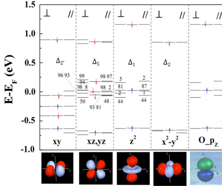
Figure 1.13: Effect of spin-orbit coupling on the orbitals at the interface of Fe/MgO. The three sub columns of every column representing a particular orbital character shows band level for out-of-plane ( \perp , left), in-plane ( \parallel , right) magnetization orientation and for the case of no spin-orbit coupling (middle). Figure adapted from [60].
