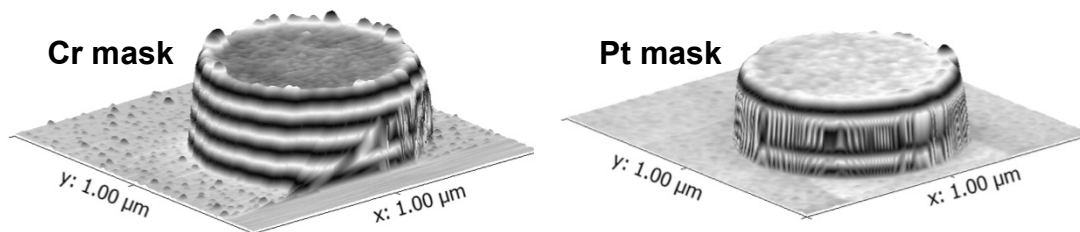
Figure 6.9: AFM images of the Ta pillars with Cr and Pt mask, exhibiting smoother surface profile in case of Pt mask.
