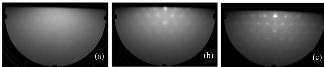
Figure 2.1: RHEED images of 3nm Co_{60}Fe_{20}B_{20} layer deposited on MgO (001) film. (a) as-deposited, and annealed at (b) 360°C and (c) 430°C for 30min. Figures redrawn from Yuasa et al.[1].
