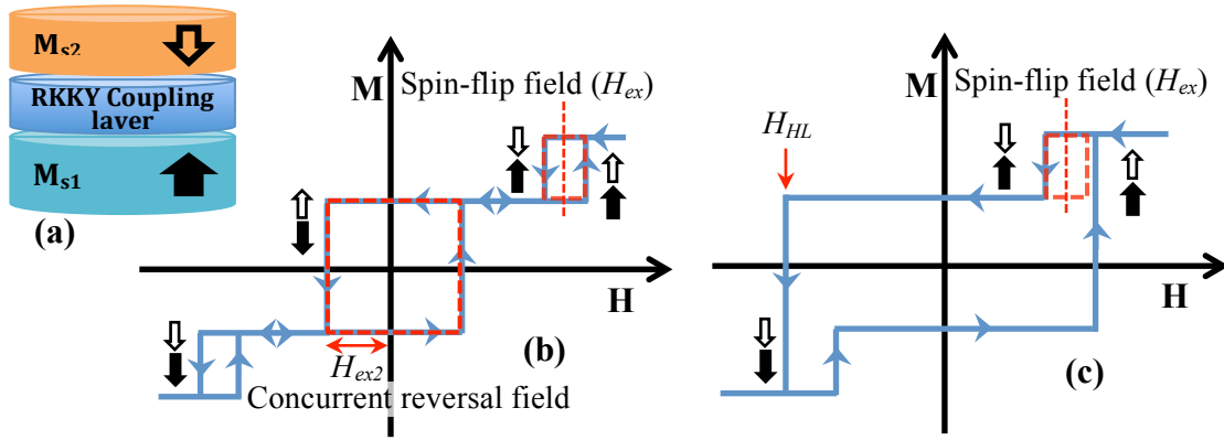
Figure 3.8: (a) Schematics of perpendicular synthetic antiferromagnet consisting of two ferromagnetic layers antiferromagnetically coupled by a RKKY coupling layer. Schematic hysteresis loops of pSAF layers with minor loop of PL for the case (b) H_{ex2} < H_{ex} (Because interlayer exchange coupling energy is larger than the anisotropy energy and the presence of significant Zeeman energy due to imbalance of magnetic moments between PL and HL) and (c) H_{ex2} > H_{ex} (When PMA exceeds interlayer exchange coupling energy and negligible contribution of Zeeman energy)
