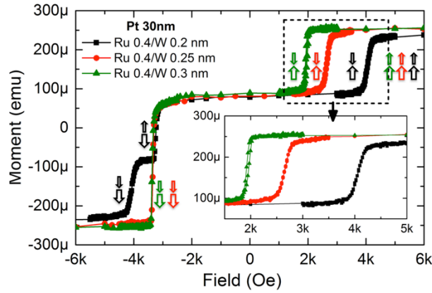
Figure 3.11: Out-of-plane magnetic variation when the field is swept from +6 kOe to -6 kOe of thin-pSAFs. The layer composition of these stacks is Si/SiO_2\ 500/Ta\ 3/Pt\ 30/[Co\ 0.5/Pt\ 0.25]_3/Co\ 0.5/Ru\ 0.4/W(t)/FeCoB\ 1.2/MgO/cap layers (thicknesses are in nm) with different W thickness, t = 0.2, 0.25, 0.3 nm after annealing at 340^\circ C . The arrows of different colors indicate the magnetization reversal processes of corresponding pSAF layers when the magnetic field is swept from +10kOe to -10kOe.
