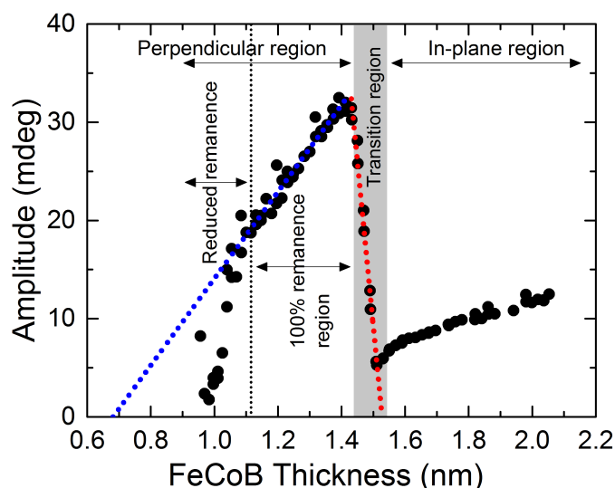
Figure 2.7: Amplitude of Kerr Signal as a function of FeCoB thickness for the stack with W2/Ta1 nm cap after annealing at 425^\circ\text{C} .
