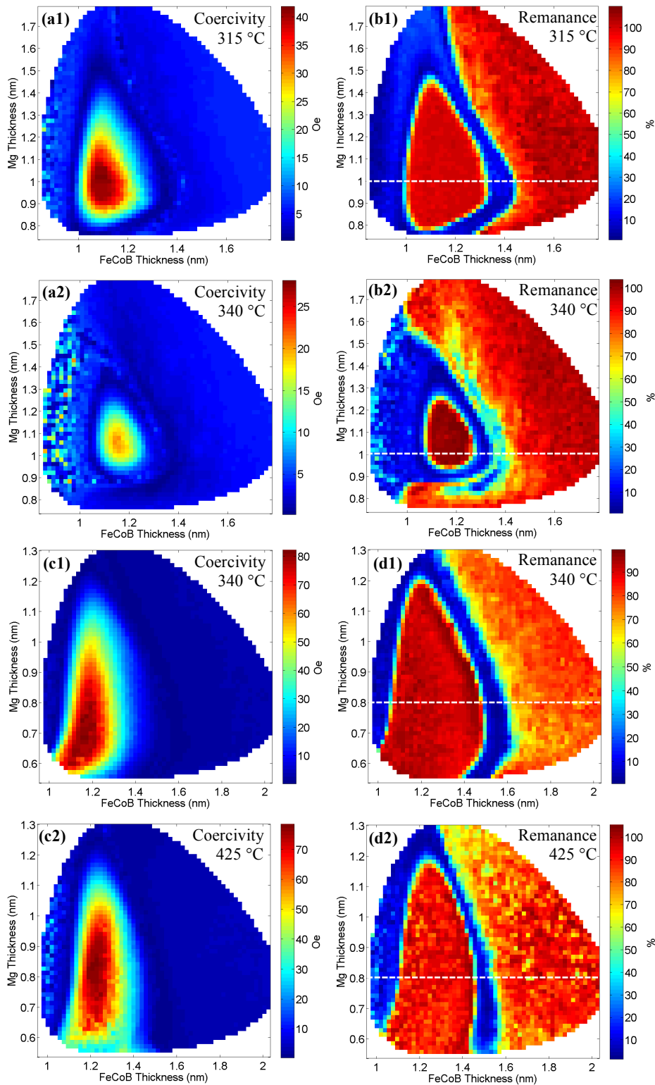
Figure 2.6: Mapping of magnetic properties of half-MTJ stacks as a function of FeCoB and Mg thicknesses across 100 mm Si wafer using MOKE measurement. (a1), (a2) coercivity (b1), (b2) remanance mapping for Ta1nm cap and (c1), (c2) coercivity (d1), (d2) remanance mapping for W2/Ta1nm cap at different annealing temperature.
