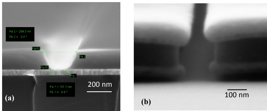
Figure 6.22: SEM images of resist profiles. (a) Resist profile does not show the expected diaphragms due to unoptimized e-beam dose. (b) Two diaphragms, one on top and another in the middle appears for optimized dose.
