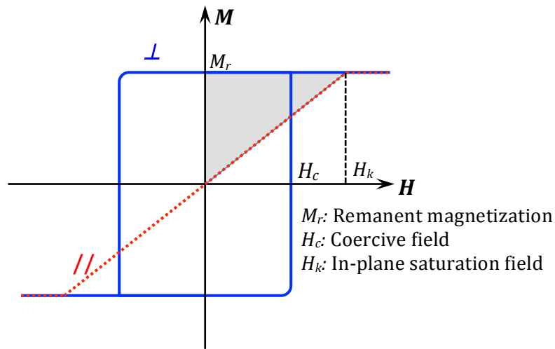
Figure 1.14: Out-of-plane ( \perp ) and in-plane ( \parallel ) M(H) loops of a magnetic thin film, where the magnetic field is applied perpendicular and parallel to the film-plane respectively.
