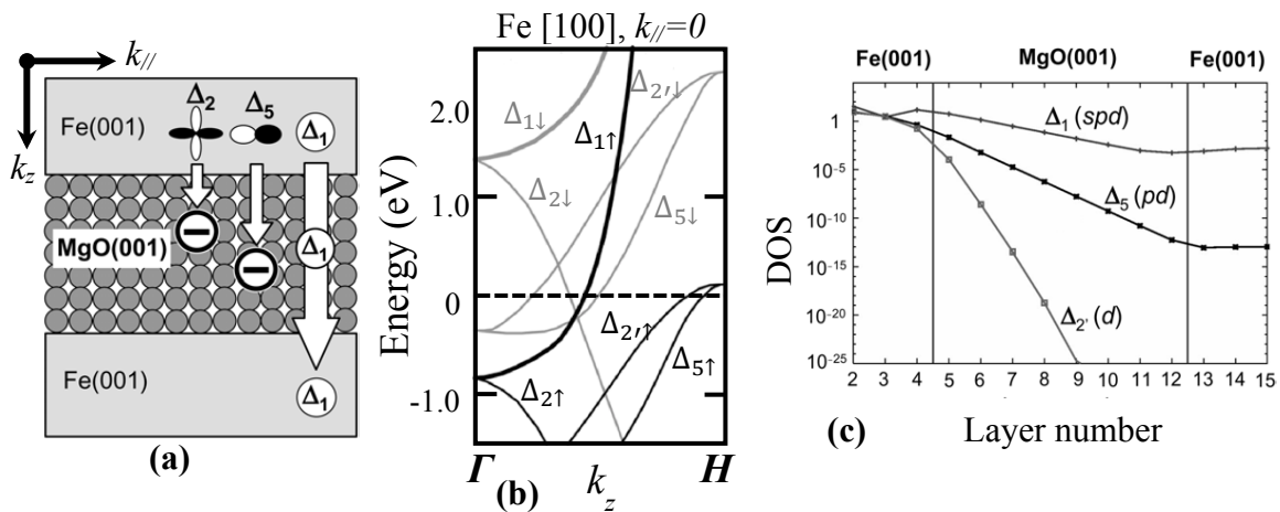
Figure 1.4: (a) Schematic representation of coherent tunneling of electron through crystalline MgO barrier. (b) Majority-spin and minority-spin band dispersion of bcc Fe along [001] direction. (c) Tunneling density of states (DOS) of majority-spin states for k_{||}=0 in Fe (001)/MgO(001)/Fe(001) with parallel magnetization orientation. Figures redrawn from Yuasa et al. [12].
