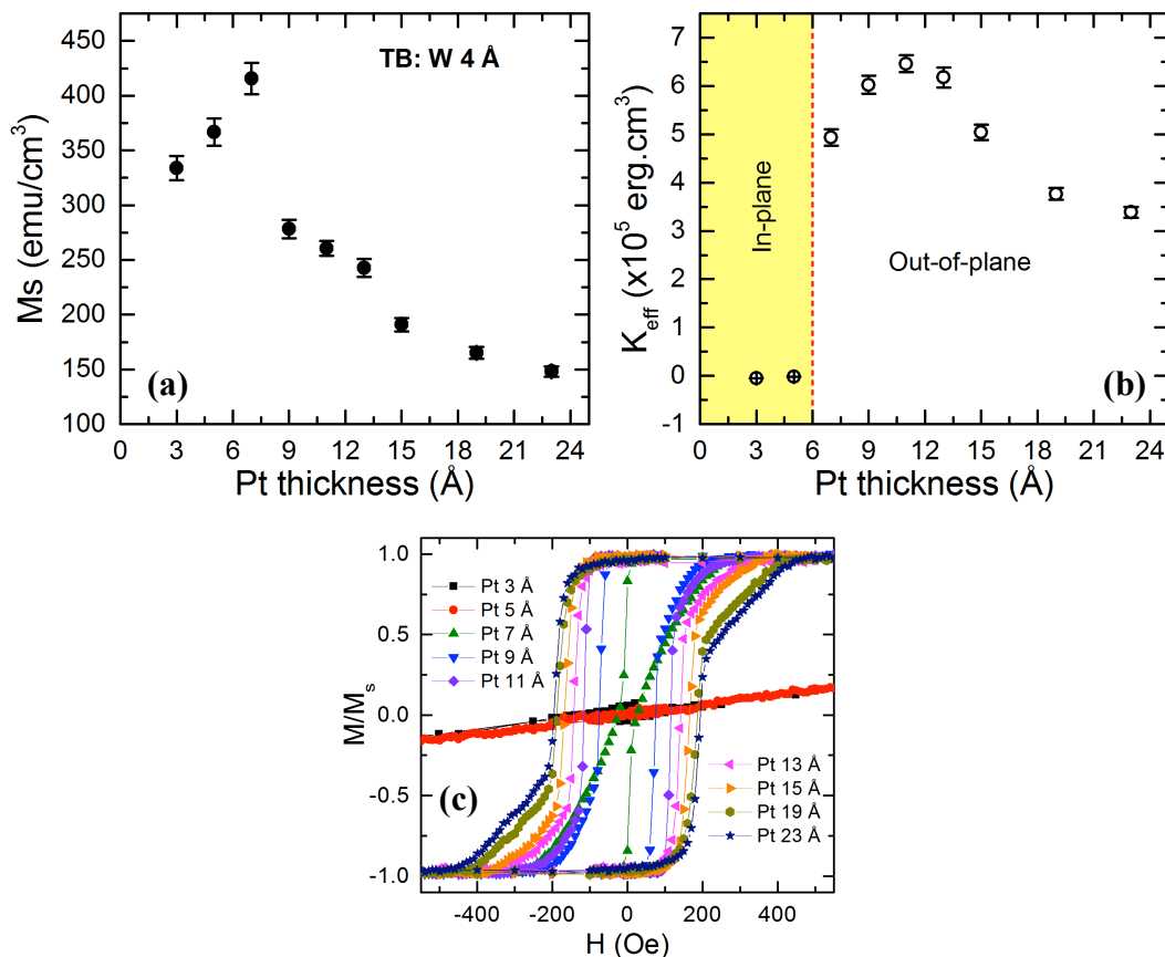
Figure 5.7: (a) M_s , (b) K_{\text{eff}} and (c) out-of-plane magnetic loops of (MgO/FeCoB 1.1/ W 0.5/[Co 0.6/Ta 0.2/Pt (t)] 5 /Ru 5 nm) MLs as a function of Pt thickness after annealing at 400°C.
