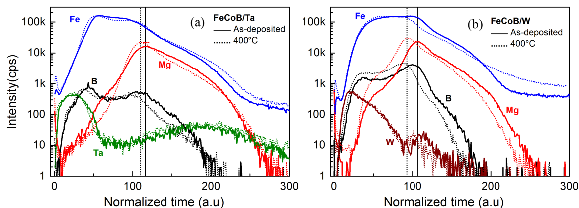
Figure 2.9: SIMS depth profile of half-MTJ stacks ( \text{Si}/\text{MgO} \sim 1/\text{FeCoB} 1.6/\text{cap} 2/\text{Pt} 3 \text{ nm} ) with (a) Ta 2 nm cap and (b) W 2 nm cap layers. Solid and dotted lines represent as-deposited and 400 °C annealed samples respectively.
