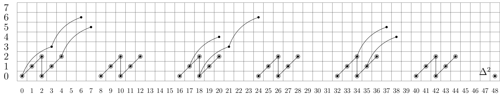
Figure III.6 – E_\infty -term of the HFPSS for E_C^{hC_6} \wedge V(0) . A circled black dot represents a copy of \mathbb{F}_4[[u_1^3]] and a black dot a copy of \mathbb{F}_4 . A curved line represents multiplication by \nu and a line of slope 1 multiplication by \eta , a vertical line multiplication with 2. The E_\infty -term is 48-periodic by multiplication by \Delta^2
