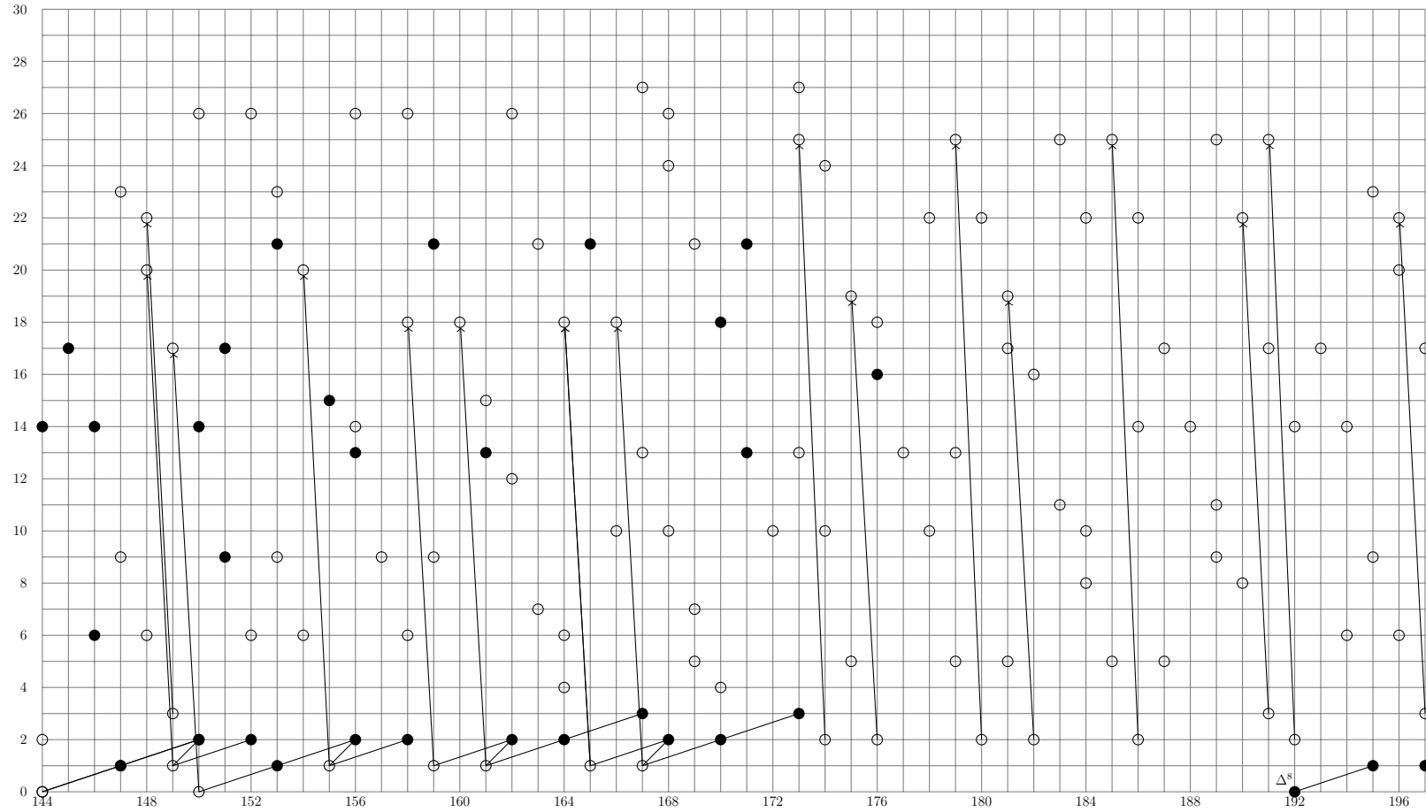
Figure II.29 – HFSS for A_1[00] and A_1[11] from E_7 -term with 144 \leq t - s \leq 197
