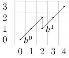
Figure II.2 – \text{Ext}_{\mathcal{A}(1)_*}^{s,t}(\mathbb{H}_*(V(0))) in the range 0 \leq t - s \leq 4 .
