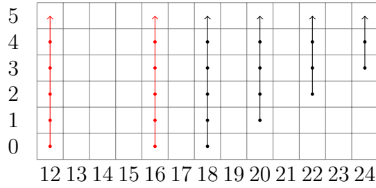
Figure II.11 – G_3 -The red part is the contribution of \text{Ext}_{\mathcal{A}(1)_*}^{s,t}(\mathbb{R}_3/\Sigma^{18}\mathbb{H}_*(C_\eta)) and the black one of \text{Ext}_{\mathcal{A}(1)_*}^{s,t}(\Sigma^{18}\mathbb{H}_*(C_\eta)) .
