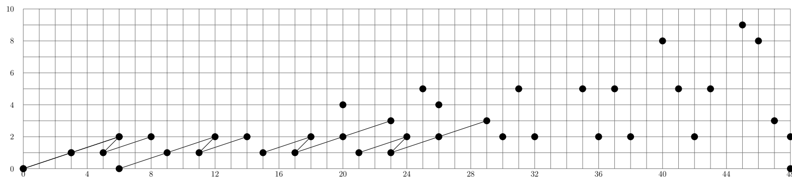
Figure II.26 – HFPSS for A_1[00] and A_1[11] from E_7 -term with 0 \leq t - s \leq 48
