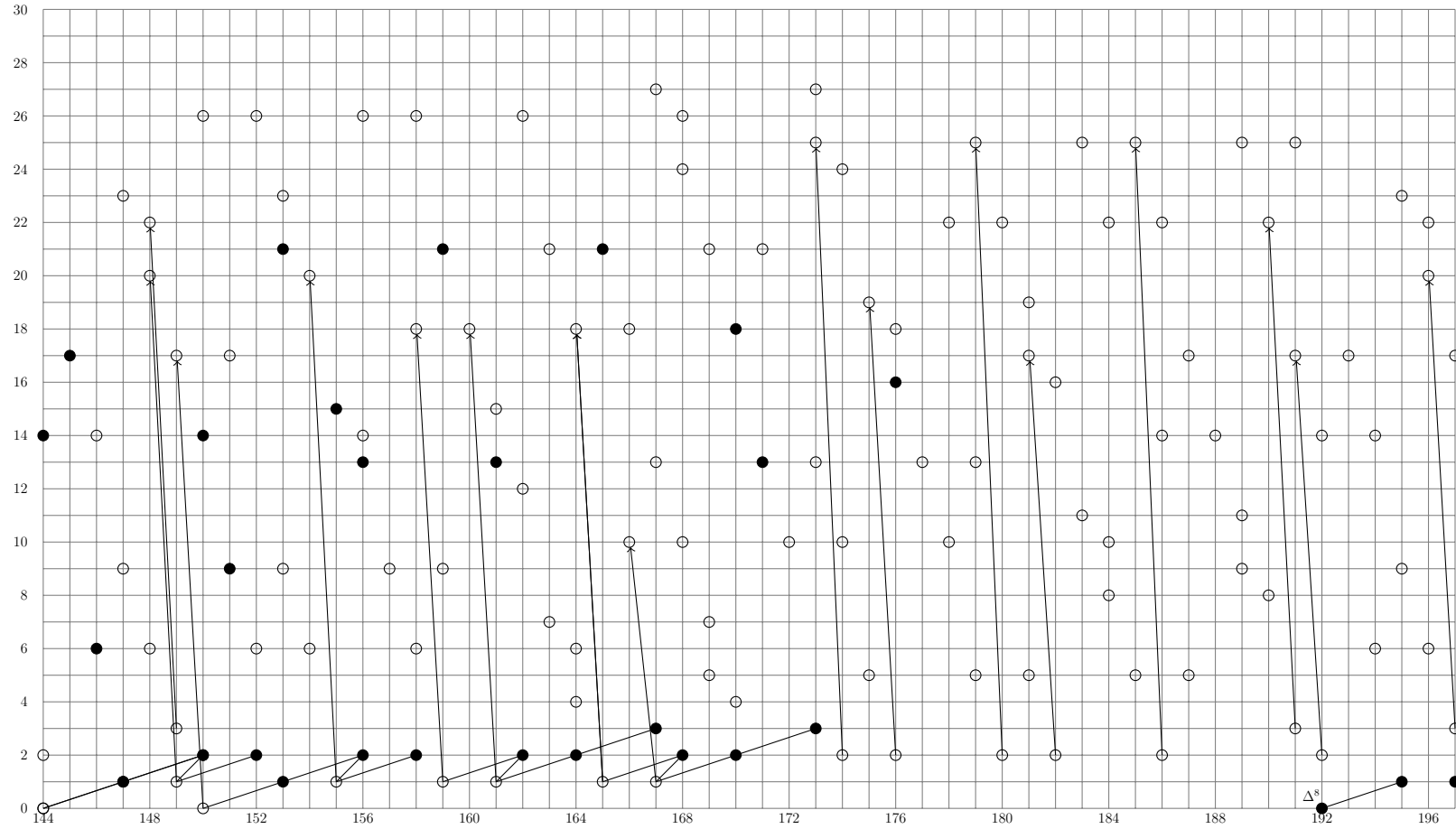
Figure II.25 – HFPSS for A_1[10] and A_1[01] from E_7 -term with 144 \leq t - s \leq 197
