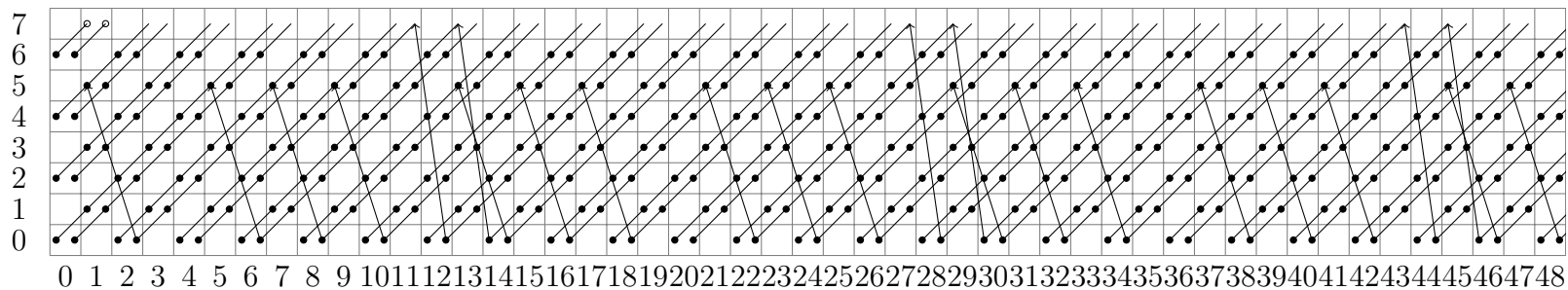
Figure III.9 – The E_2 -term of the HFPSS for E_C^{hC_2} \wedge A_1 and the differentials d_5 and d_7 . A black dot represents a copy of \mathbb{F}_4 and straight line a multiplication with t .
