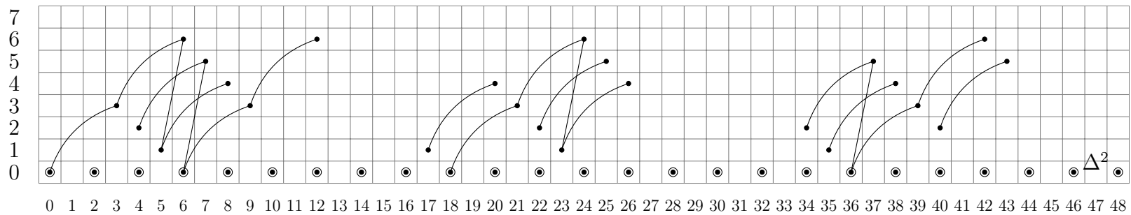
Figure III.8 – E_\infty -term of the HFPSS for E_C^{hC_6} \wedge Y . A circled black dot represents a copy of \mathbb{F}_4[[u_1^3]] and a black dot a copy of \mathbb{F}_4 . A curved line represents multiplication by \nu and a straight line multiplication by \eta . The E_\infty -term is 48-periodic by multiplication by \Delta^2 .
