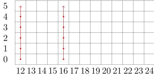
Figure II.10 – \text{Ext}_{\mathcal{A}(1)_*}^{s,t}(\mathbb{R}_3/\Sigma^{18}\mathbb{H}_*(C_\eta)) .
