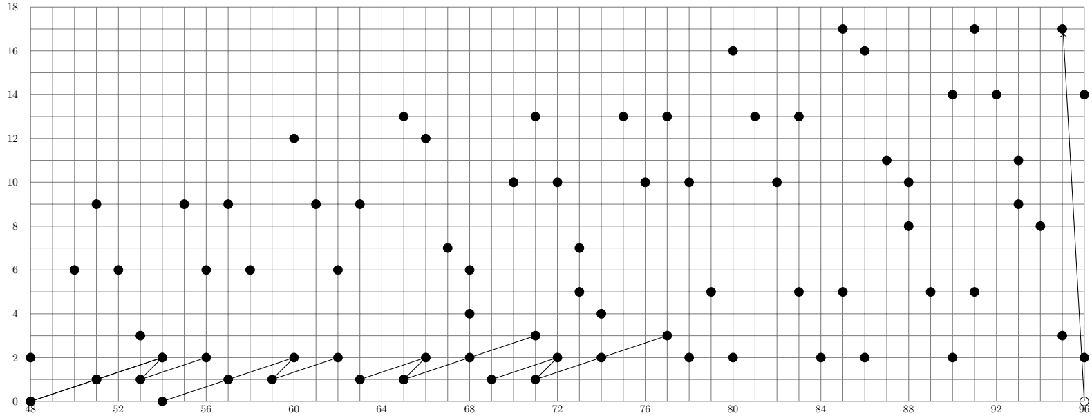
Figure II.27 – HFSS for A_1[00] and A_1[11] from E_7 -term with 48 \leq t - s \leq 96
