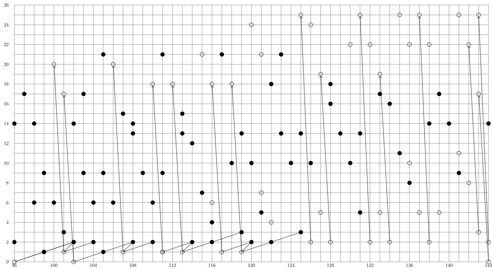
Figure II.28 – HFPS for A_1[00] and A_1[11] from E_7 -term with 96 \leq t - s \leq 144
