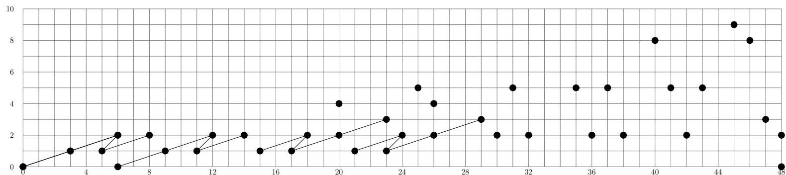
Figure II.22 – HFPSS for A_1[10] and A_1[01] from E_7 -term with 0 \leq t - s \leq 48
