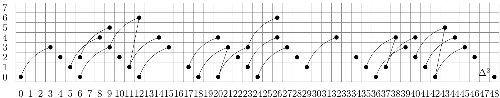
Figure III.10 – E_\infty -term of the HFPSS for E_C^{hC_6} \wedge A_1 . A black dot represents a copy of \mathbb{F}_4 . A curved line represents multiplication by \nu , a straight line multiplication by \eta . The E_\infty -term is 48-periodic by multiplication by \Delta^2 .
