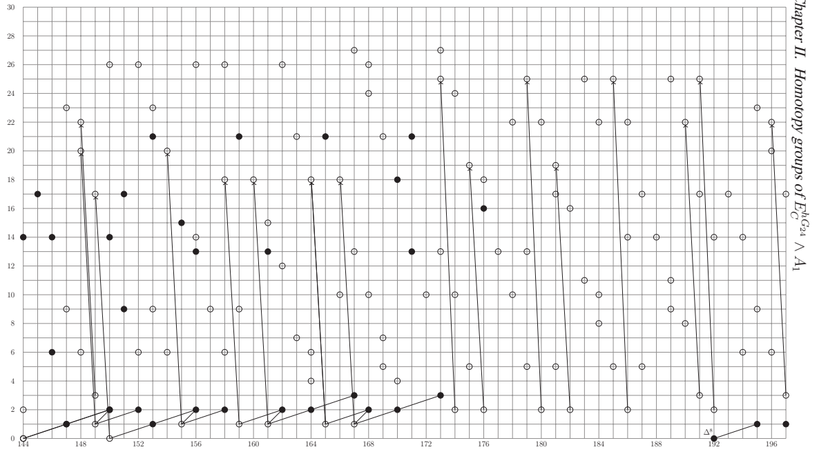
Figure II.29 – HFPS for A_1[00] and A_1[11] from E_7 -term with 144 \leq t - s \leq 197
