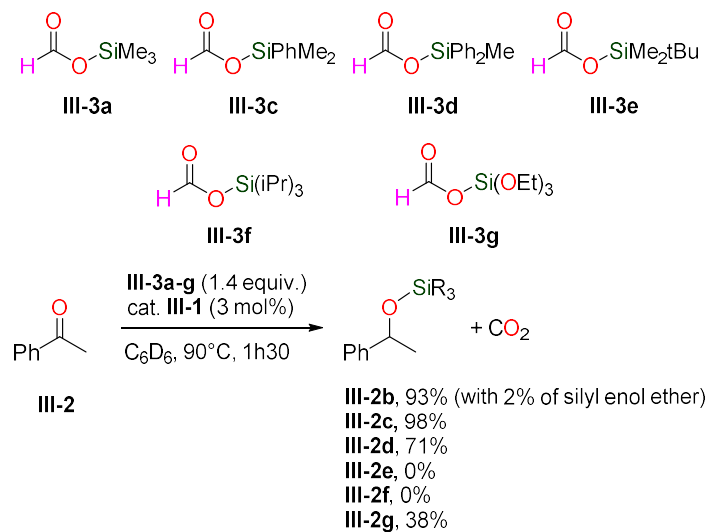
Figure V-52: Scope of the silyl formates in transfer hydrosilylation of acetophenone III-2 . Reaction conditions: acetophenone III-2 (0.1 mmol); silyl formate (0.14 mmol); complex III-1 (3 mol%); \text{C}_6\text{D}_6 (0.4 mL; 0.2 M); 1h30 at 90 °C. Yields determined by ^1\text{H} NMR analysis using mesitylene (10 \mu\text{L} ) as an internal standard.
