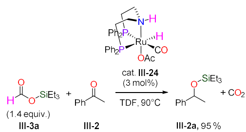
Figure V-69: Test of activity of the ruthenium complex [(PNP)Ru(H)(CO)(OAc)] on the transfer hydrosilylation of acetophenone.
