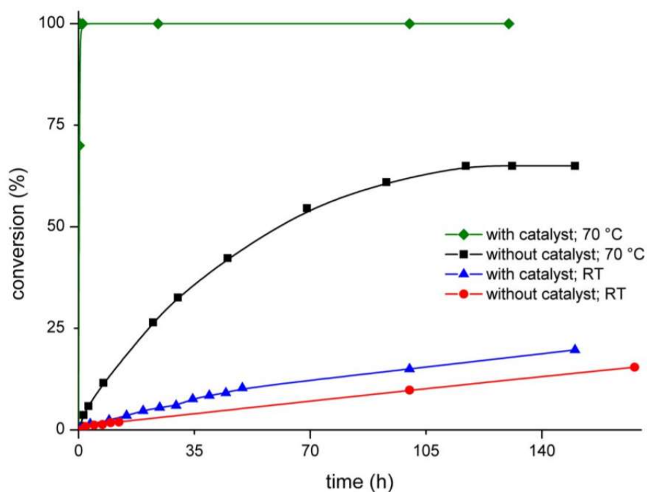
Figure V-18: Influence of the temperature and the catalyst on the equilibrium between silylformates and silylethers
