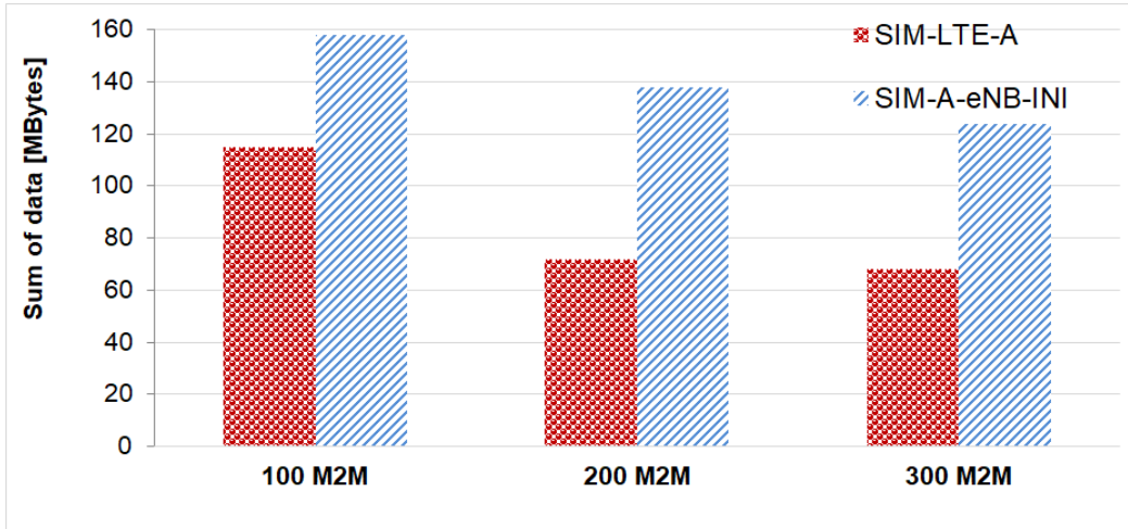
Figure 4-6: FTP-DL improvement in LTE-M comparing to LTE-A., where SIM-LTE-A represents the results in a regular eNodeB/LTE-A and SIM-A-ENB-INI is the results during an initial stage of the A-eNB/LTE-M.
