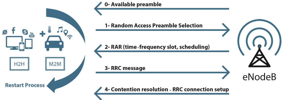
Figure 3-4: Contention-based RACH procedure.
