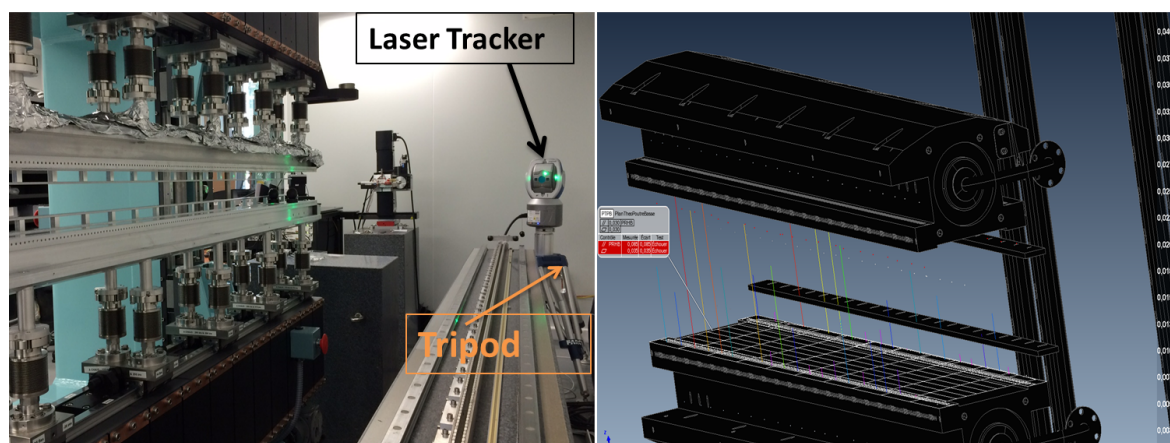
Figure 4.13: FARO Laser Tracker Vantage held on a tripod measures the position of the girders and displays them with Innovmetric Polyworks (figure on the right).
