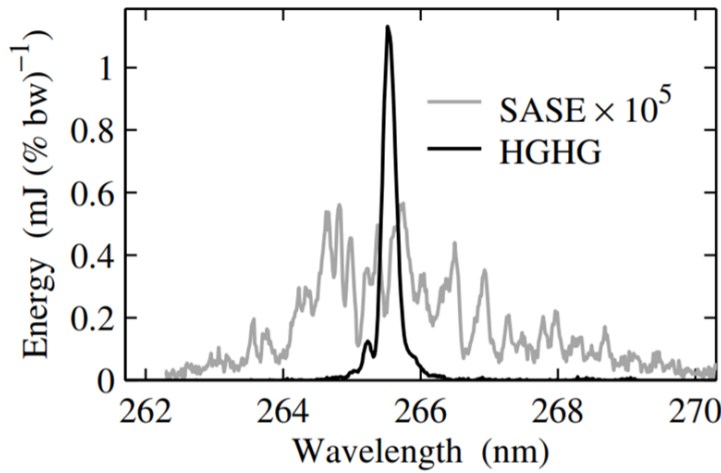
Figure 1.10: Single shot HGHG spectrum using a 800 nm laser seed compared with a SASE shot. Figure from [122].
