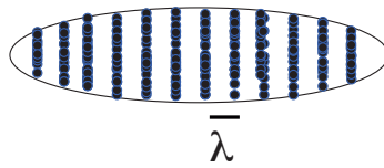
Figure 2.18: Schematic representation of the slices of length \lambda along a bunched electron beam.
