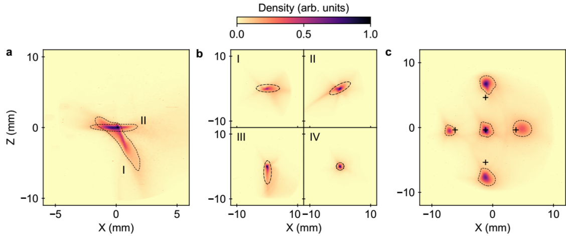
Figure 7.21: Super-imposed images with the appropriate adjustment of the QUAPEVAs magnetic axis. (a) Case of screen in the middle of the chicane where the beam is horizontally dispersed, correction of the vertical dispersion (from I to II ) (b) Screen located at the undulator entrance: initial beam I , with artificial vertical dispersion introduced II , with horizontal dispersion corrected III , with artificial vertical dispersion removed IV . (c) Beam experimental transverse position control with respect to expected displacements from the model (black crosses).
