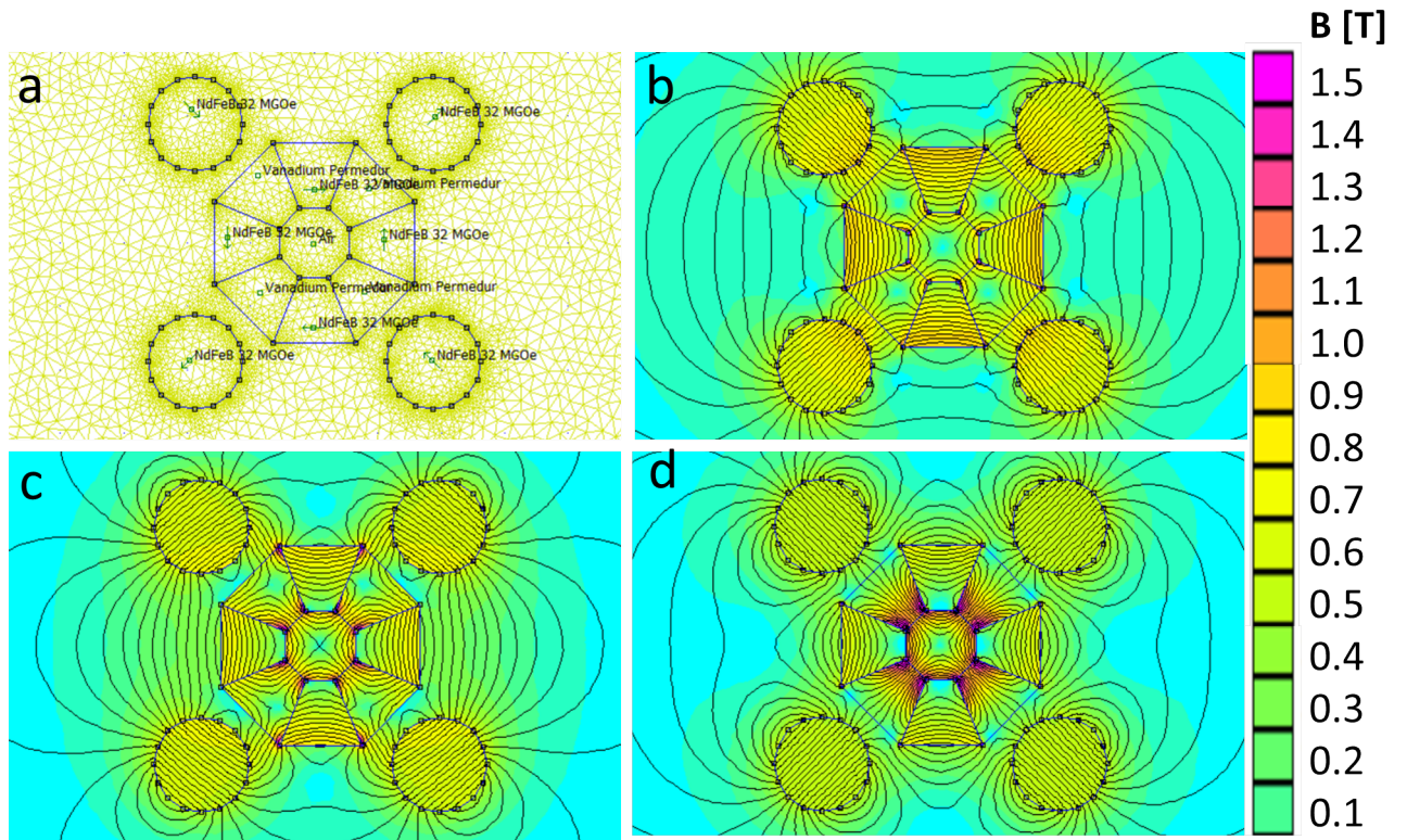
Figure 5.21: (a) QUAPEVA model using FEMM software alongside the field lines produced for the minimum (b), average (c) and maximum (d) gradients. Magnets: Nd 2 Fe 14 B 32MGoe, poles: Vanadium Permendur. Core and the surrounding is air medium.
