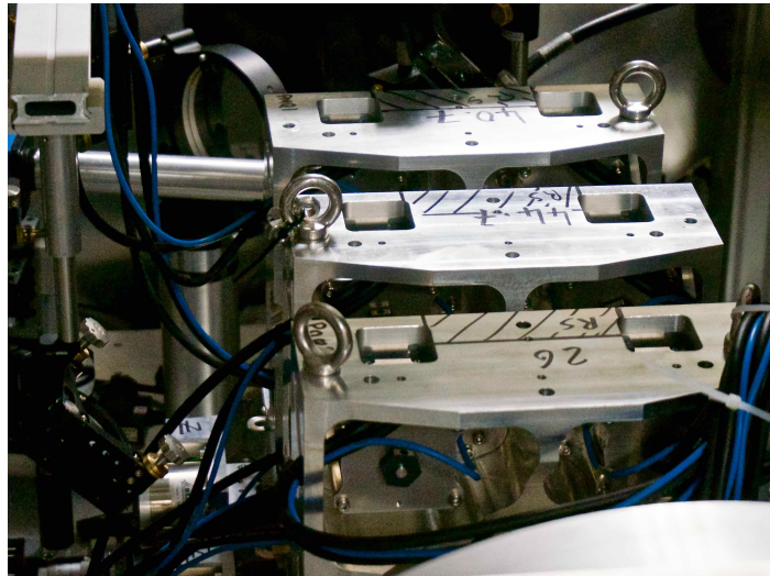
Figure 7.5: QUAPEVA triplet installed at COXINEL beam line in the laser chamber.
