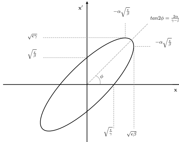
Figure 2.2: Phase space with the ellipse containing all the particles.
