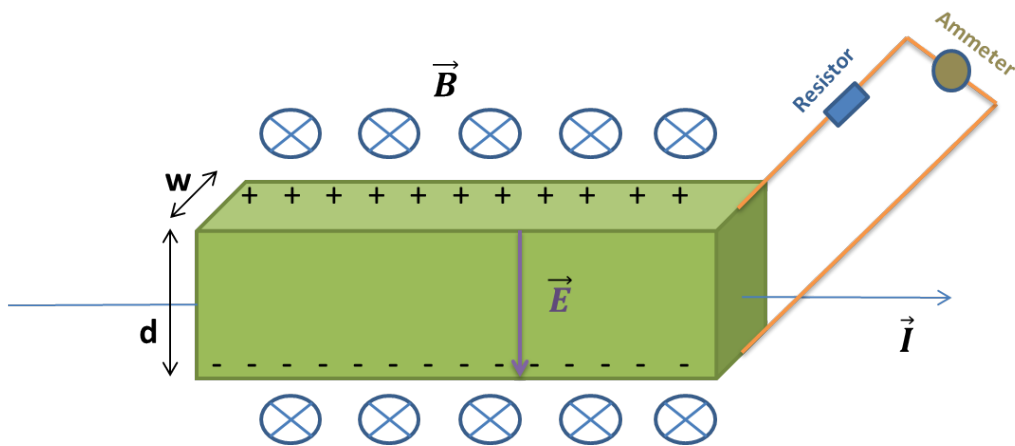
Figure 4.11: Schematic view of the physical concept behind the Hall probe. 'd' and 'w' are the thickness and width of the rod respectively, E the electric field induced, B the magnetic field, and I the current traversing the rod.
