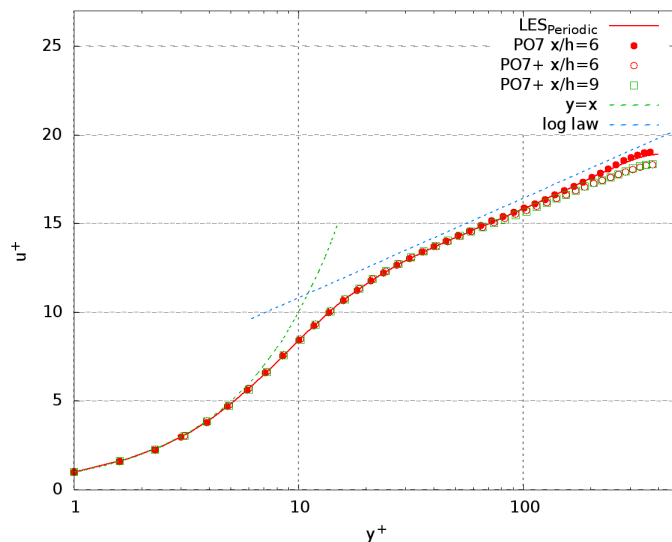
Figure 3.37: Mean velocity profile of PO7 (at x/h = 6 ), PO7+ (at x/h = 6 and x/h = 9 ): symbol, LES with improved vortex method; line, reference periodic LES
