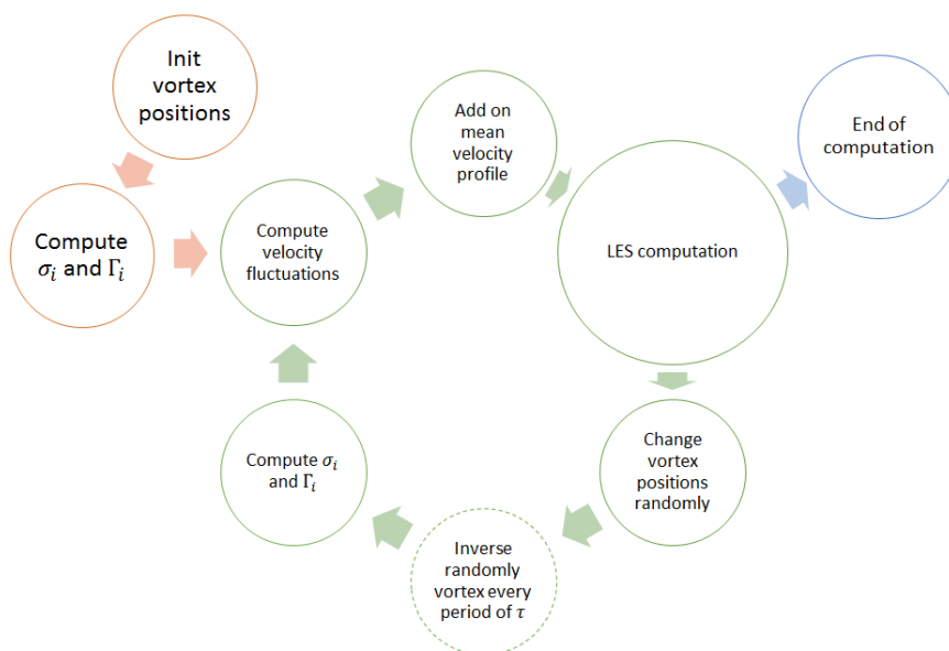
Figure 2.4: Flowchart of vortex method ([Sergent, 2002])
