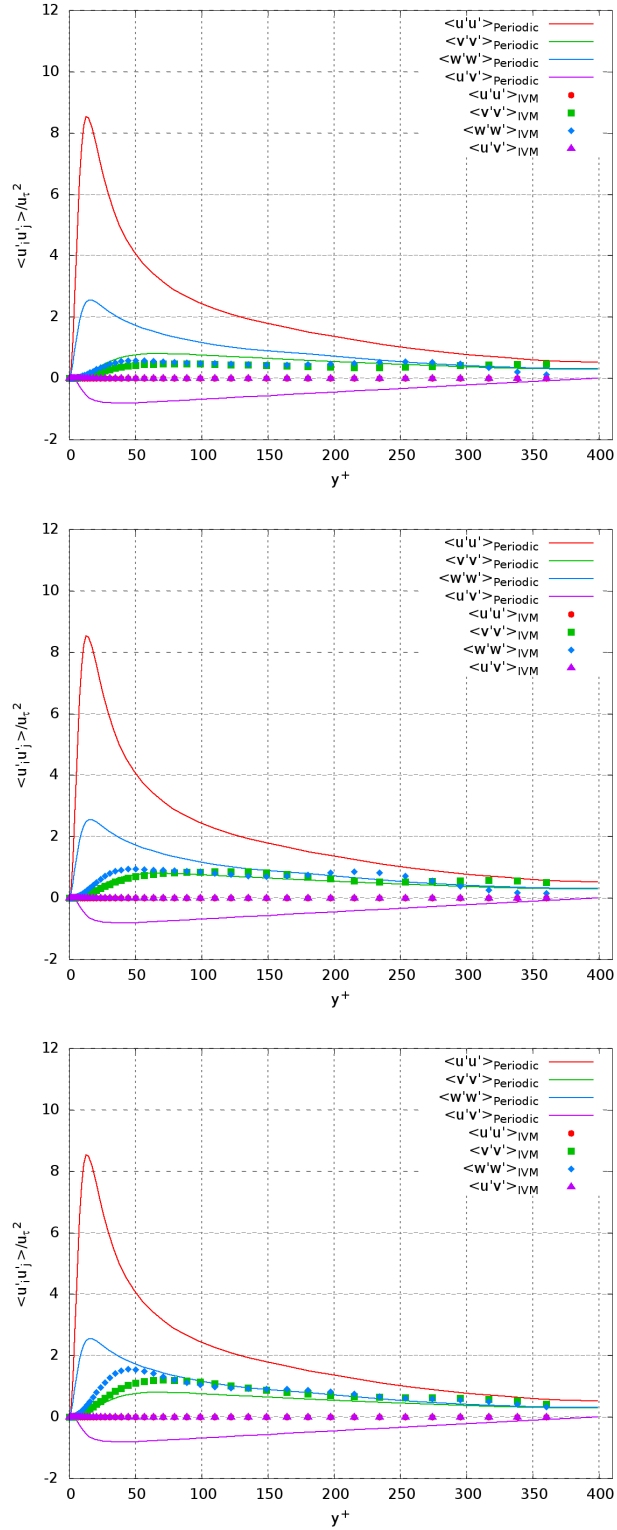
Figure 3.30: Reynolds stresses at inlet x/h = 0 of PO12 (top), PO13 (mid), PO14 (bottom): symbol, LES with improved vortex method; line, reference periodic LES
