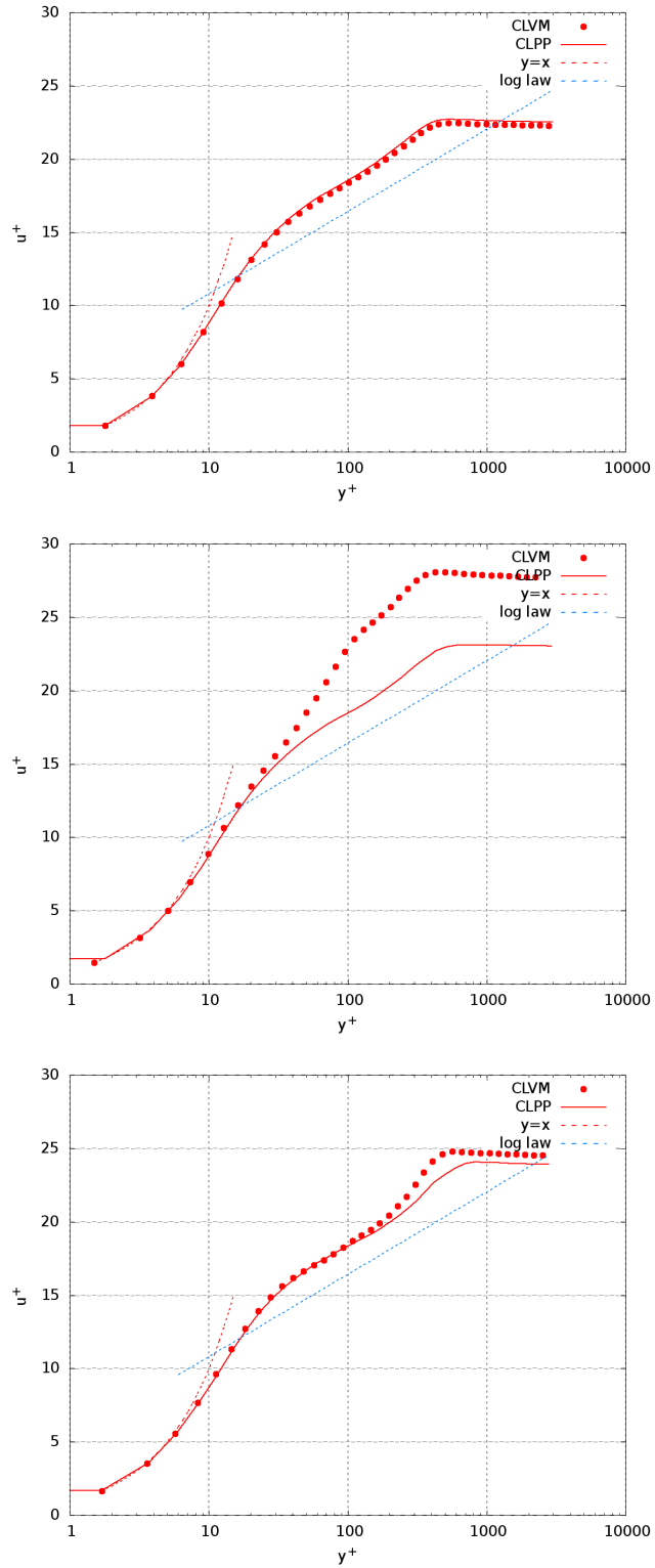
Figure 4.21: Mean velocity profile at x = 0.1243 (top), x = 0.1543m (mid) and x = 0.175m (bottom): symbol, LES with improved vortex method - CLVM; line, reference LES - CLPP
