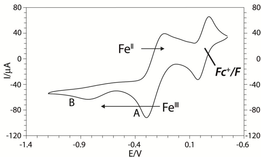
Figure 12: Cyclic voltammogram of 2 FeCl 3 and H 4 L 10 mM in DMF (TBA(PF 6 ) = 0.15 M). Working electrode glassy carbon; \nu = 0.1 \text{ V s}^{-1} .
