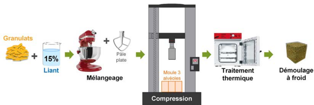
FIGURE 5.1 – Fabrication des composites.
