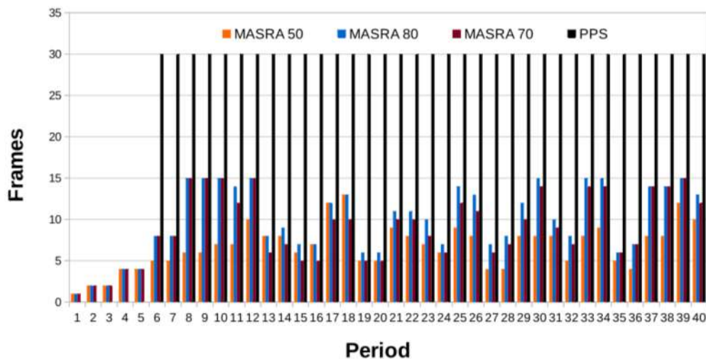
Figure 4.10: Difference between MASRA and PPSS on the transmission phase
