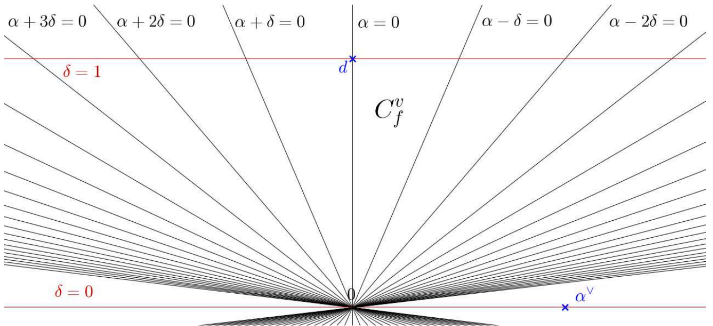
Figure 3.4.2 – Vectorial apartment of \widetilde{\mathrm{SL}}_2 with forty-one walls
