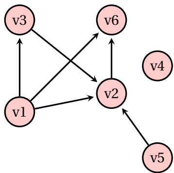
Proportion N1: 19.8%
