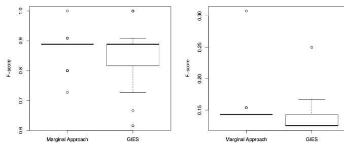
FIGURE 3.7 – F-score of the marginal causal approach and GIES algorithm. The F-score is based on downstream (left) or not-downstream (right) links. For the marginal approach, a hard threshold of -0.5 is used for the \log_{10} Bayes factor to select between models. For the GIES algorithm, the inferred topology is used to classify nodes as downstream or not.
