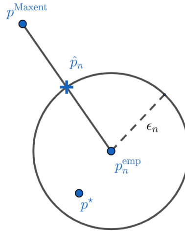
Figure 4.2 – Barycenter between experts and data.
