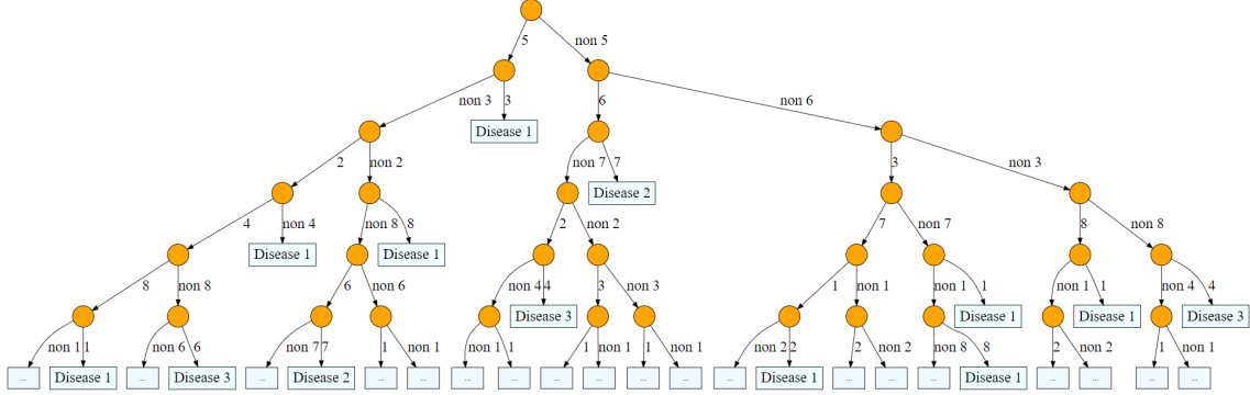
Figure 3.3 – Optimal decision tree for a subtask with 8 possible symptoms.
