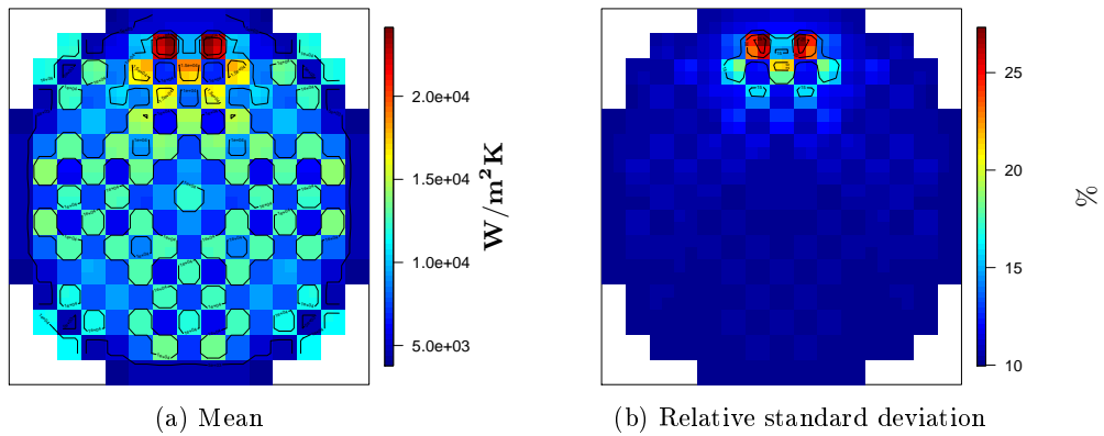
Figure F.24: H_{gap}^{3D} estimated mean and relative standard deviation in the radial cross-section at Z30 for IBE with 3D and finer discretized thermal-hydraulic channels coupling study in PWR core.
