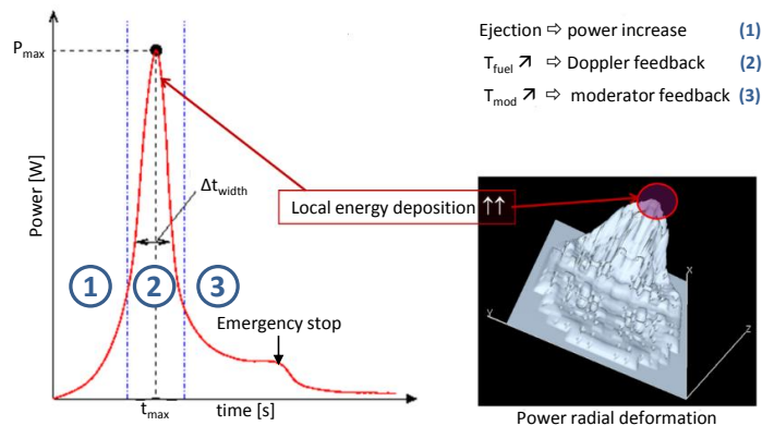
Figure 1.14: Power evolution during REA.
