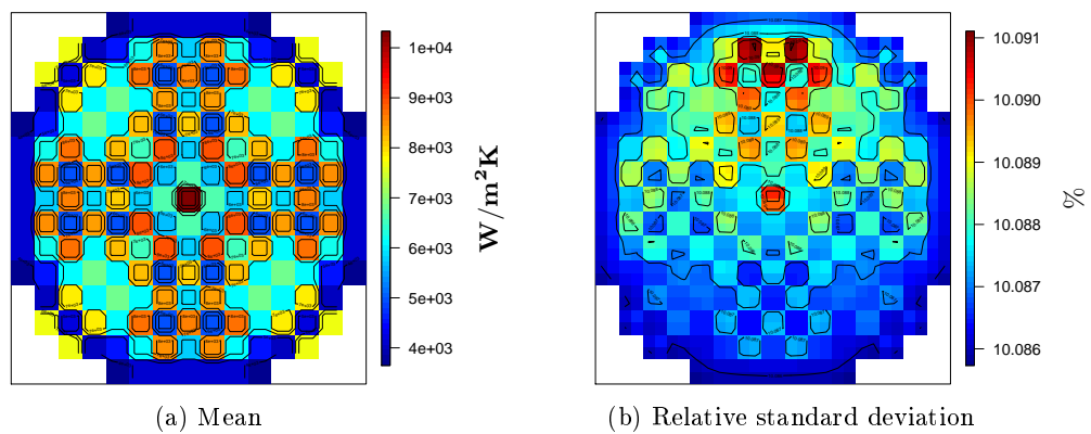
Figure F.20: H_{gap}^{3D} estimated mean and relative standard deviation in the radial cross-section at Z1 for IBE with 3D and finer discretized thermal-hydraulic channels coupling study in PWR core.
