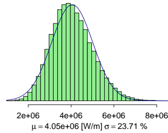
Figure D.1: Estimated histogram of P_{lin}^{max} for point kinetics study.
