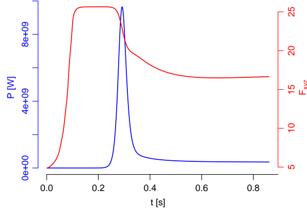
Figure 4.6: Integral power and F_{xyz} deformation factor evolution for the reference REA in the PWR core.
