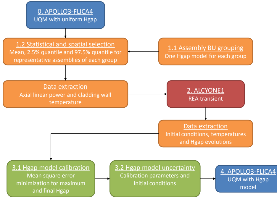
Figure 3.30: Gap heat transfer model calibration methodology scheme.
