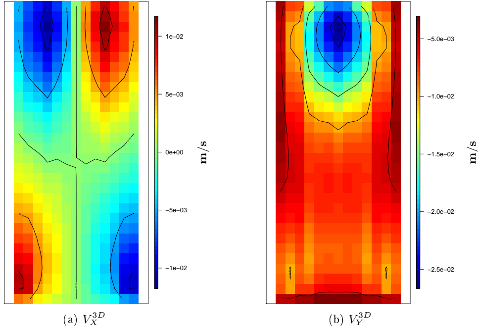
Figure 4.34: V_X^{3D} and V_Y^{3D} estimated mean distribution in the axial cross-section for 3D IBE coupling study.
