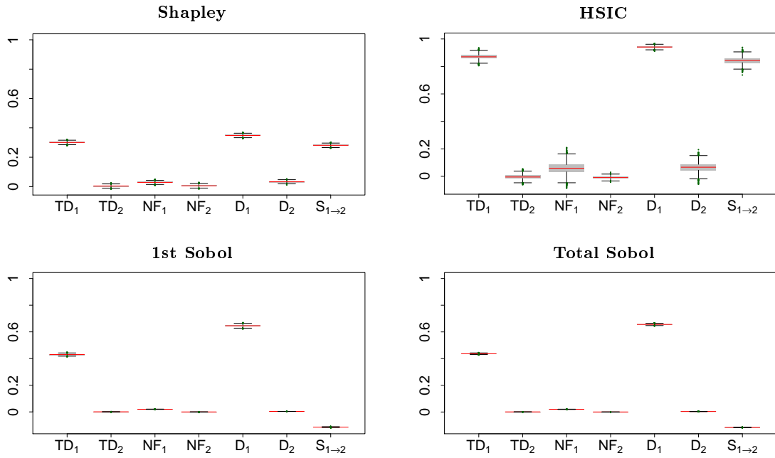
Figure 3.10: F_{xyz}^{\text{ej}} sensitivity analysis results for neutronics stand-alone static study in the MiniCore.
