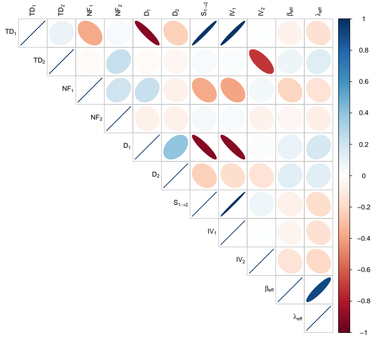
Figure 3.7: Correlation matrix for neutronic inputs.
