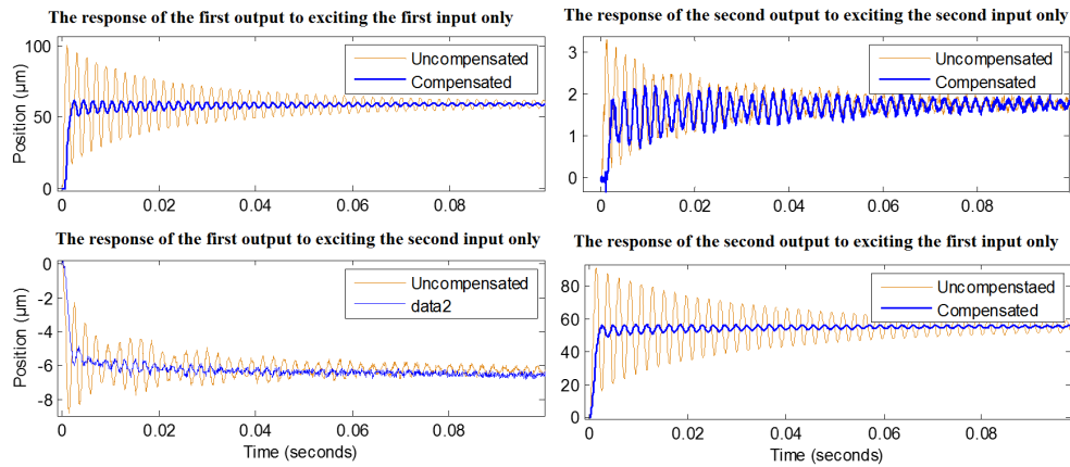
Figure 6.17: Exciting one input and showing the cross coupling effect experimental results.
