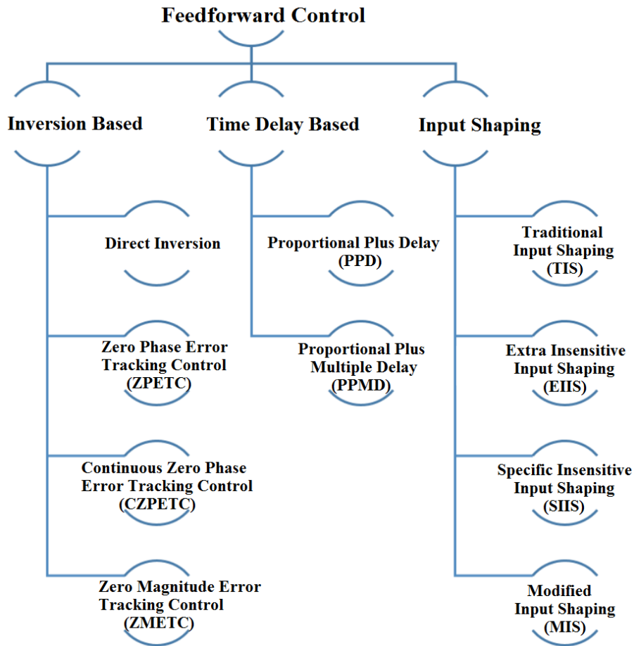
Figure 3.2: Classification of some feedforward control schemes.
