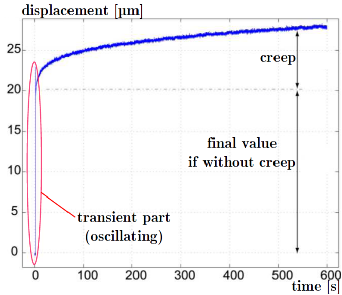
Figure 2.10: Example of creep in piezoelectric cantilever
