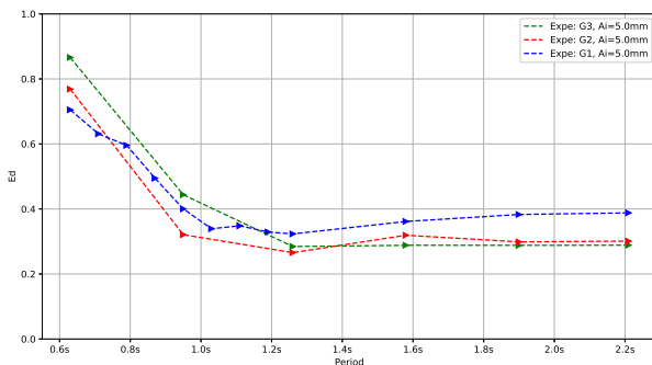
Figure 4.28: Dissipation rate, A_i=12.5\text{mm}
