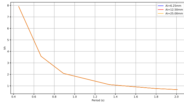
Figure 3.16: kh , Simple porous medium
