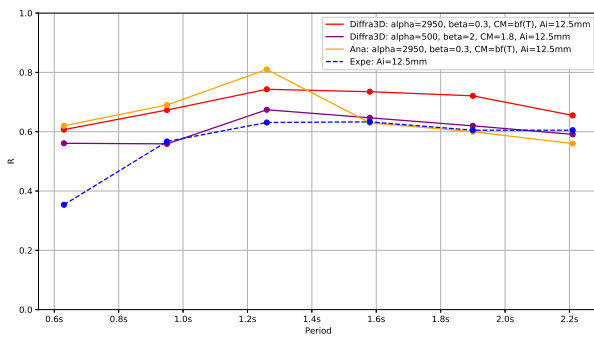
Figure 4.26: Reflection curve, A_i=12.5\text{mm}
