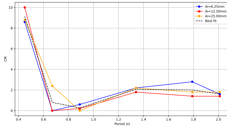
Figure 3.12: Inertia coefficient C_M , Simple porous medium
