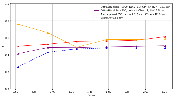
Figure 4.27: Transmission curve, A_i=12.5\text{mm}
