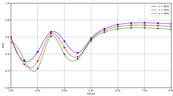
Figure 2.9: Reflection coefficient, A_i = 250mm Sensitivity to porosity
