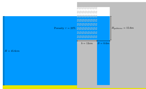
Figure 5.16: Spaced gabions, no floor
