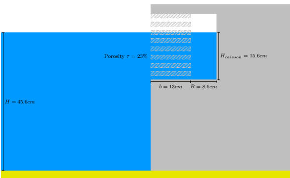
Figure 5.15: Spaced gabions
