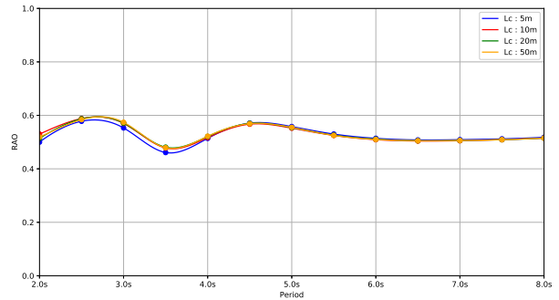
Figure 2.8: Transmission coefficient, A_i = 250mm Sensitivity to channel's length
