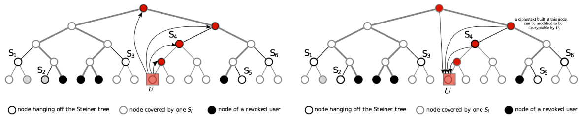
Figure 4.1: Comparison between Asano's method and our method.
