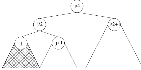
Figure I.6: SD Key Assignment for S_{j/4,j}
