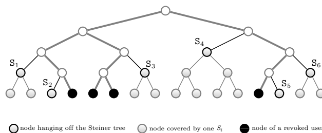
Figure F.1: Complete subtree: leaves correspond to users, S_1, \dots, S_6 is the covering that excludes revoked users in black while allowing other users to decrypt derived from the Steiner tree associated to the set of revoked users R .
