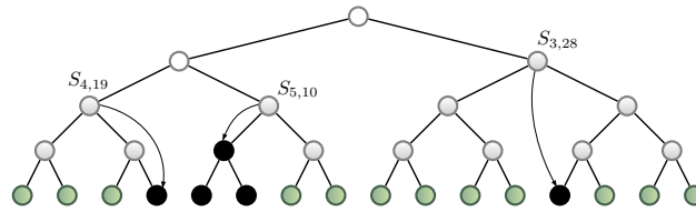
Figure 2.3: Subset difference: leaves correspond to users and black nodes are not able to derive the necessary information to decrypt. Therefore S_{4,19} prevents user 19 from decrypting, S_{5,10} prevents users 20 and 21 from decrypting, and S_{3,28} prevents user 28 from decrypting. All other users are able to decrypt.
