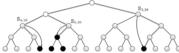
Figure F.3: Subset difference: leaves correspond to users and black nodes are not able to derive the necessary information to decrypt. Therefore S_{4,19} prevents user 19 from decrypting, S_{5,10} prevents users 20 and 21 from decrypting, and S_{3,28} prevents user 28 from decrypting. All other users are able to decrypt.
