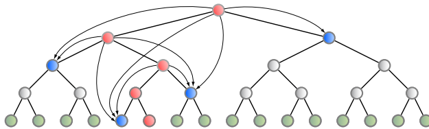
Figure 2.2: Key assignment. User u receives all the labels \text{LABEL}_{i,j} such that i is a parent of j and i is on the path from the leaf of u to the root.
