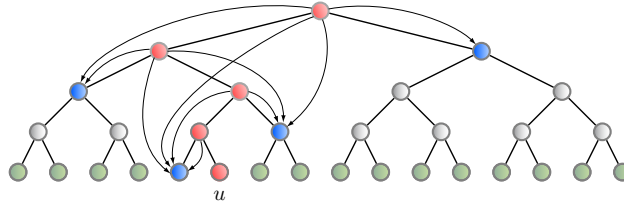
Figure F.2: Key assignment. User u receives all the labels \text{LABEL}_{i,j} such that i is a parent of j and i is on the path from the leaf of u to the root.
