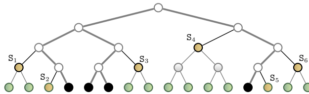
Figure 2.1: Complete subtree: leaves correspond to users, S_1, \dots, S_6 consist of the covering that excludes revoked users (in black) while allowing other users to decrypt. This is derived from the Steiner tree associated to the set of revoked users R .
