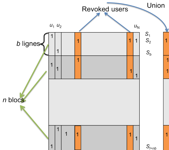
Figure 2.5: Construction of (r, s) -disjunct matrices
