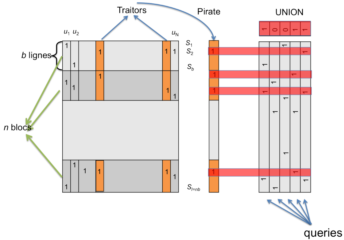
Figure 2.6: The shadow technique
