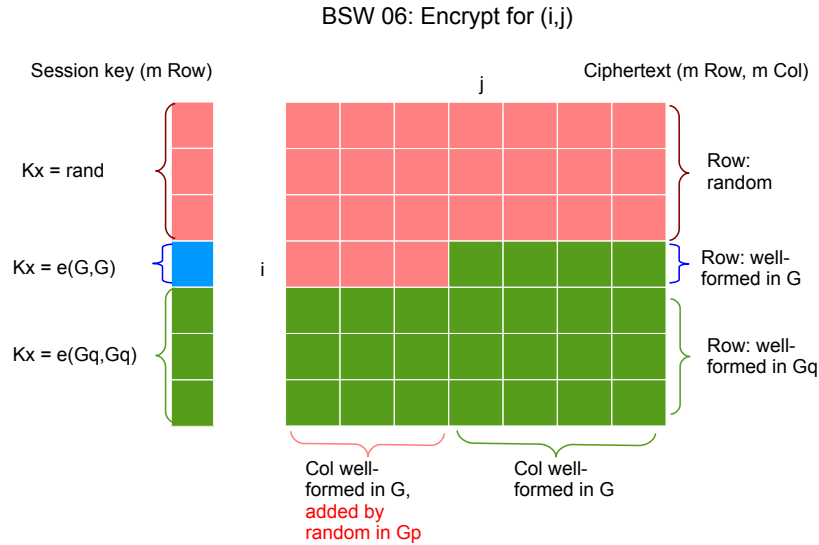
Figure 3.2: High-level view of the BSW's method.
