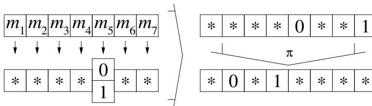
Figure 3.3: Hiding a mark at position 5 in a sequence of 7 blocks.
