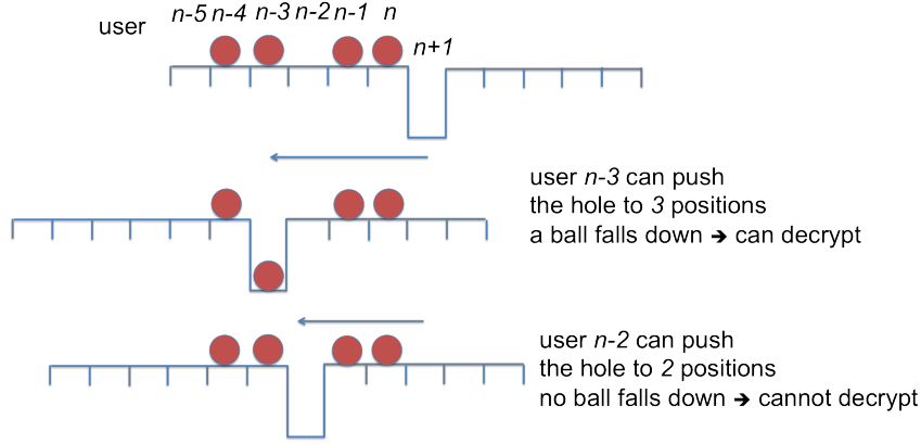
Figure 3.1: High-level view of the BGW method.
