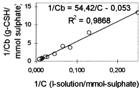
Figure 1.17 – Langmuir isotherm of \text{SO}_4^{2-} ions on C-S-H in 0.5 mol/L NaOH at T=25\text{ }^\circ\text{C} [97]
