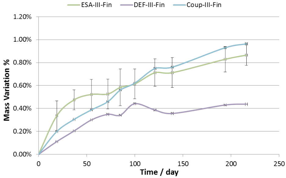
Figure 3.38 – Mass variations of the CEM III 2 \times 2 \times 12 \text{ cm}^3 specimens.
