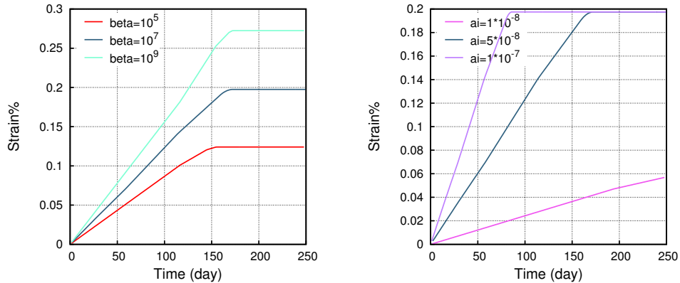
(a) Effect of \beta on strain% with a_i = 5 \times 10^{-8} , E = 20 GPa and b=1 . (b) Effect of kinetic constant a_i on strain% with \beta = 1 \times 10^7 , E = 20 GPa and b=1 .
