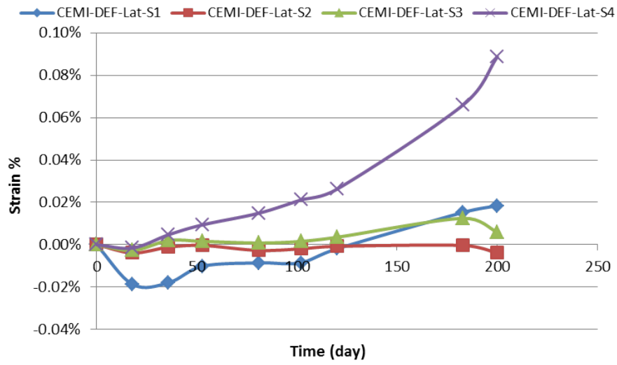
Figure B.7 – Strain of DEF-I-Lat 11 \times 11 \times 22 \text{ cm}^3 specimens on different faces
