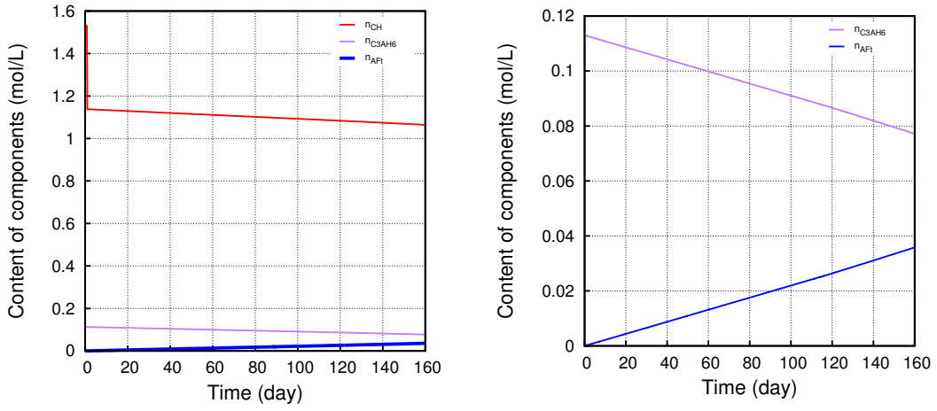
Figure 4.27 – Content of CH, CSH 2 , C 3 AH 6 and AFT when pH is not controlled
