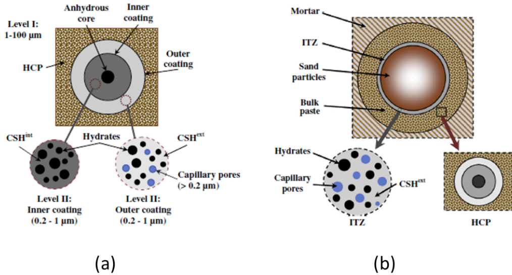
Figure 1.30 – 2D representation of the cement paste microstructure (a) and mortar microstructure (b) used to estimate the effective elastic and diffusive properties [204].
