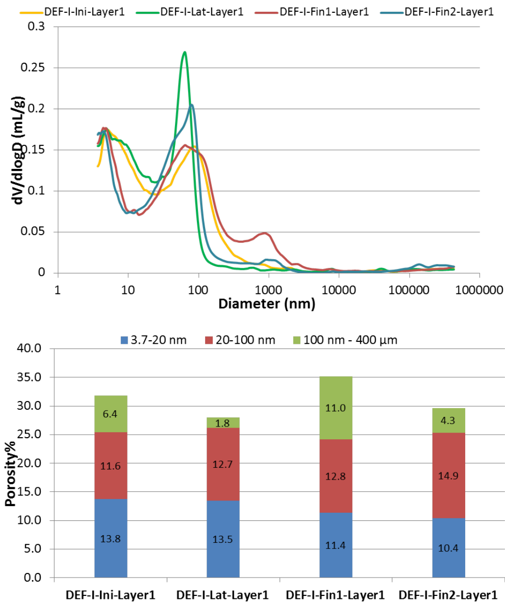
Figure C.1 – Evolution of pore size distribution of 11 \times 11 \times 22 \text{ cm}^3 DEF specimen at the core layer
