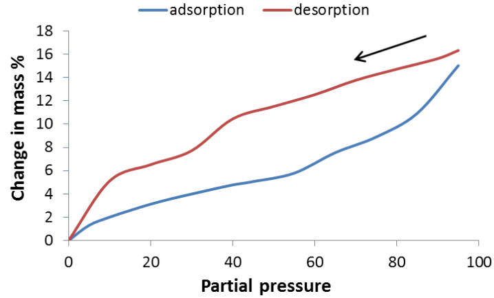
Figure 2.19 – Water vapor sorption isotherm from DVS.
