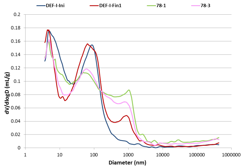
Figure 3.34 – Pore size distribution measured from MIP after the heat-based dissolution test at 78 °C
