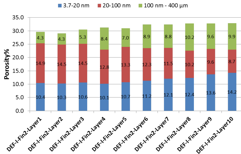
Figure 3.25 – Pore volume in different pore ranges of the 11 × 11 × 22 cm 3 DEF-I-Fin2 specimen along the depths at the final state from MIP.
