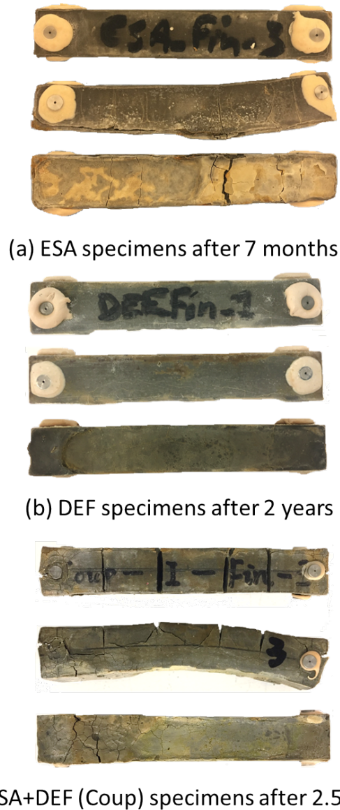
Figure 3.1 – Observations of a selection of specimens under different sulfate attack conditions (for each attack, the same specimen is observed from different surfaces).
