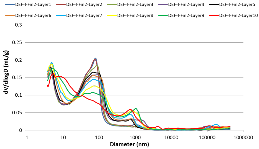
Figure 3.24 – Pore size distribution of the 11 × 11 × 22 cm 3 DEF-I-Fin2 specimen along the depths at the final state from MIP.
