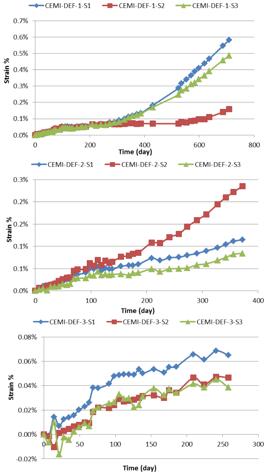
Figure B.2 – Strain of DEF-I-Fin 2 \times 2 \times 12 \text{ cm}^3 specimens on different faces
