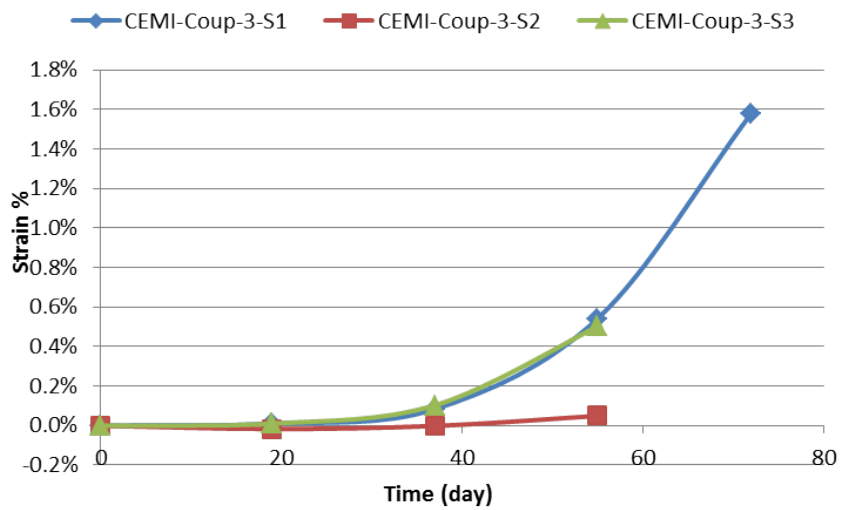
Figure B.3 – Strain of Coup-I-Fin 2 \times 2 \times 12 \text{ cm}^3 specimens on different faces
