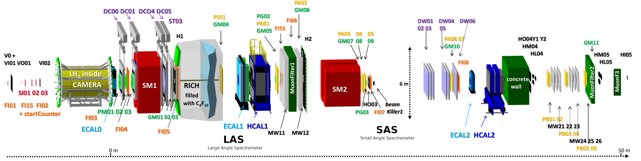
Figure 24: Schematic view of the COMPASS 2016/2017 setup.
