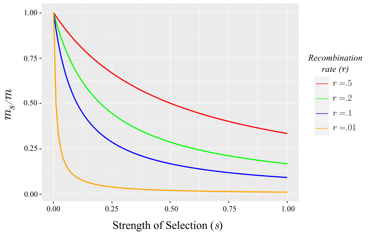
Figure 4.1 – The relation between effective migration and migration for the neutral model ( m_s/m ) as a function of the strength of selection ( s ) for various values of r .
