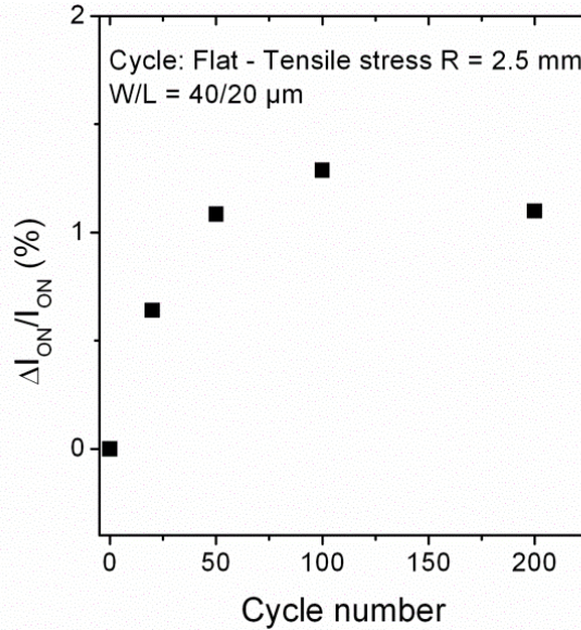
Figure 3.24: Relative variation of the on-current at V_{GS}=30 V of the 40/20\mu\text{m} TFT when submitted to Flat – Tensile cycles at R=2.5\text{mm} until 200 cycles.
