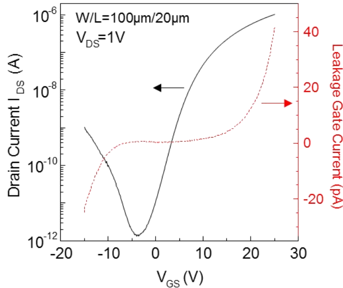
Figure 4.5: Transfer characteristic of microcrystalline silicon TFT (100/20 µm) with ECR-CVD deposited silicon oxide as gate insulator
