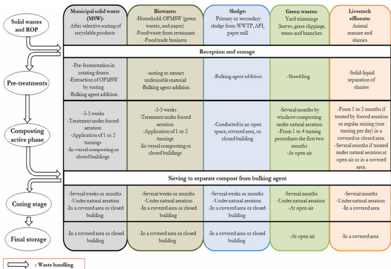
Fig. 7. Summary of operational stages involved in the composting process of solid wastes and ROP
