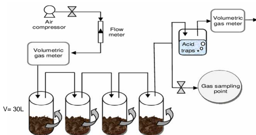
Fig. 3. Experimental device used to monitor gas emissions during the turning of compostable substrates
