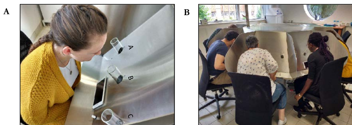
Fig. 4. Dynamic olfactometer and odor concentration (OC) measurement: three port-sniffing station (A), odor panel formed by 5 up to 8 assessors (B)
