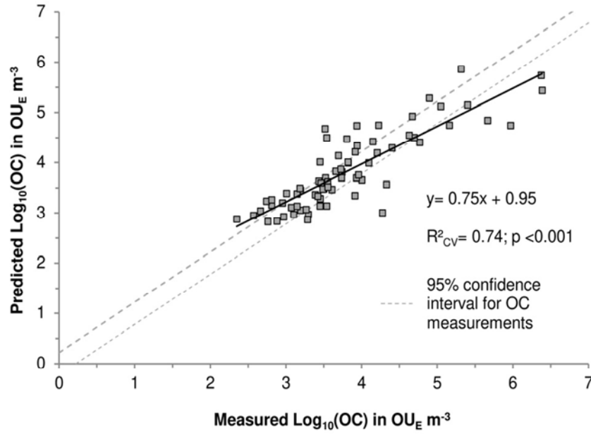
Fig. 4. Comparison between the measured odor concentration (OC in \text{OU}_E \text{ m}^{-3} ) and the predicted OC. A partial least squares (PLS) regression model with three components was validated by cross-validation ( N=72 ). OC was predicted by the weighted odor activity values (OAV) of 10 odorants. OC and OAV were log-transformed
