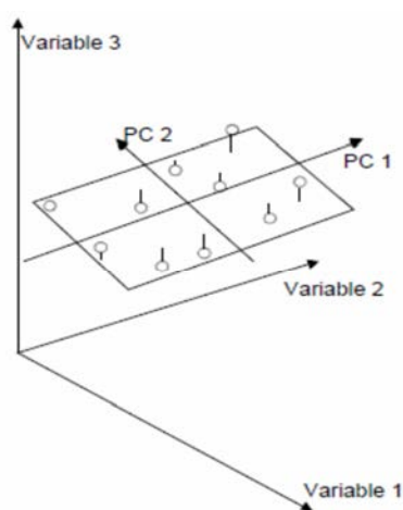
Fig. 6. Principal Components (PC) in a multidimensional space (Camo, 2006)
