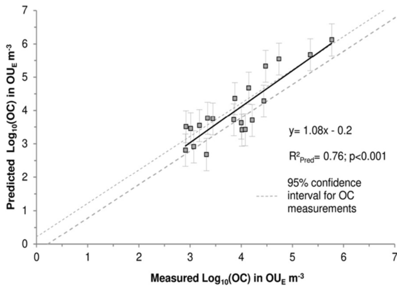
Fig. 5. Test set validation ( n=20 ) of the developed PLS model with three components. Odor concentration (OC in \text{OU}_E \text{ m}^{-3} ) was predicted by the weighted odor activity values (OAV) of 10 odorants. OC and OAV were logarithmically transformed. Root mean square errors of test set validation (RMSEP) are depicted for each prediction
