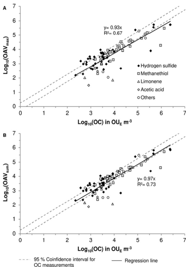
Fig. 1. Linear correlations between (A) the maximum OAV (OAV max ) and odor concentration (OC), and (B) the sum of individual OAV (OAV sum ) and OC for 92 gas samples from the active composting phase of 9 organic matrices. OAV and OC were log-transformed. Main compounds displaying the OAV max are indicated for all gas samples in both correlations. The regression lines are depicted as full lines, and the dashed lines represent the 95% confidence intervals for OC measurements
