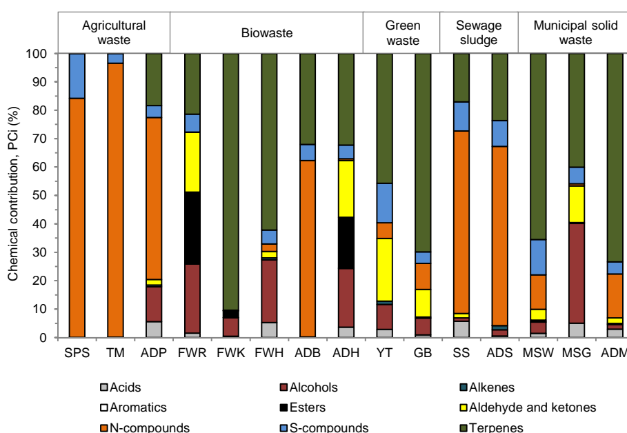
Fig. 4. Chemical contribution PC_i (%) of identified chemical families during the composting process of solid wastes and digestates
