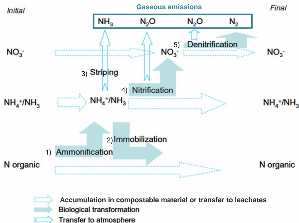
Fig. 14. Nitrogen transformations and major nitrogen species released during composting (adapted from de Guardia et al., 2010)
