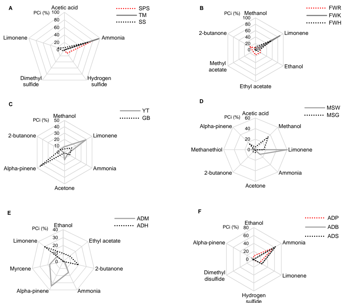
Fig. 5. Chemical contribution PC i (%) of major volatile compounds emitted upon composting of agricultural waste and sewage sludge (A), biowaste (B), green waste (C), municipal solid waste (D), and digestates (E, F)
