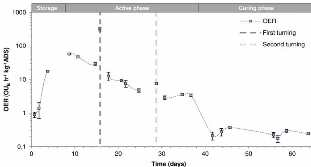
Fig. 5. Odor emission rates at different operational stages of ADS composting
