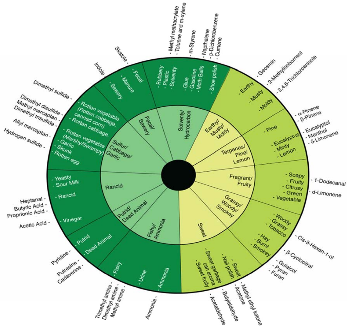
Fig. 3. Composting odor wheel (Rosenfeld et al., 2007)
