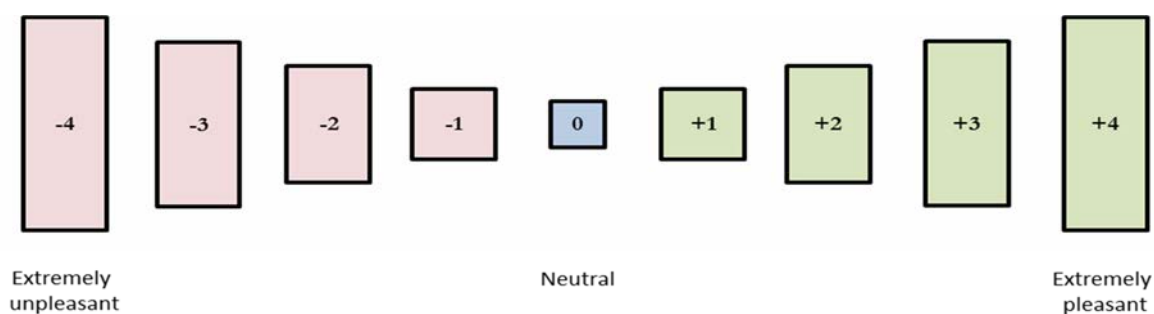
Fig. 4. Nine-point category scale to assess hedonic tone according to the VDI 3882/Part 2 guideline
