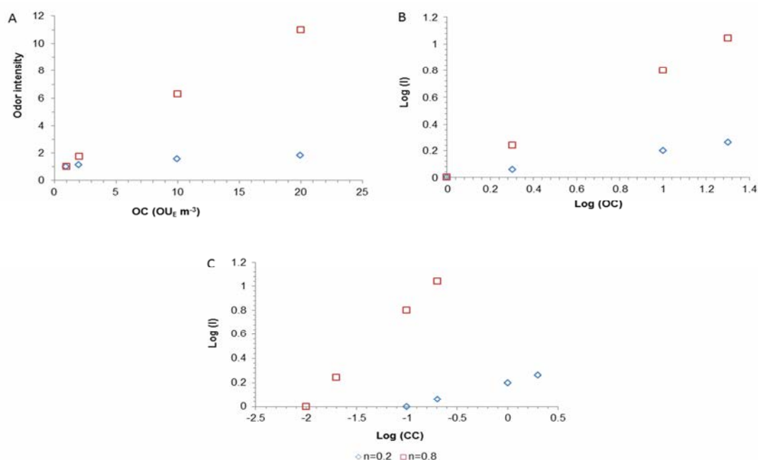
Fig. 2. Odor intensity ( I ) as a function of odor concentration (OC in \text{OU}_E \text{ m}^{-3} ) (A), \text{Log}(I) as a function of \text{Log}(OC) (B), and \text{Log}(I) as a function of \text{Log} of chemical concentration (CC) (C) for two gas samples containing different single compounds with n equal to 0.2 and 0.8
