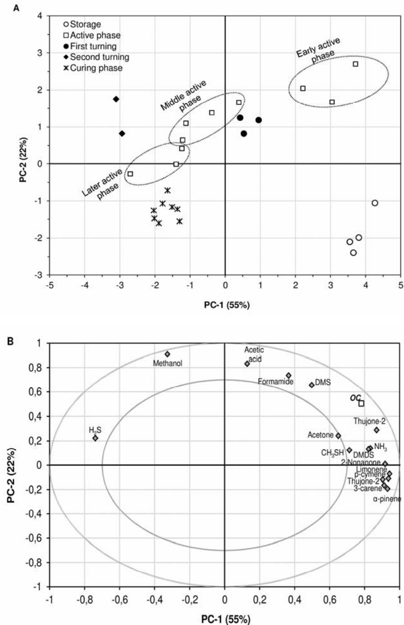
Fig. 7. Score plot (A) and correlation loading plot (B) obtained by the principal component analysis (PCA) on odor concentration (OC in \text{OU}_E \text{ m}^{-3} ) and odor activity values (OAV, dimensionless) of pollutants released along different composting stages (storage, active phase, first turning, second turning and curing phase) of anaerobically digested sewage sludge
