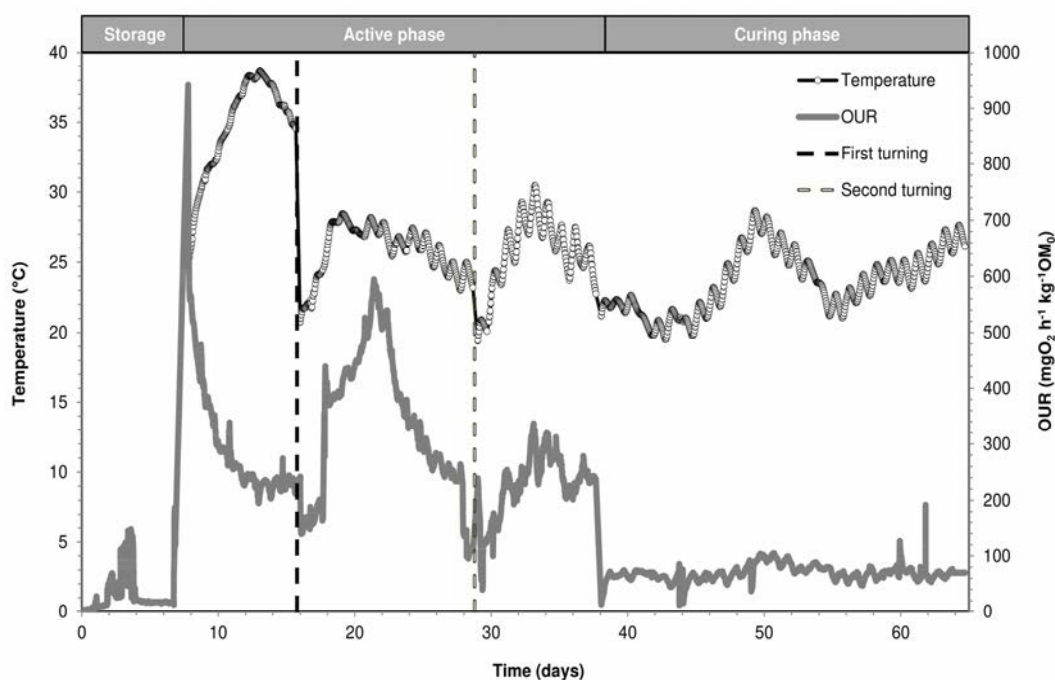
Fig. 3. Oxygen uptake rates (OUR) and temperature throughout the operational composting stages of anaerobically digested sewage sludge (ADS)
