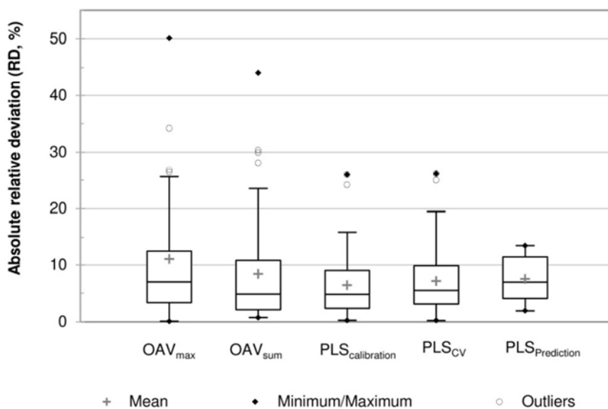
Fig. 6. Percentage of absolute relative deviation (RDs, %) for odor concentrations (OC in \text{OU}_E \text{ m}^{-3} ) predictions standing outside of the 95% confidence interval for the OC measurements. Predictions were conducted by a partial least squares (PLS) regression model with three components and odor surrogates such as the maximum odor activity value ( \text{OAV}_{\text{max}} ) and the sum of individual OAV ( \text{OAV}_{\text{sum}} ). The RDs from the PLS calibration model, cross-validation (CV) and test set validation (prediction) are depicted
