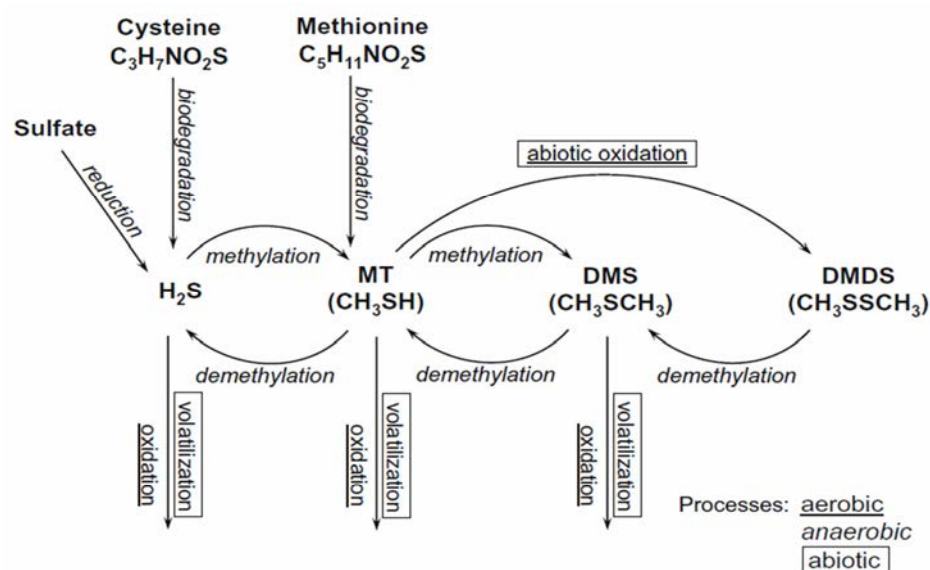
Fig. 13. Production and degradation of principal volatile sulfur compounds (Drennan and DiStefano, 2010)
