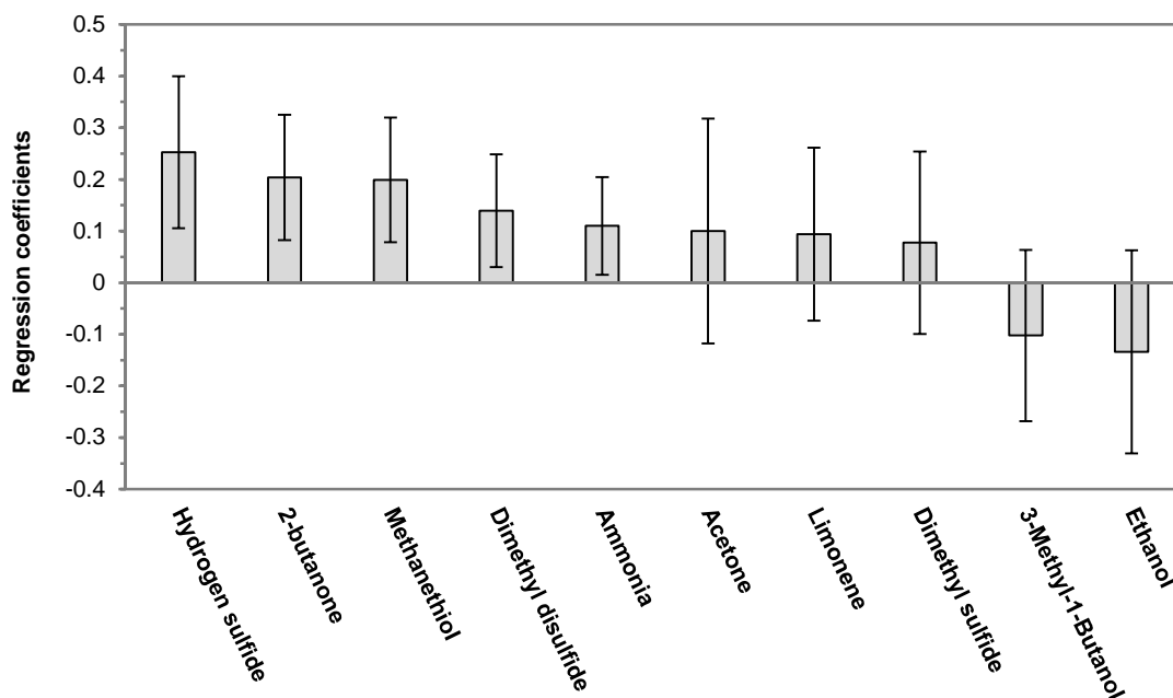
Fig. 3. Regression coefficients for the final partial least squares (PLS) regression model to predict odor concentration (OC in \text{OU}_E \text{ m}^{-3} ) through odor activity values (OAV). OC and OAV were log-transformed to build a 3-PLS components model. Error bars represent the uncertainty estimates calculated by the jack-knifing approach
