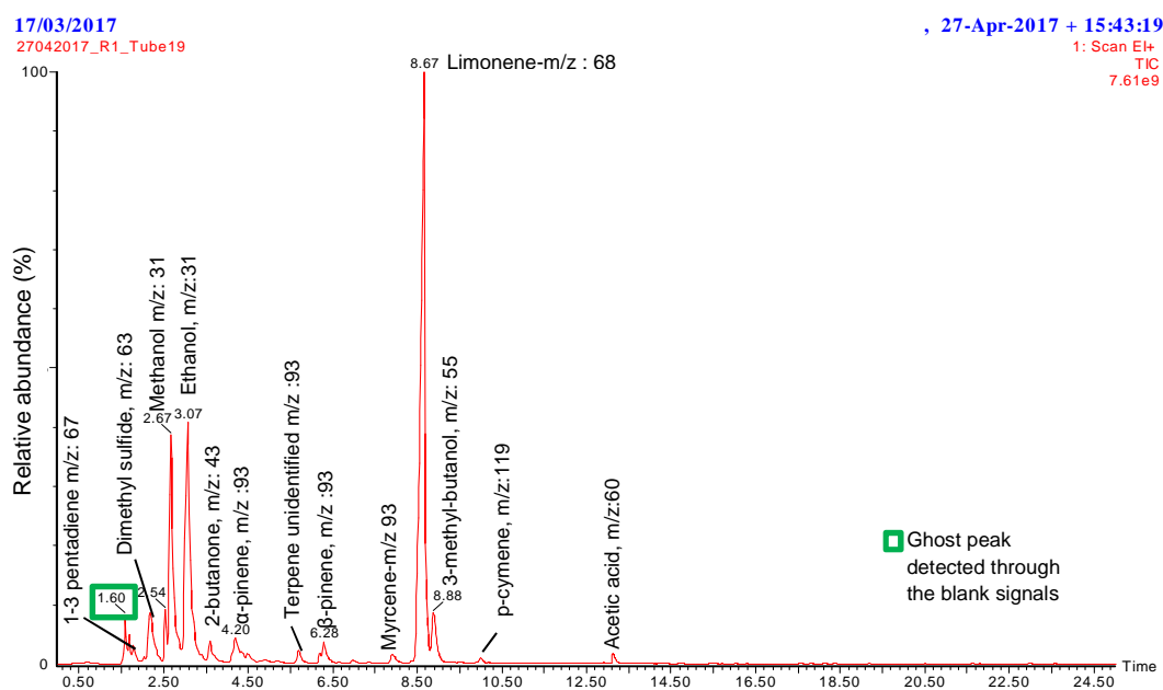
Fig. 1S. GC chromatogram for a gas sample collected during composting of household biowaste
