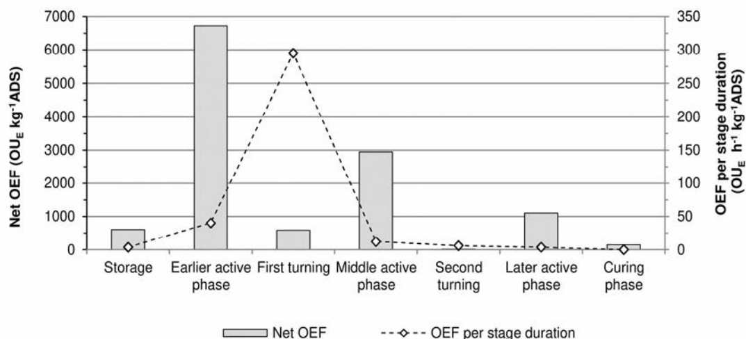
Fig. 6. Odor emission factors (OEF) for each composting stage. OEF was also expressed as a ratio of the stage time duration (hours)
