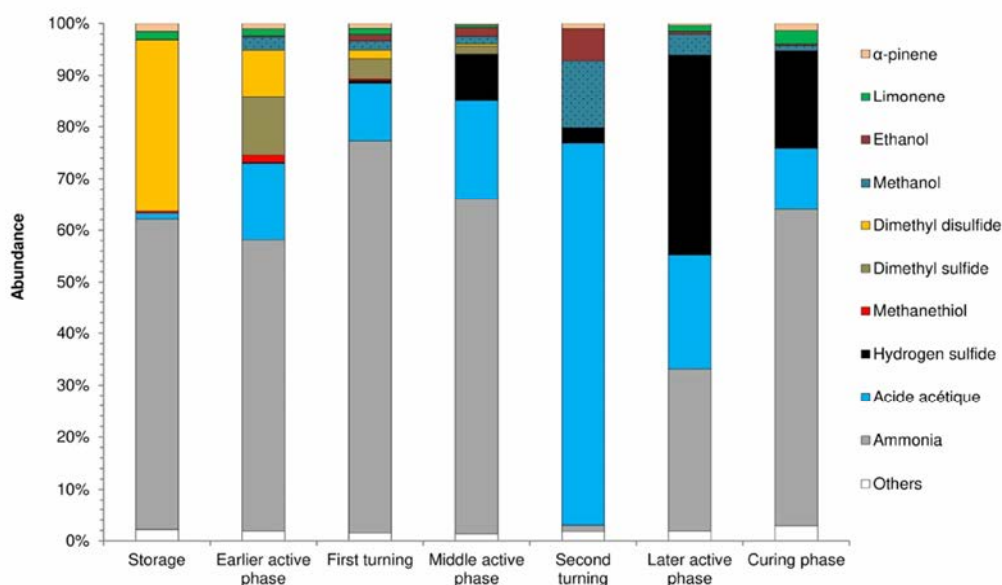
Fig. 4. Abundance (%) of the major volatile compounds emitted throughout the composting process of anaerobically digested sewage sludge. The emissions' chemical fingerprints at each composting stage are depicted
