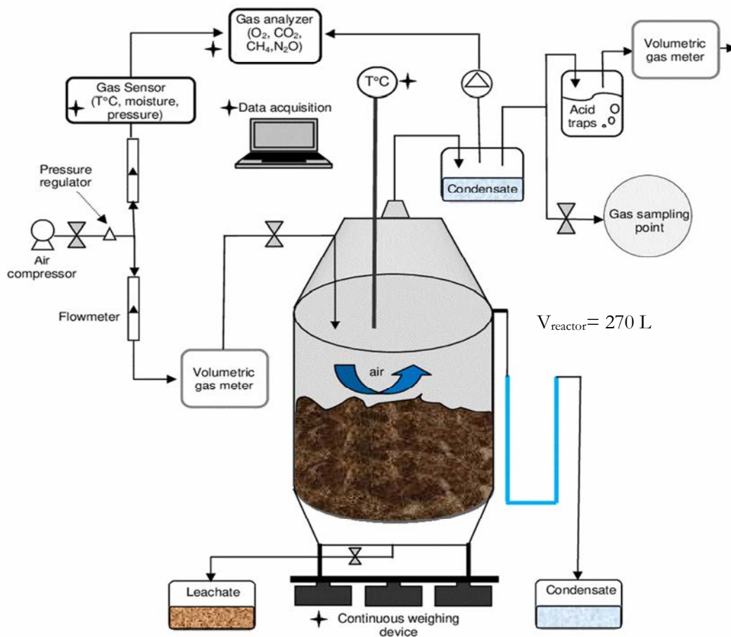
Fig. 1. Experimental device used to simulate and monitor gas emissions during storage and curing stage
