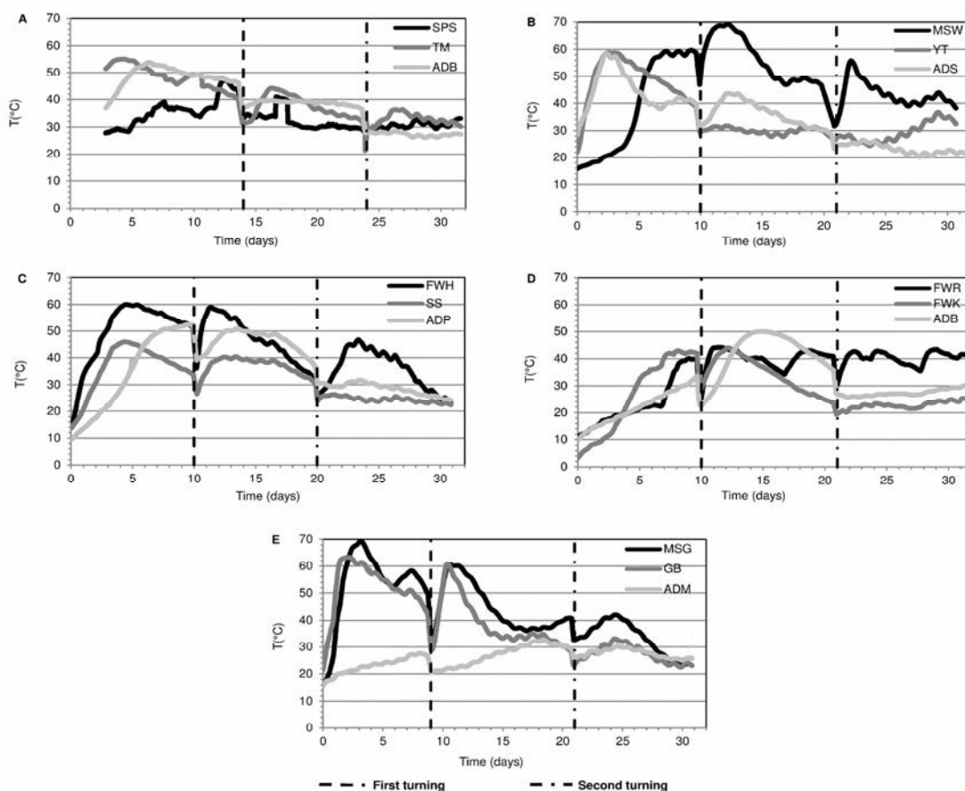
Fig. 1. Temperature ( T, ^\circ\text{C} ) profiles for solid waste and digestates composting
