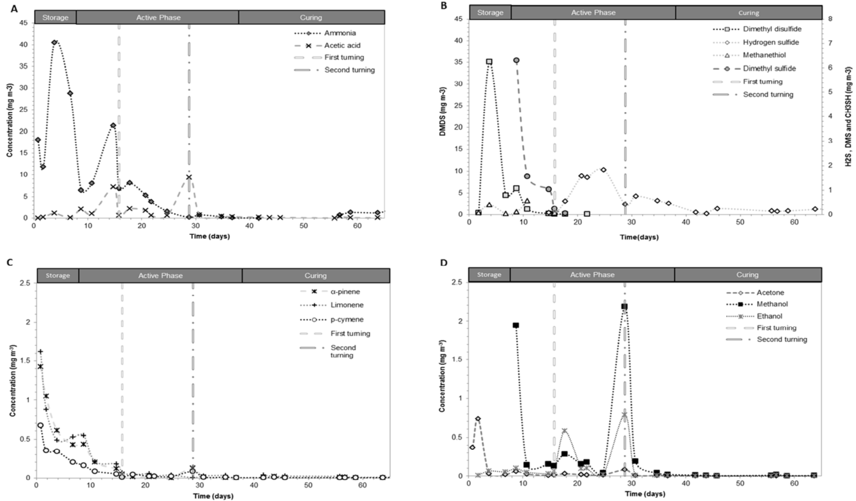
Fig. 1S. Emission profiles of main pollutants released upon composting of anaerobically digested sewage sludge: ammonia and acetic acid (A), volatile sulfur compounds (B), terpenes (C) and oxygenated compounds (D)
