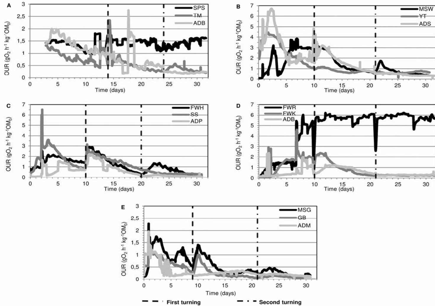
Fig. 1S. Oxygen uptake rates (OUR in \text{gO}_2 \text{ h}^{-1} \text{ kg}^{-1} \text{ OM}_0 ) profiles along composting of solid wastes and digestates
