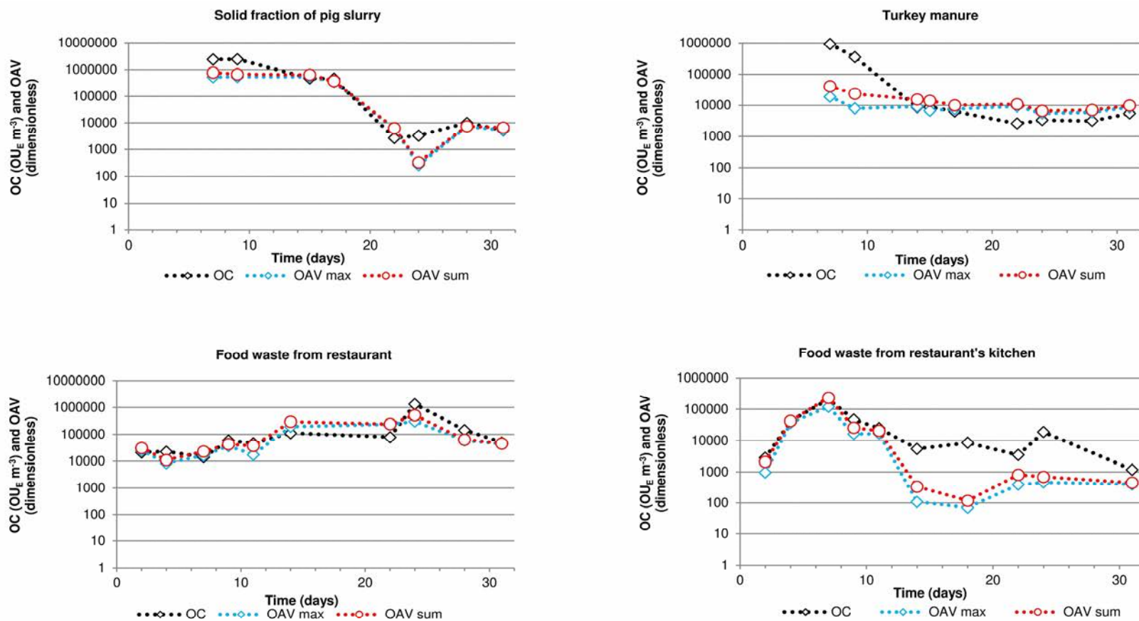
Fig. 2S. Odor emission profiles during composting process of solid wastes and digestates: Odor concentration in \text{OU}_E \text{ m}^{-3} and OAV (dimensionless)
