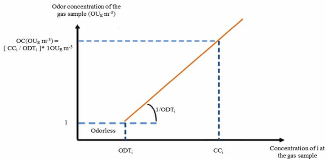
Fig. 1. Odor concentration (OC in \text{OU}_E \text{m}^{-3} ) as a function the odorant's concentration for a gas sample containing one single compound (Adapted from Blazy, 2014)
