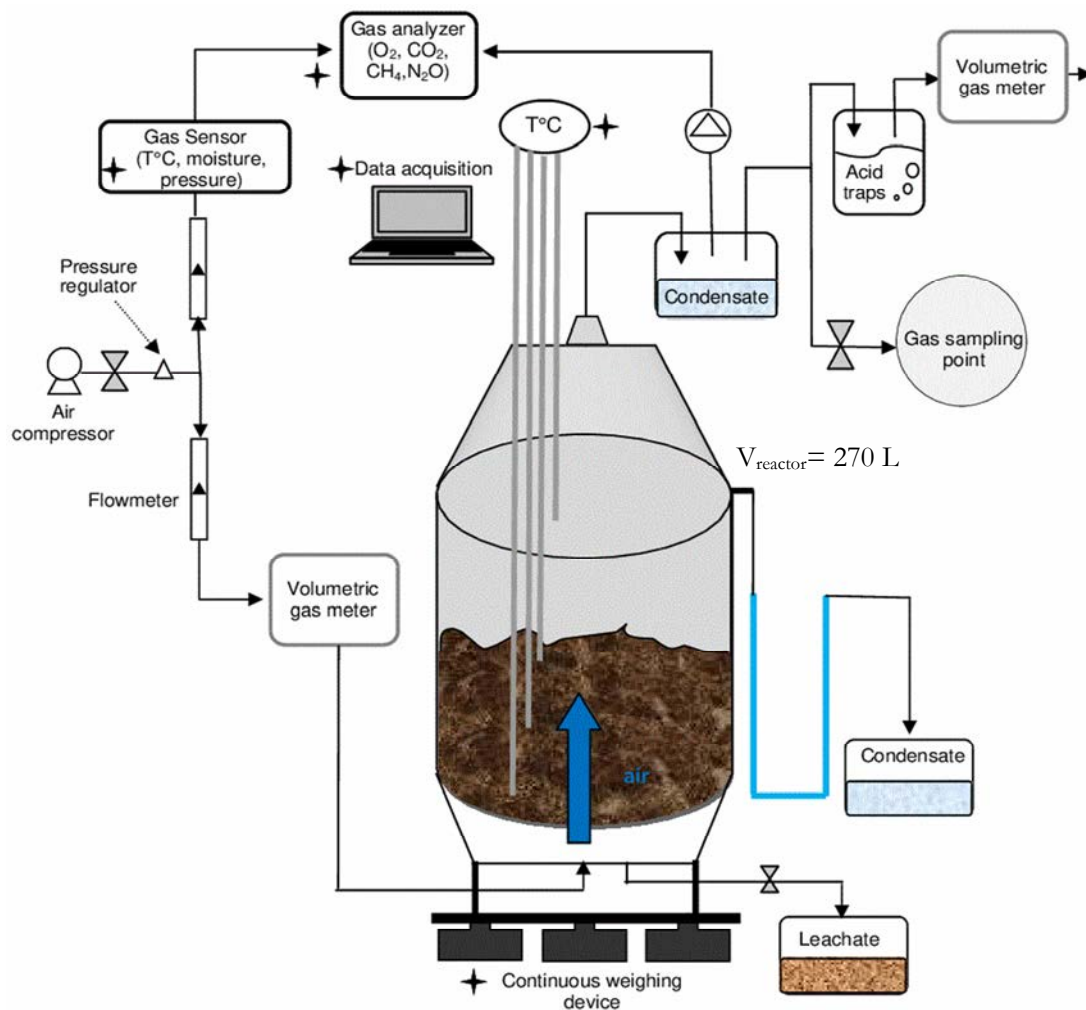
Fig. 2. Experimental device used to simulate and monitor the composting active phase
