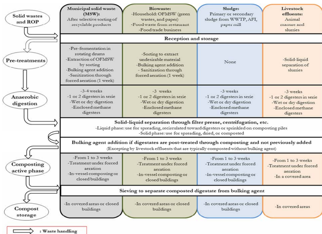
Fig. 8. Summary of operational stages involved in the methanization process of solid wastes and ROP
