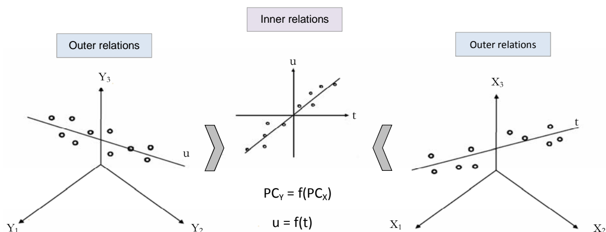
Fig. 8. Basic procedure to construct PLS components (Adapted from Camo, 2006)
