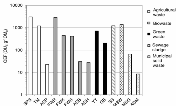
Fig. 3. Odor emission factors (OEF in OU_E g^{-1} OM_0 ) obtained upon aerobic treatment of solid wastes and digestates
