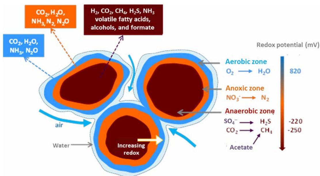
Fig. 9. Schematic representation of oxidation gradients in composting and their impacts on biological reactions and gaseous emissions (Dabert and Pourcher, 2018)
