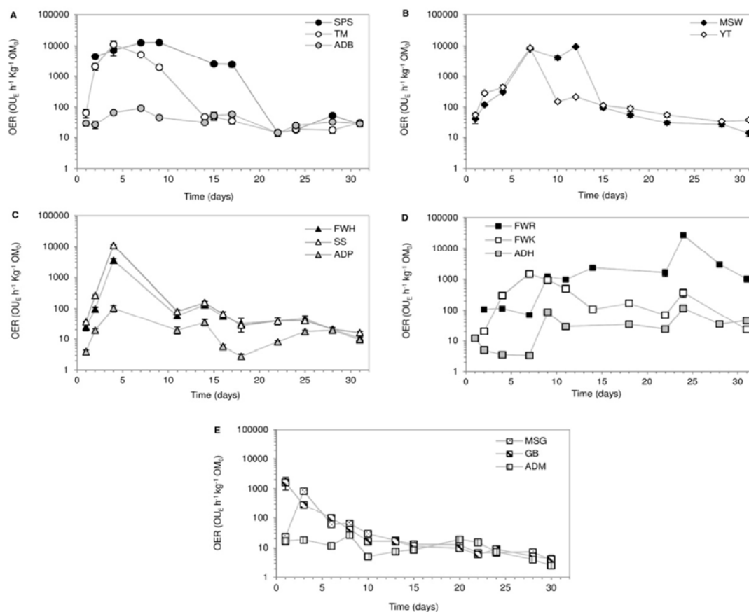
Fig. 2. Odor emission rates (OER in \text{OU}_E \text{ h}^{-1} \text{ kg}^{-1} \text{ OM}_0 ) for solid wastes and digestates composting
