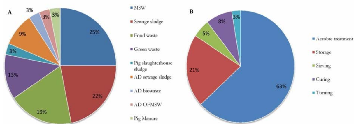
Fig. 15. Organic matrices (A) and operational stages (B) commonly assessed on studies dealing with odorants emissions from composting process
