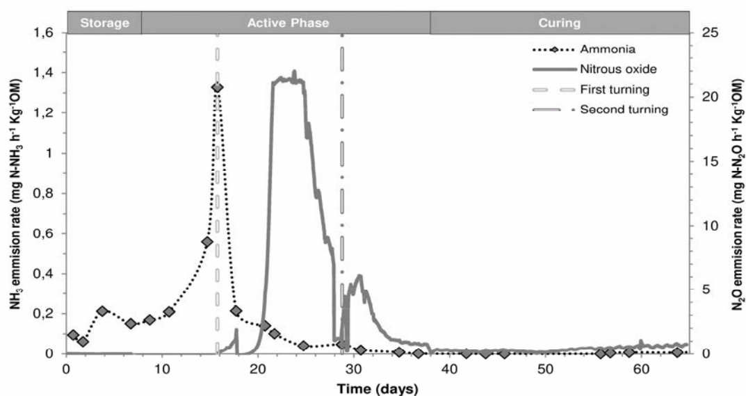
Fig. 2S. Emission rates for ammonia and nitrous oxide through different operational composting stages of ADS
