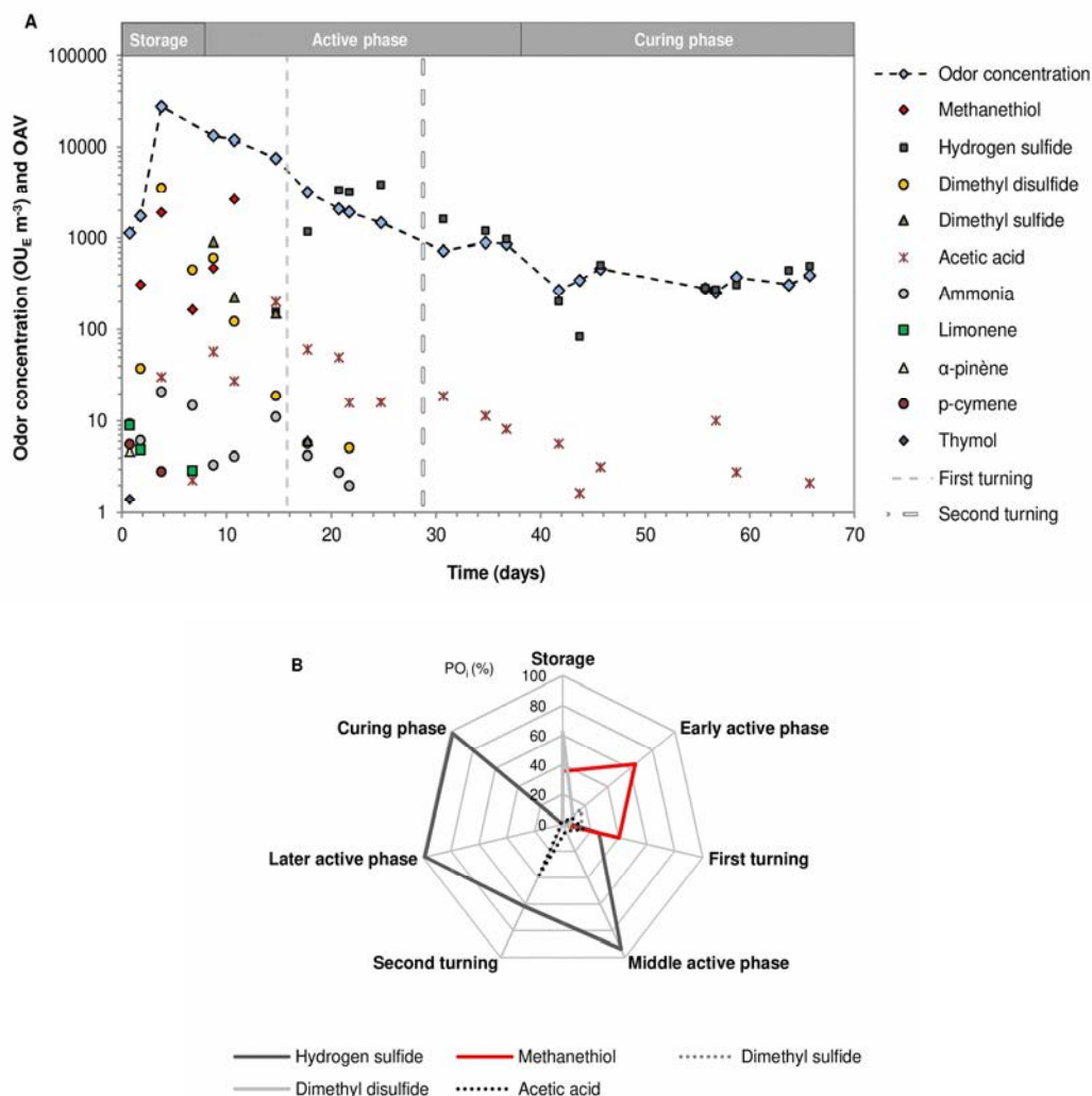
Fig. 8. Odor concentration (OC in OU E m -3 ) and odor activity values (OAV, dimensionless) profiles (A). Percentage of odor contribution (PO i , %) for the major odor-causing compounds released throughout the different stages of ADS composting (B)
