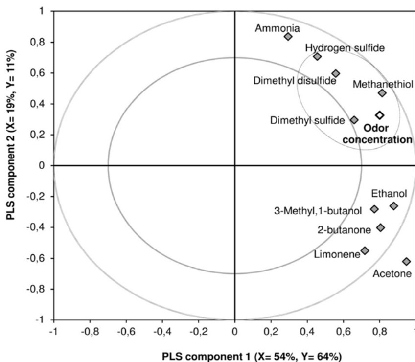
Fig. 2. Correlation loadings plot for a developed partial least squares (PLS) model to predict odor concentration (OC in \text{OU}_E \text{ m}^{-3} ) through odor activity values (OAV). OC and OAV were log-transformed. The first two PLS components explained 75% of the OC (Y) variance during model calibration
