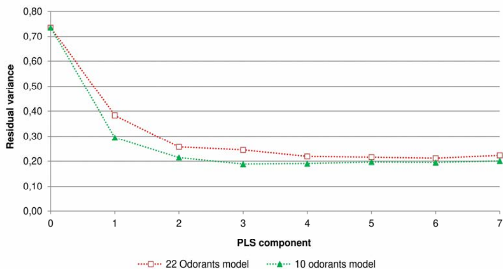
Fig. 3S. Changes in residual variance depending on the components number to developed two PLS models. The three-components PLS models exhibited the lowest residual variance
