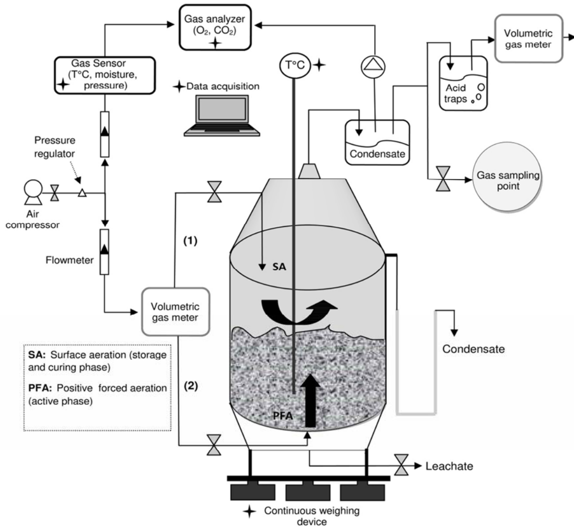
Fig. 1. Composting device and gas monitoring system. Two reactor configurations were set: (1) surface aeration (SA) to simulate the storage and curing phase; and (2) positive forced aeration (PFA) to simulate the active composting phase
