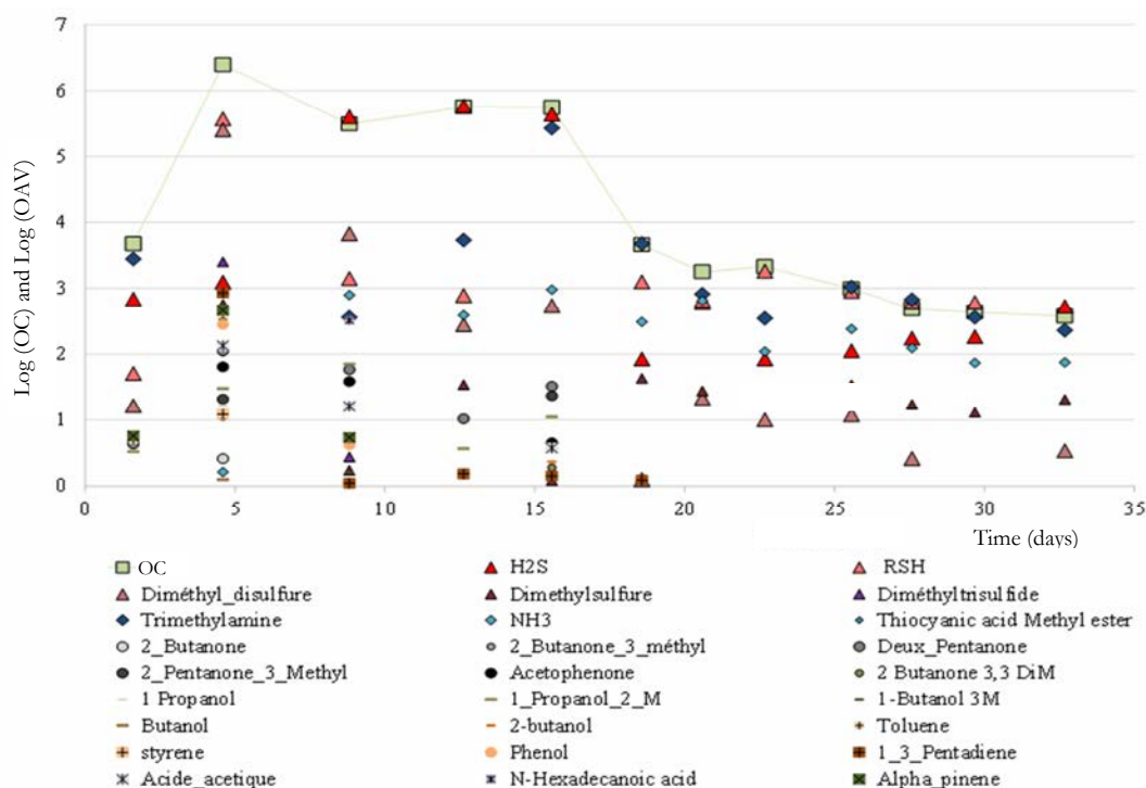
Fig. 11. OC and OAV (logarithmically transformed) as a function of time along the composting process of pig slaughterhouse sludge under forced aeration (Blazy, 2014)
