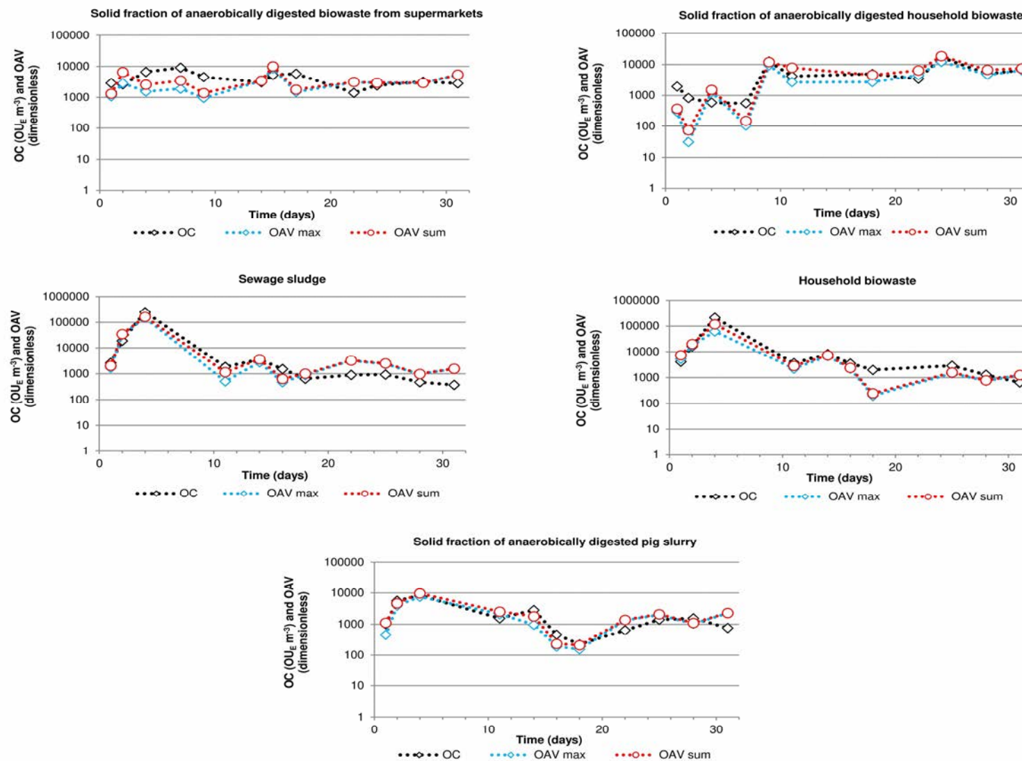
Fig. 2S. Odor emission profiles during composting process of solid wastes and digestates: Odor concentration in \text{OU}_E \text{ m}^{-3} and OAV (dimensionless)
