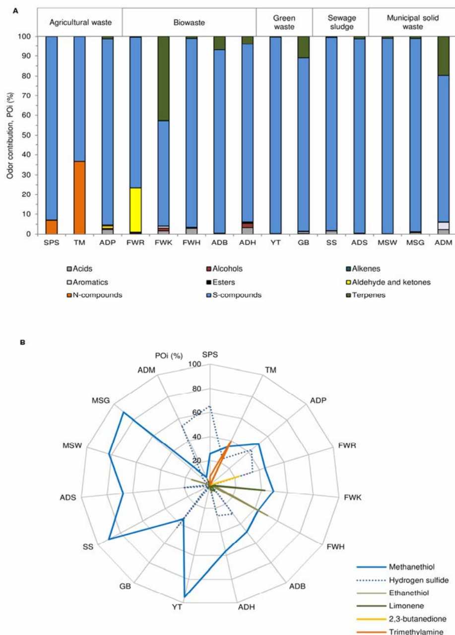
Fig. 6. Odor contribution (PO i , %) of identified chemical families (A) and main odorants (B) emitted upon the composting process of solid wastes and digestates
