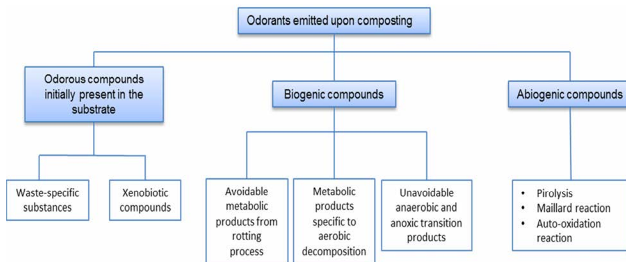
Fig. 12. Type of odor-causing compounds released during the composting process (adapted from Bidlingmaier and Müsken, 2007)
