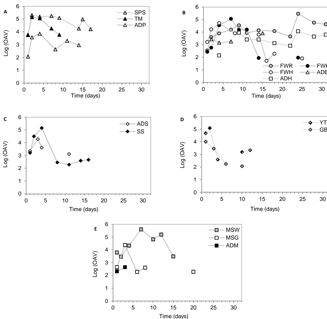
Fig. 7. OAV profiles for \text{CH}_3\text{SH} upon composting process of agricultural wastes (A), biowastes (B), green wastes (C), sewage sludge (D), and municipal solid waste (E)
