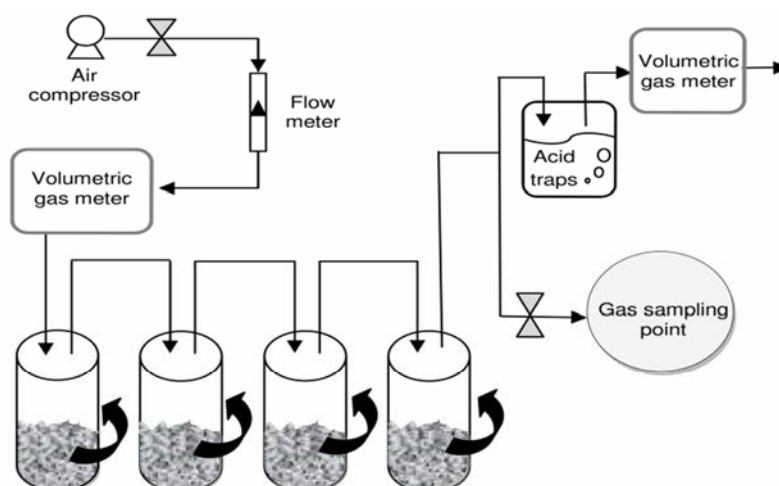
Fig. 2. Experimental device used to study the gas emission released throughout the turning process of compostable substrates
