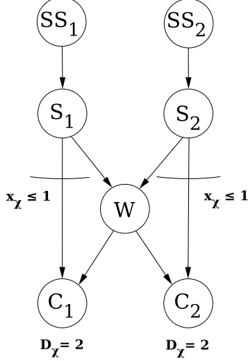
Figure 3.9: Valid inequalities
