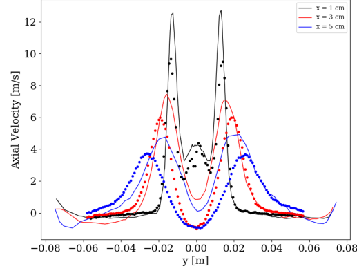
Figure 4.16: Plot of mean axial velocity along the y -axis for different heights along the chamber axis for the non-reacting flow simulation. Solid lines are numerical results; dots are experimental data
