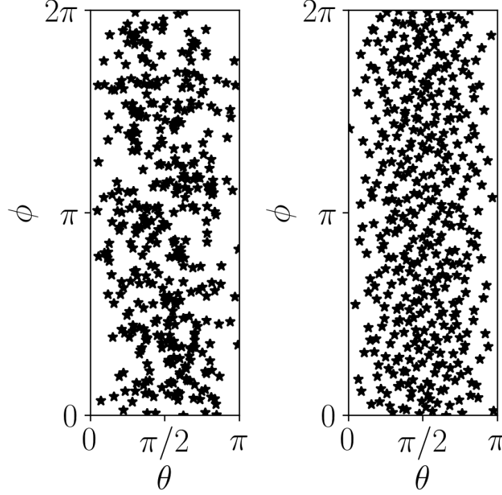
Figure 3.4: Comparison of the sampling of polar ( \theta ) and azimuthal angle ( \phi ) generated accordingly to the probability function defined in Eqs. (3.4 - 3.5) using a classic pseudo-random sequence (left) and a Sobol sequence (right) .
