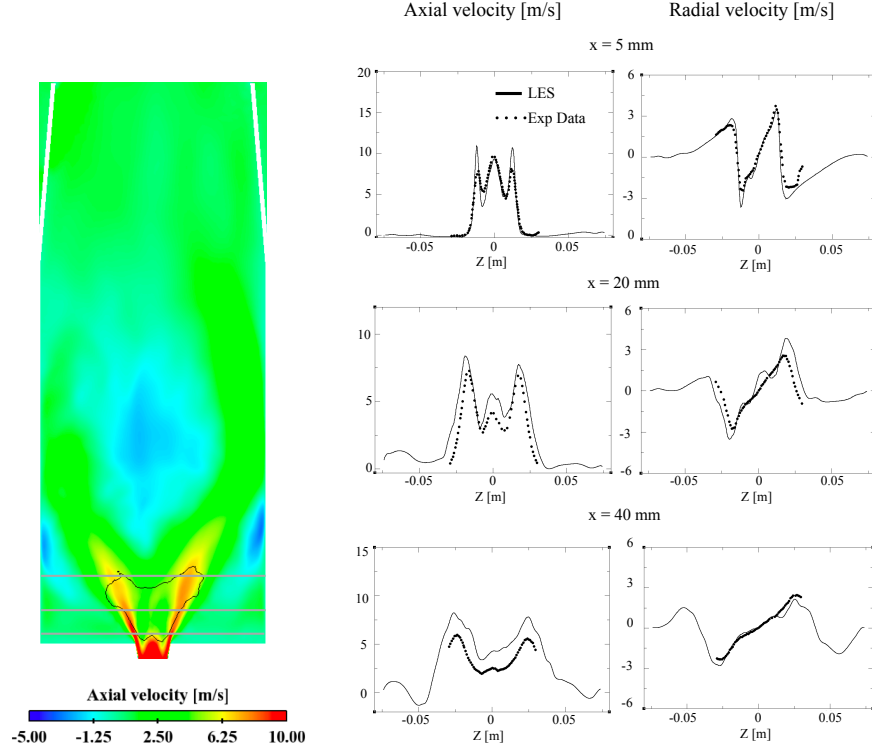
Figure 7.17: On the left: mean axial velocity field. Black line is the iso-contour of mean heat release equal to 4 \times 10^7 \text{ W m}^{-3} . On the right: axial and radial velocity profiles for three heights along the chamber: x = 5 \text{ mm} , x = 20 \text{ mm} , x = 40 \text{ mm} .
