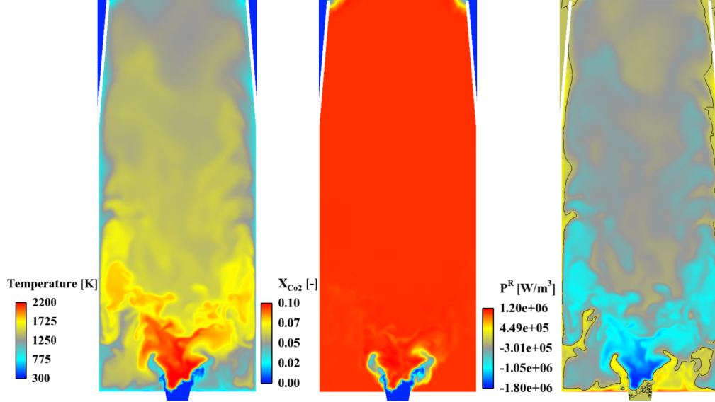
Figure 6.7: From left to right: instantaneous field of temperature, \text{CO}_2 molar fraction and radiative power on a longitudinal plane of the chamber. Black lines are iso-contour of P^R=0 .
