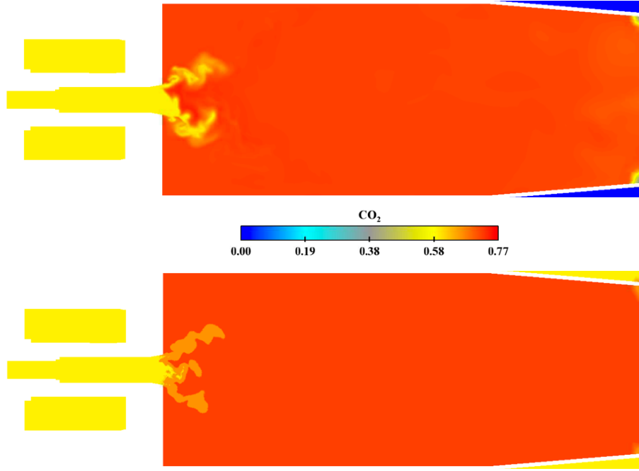
Figure 7.18: Instantaneous field of \text{CO}_2 molar fraction taken from preliminary LES of Flame B (top) and its adaptation to the spatial distribution of \text{CO}_2 field taken from converged LES of Flame A.
