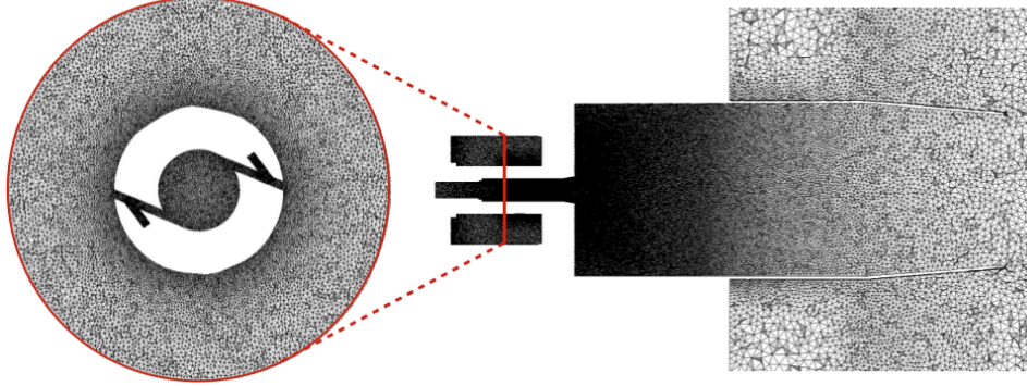
Figure 4.7: Visualization of the numerical domain through a 2D cut of the numerical domain on a cross section of the injector (left) and on a longitudinal plane of the chamber (right).
