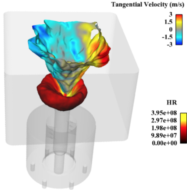
Figure 4.26: Iso-surfaces of axial velocity equal to 0 delineating the inner recirculation zone, colored by the tangential velocity, and iso-surface of progress variable equal to 0.9 colored by the heat release.
