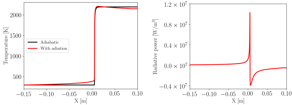
Figure 7.5: Temperature profile with and without radiation (left) and radiative power profile (right) for Flame B.
