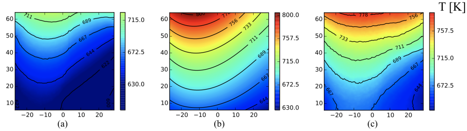
Figure 1.5: Wall temperature over the measurements zone (lengths in mm). (a): numerically computed wall temperature without radiation. (b) experimentally measured temperature ( Mercier et al. 2016 ). (c): numerically computed wall temperature with radiation ( Koren et al. 2017 ).
