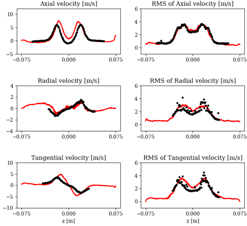
Figure 4.15: Profiles of mean (left) and RMS (right) velocity at x = 3 cm from the injector outlet: axial (top), radial (middle) and tangential (bottom) component. -- : Numerical results; \bullet : Experimental data.
