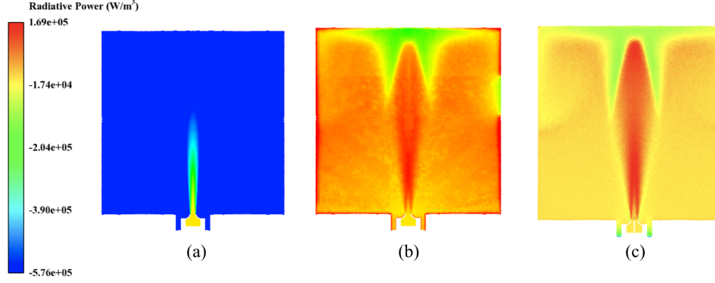
Figure 1.8: Numerical radiative power fields obtained in case of optically thin assumption (a), solved with a Discrete Ordinates Method using a gray gas model (b) and solved with a Monte Carlo method with a narrow band model (c).
