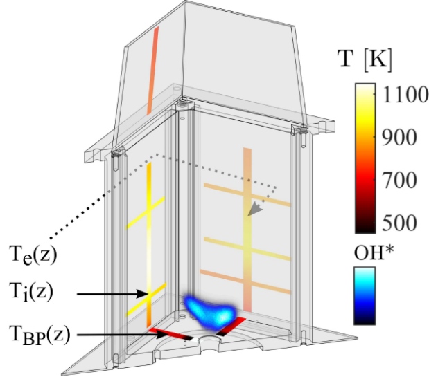
Figure 4.5: Cut of the Oxytec chamber with the temperature profiles extracted from LIP measurements. T_e(z) and T_i(z) correspond respectively to external and internal temperatures of the quartz windows, while T_{BP}(z) is the temperature of the dump plate: extracted from Degenève et al. (2019a) .
