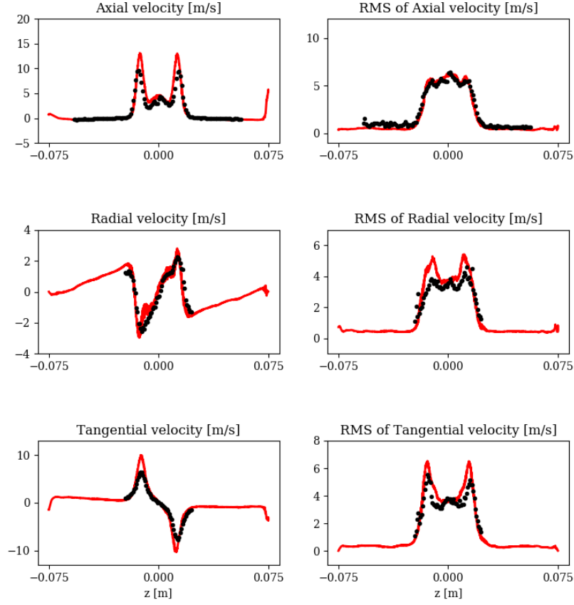
Figure 4.13: Profiles of mean (left) and RMS (right) velocity at x = 1 cm from the injector outlet: axial (top), radial (middle) and tangential (bottom) component. --: Numerical results; \bullet : Experimental data.
