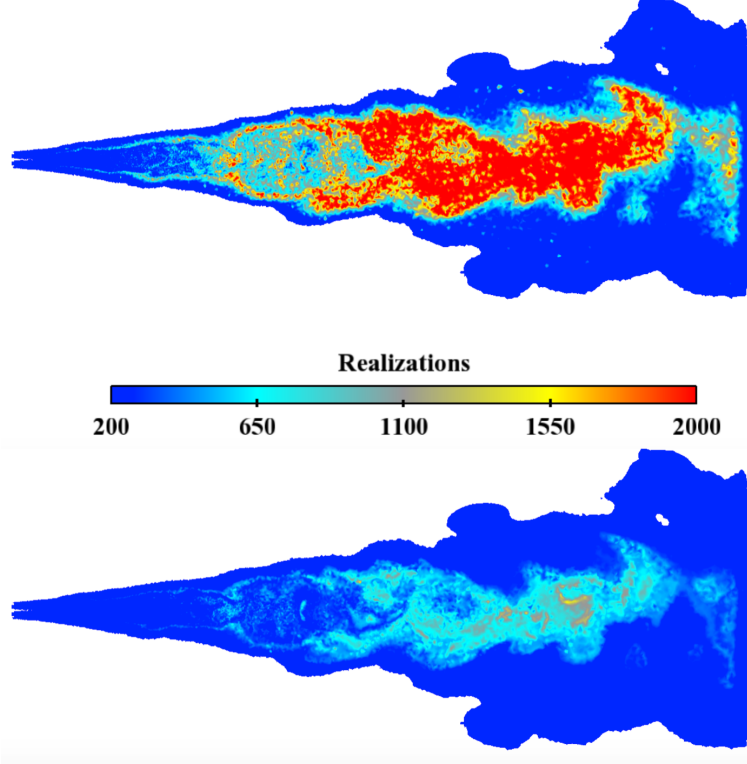
Figure 3.24: Field of the required number of rays in controlled-convergence Test 2 with MC (top) and RQMC (bottom) in a sooted jet flame application (Case 2).
