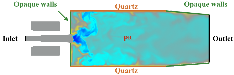
Figure 6.21: Control volume retained for the radiative transfer balance
