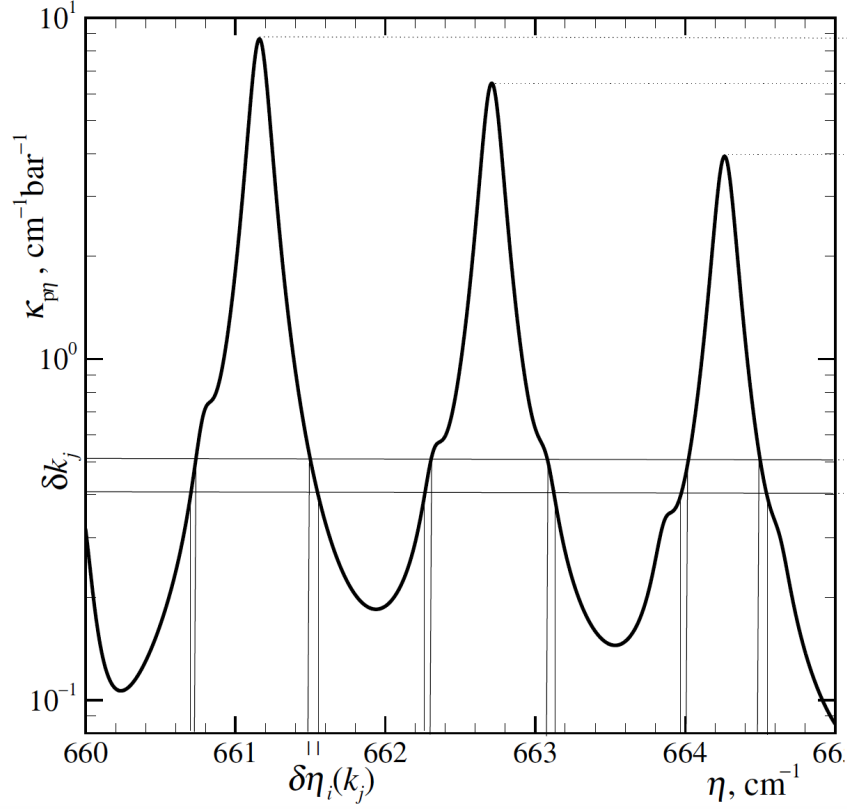
Figure 1.1: Absorption coefficient across a small portion of the \text{CO}_2 band as a function of the wavenumber \eta ( p = 1.0 bar, T = 296 K). Extracted from Modest (2013) .
