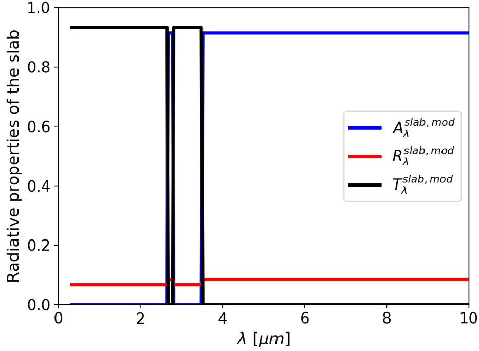
Figure 5.8: Modeled slab absorptance ( A_{\lambda}^{slab} ), transmittance ( T_{\lambda}^{slab} ) and reflectance ( R_{\lambda}^{slab} ) as a function of the wavelength for a 8 mm thickened fused silica VI 942.
