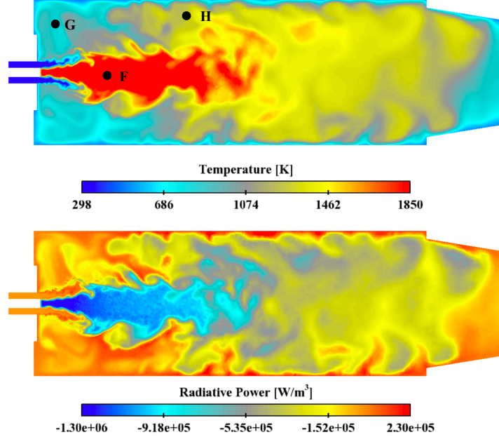
Figure 3.16: Instantaneous fields of temperature (top) and radiative power (bottom) on a longitudinal section of the burner. Points F, G and H, whose results are analyzed in Sec. 3.4, are indicated by black circles on the top figure.
