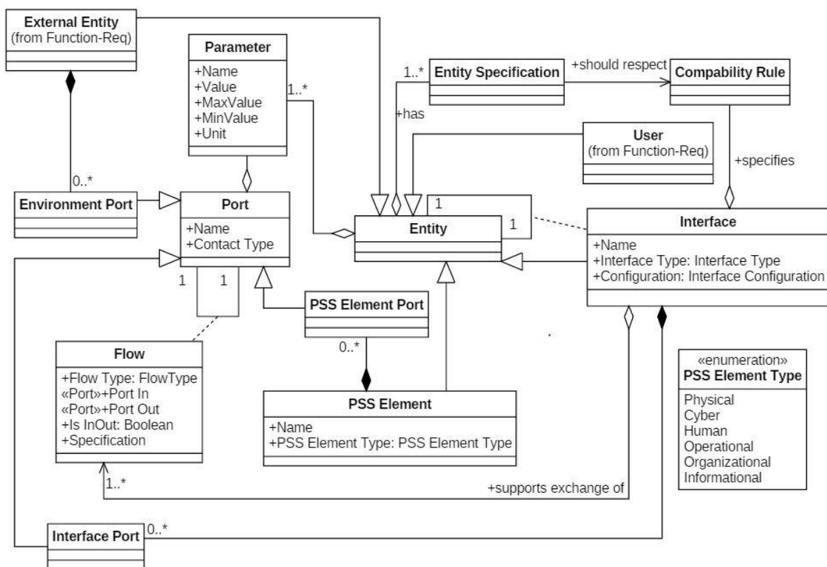
Figure 50. Interface model
