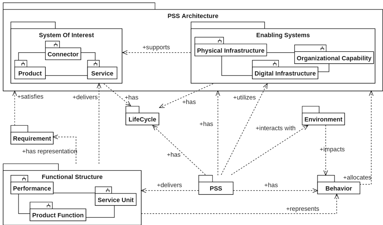
Figure 36. Package diagram
